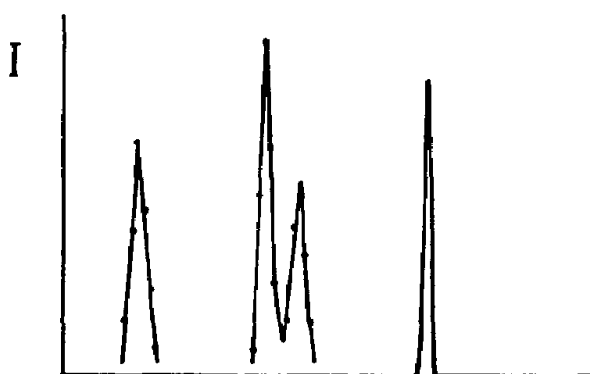
WAVELENGTH CHARACTERISTIC OF HYBRID LIGHT SOURCE INCLUDING MEDIUM-PRESSURE MERCURY (3MPa) AND RED LASER
