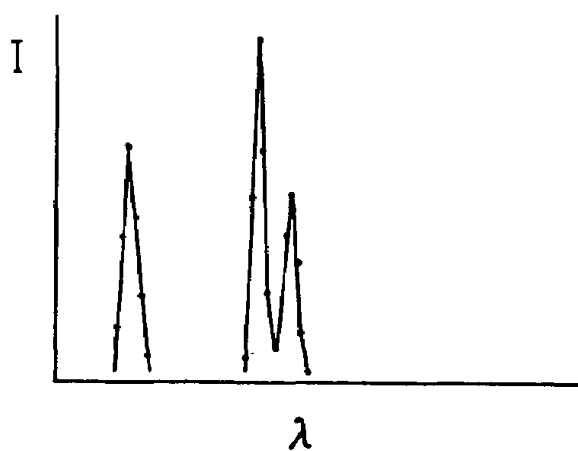
EMISSION WAVELENGTH CHARACTERISTIC OF MEDIUM- PRESSURE MERCURY LAMP
