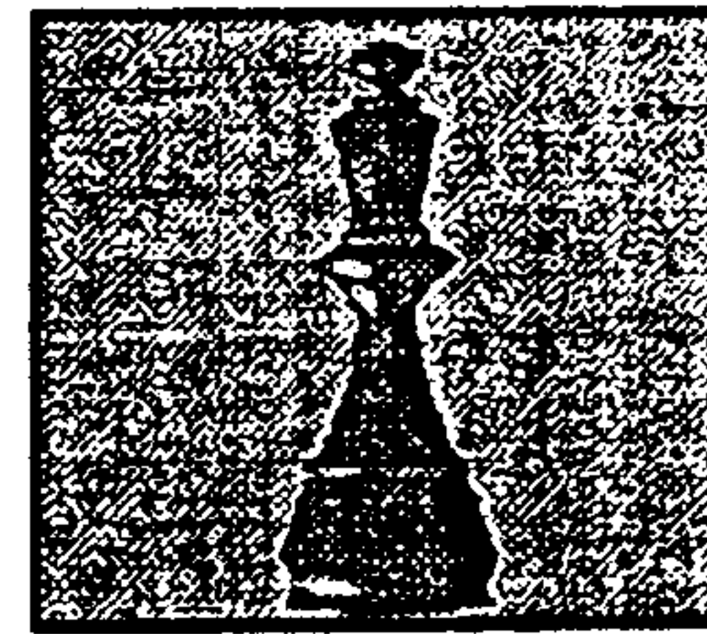
Fedor Shading
