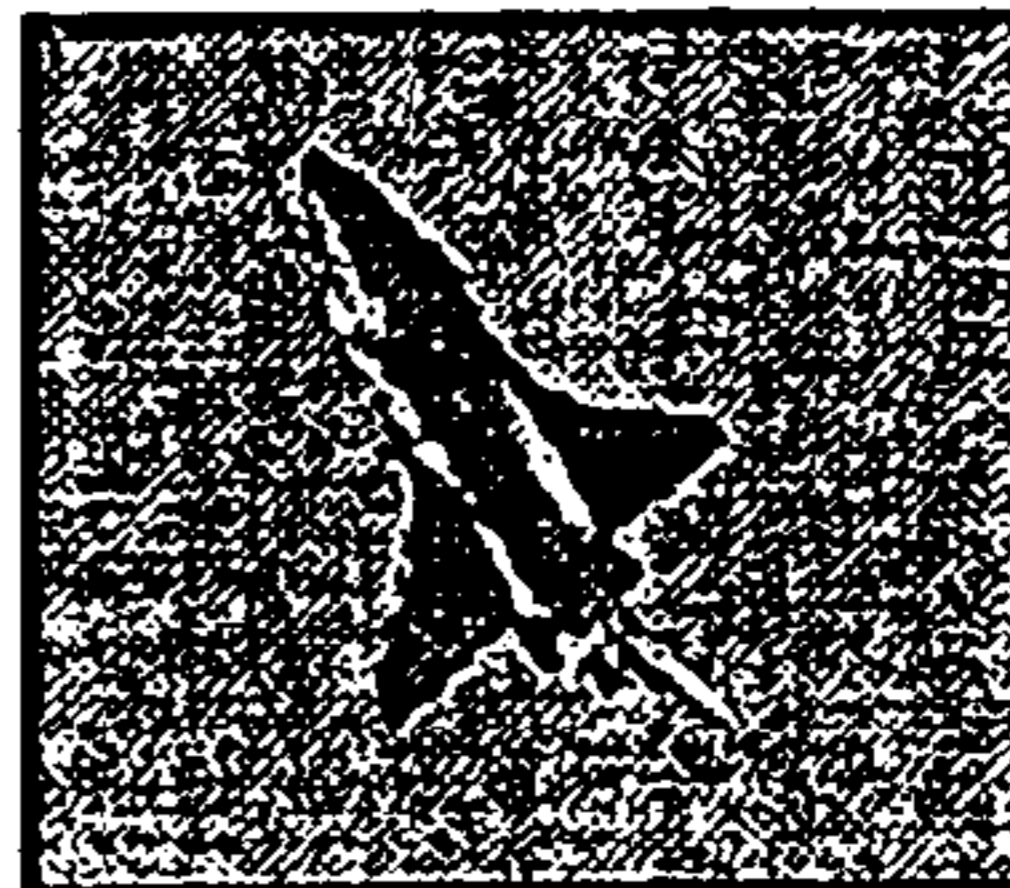
Fedor Shading
