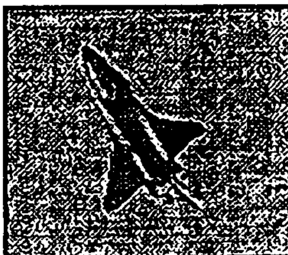
Phong Shading
