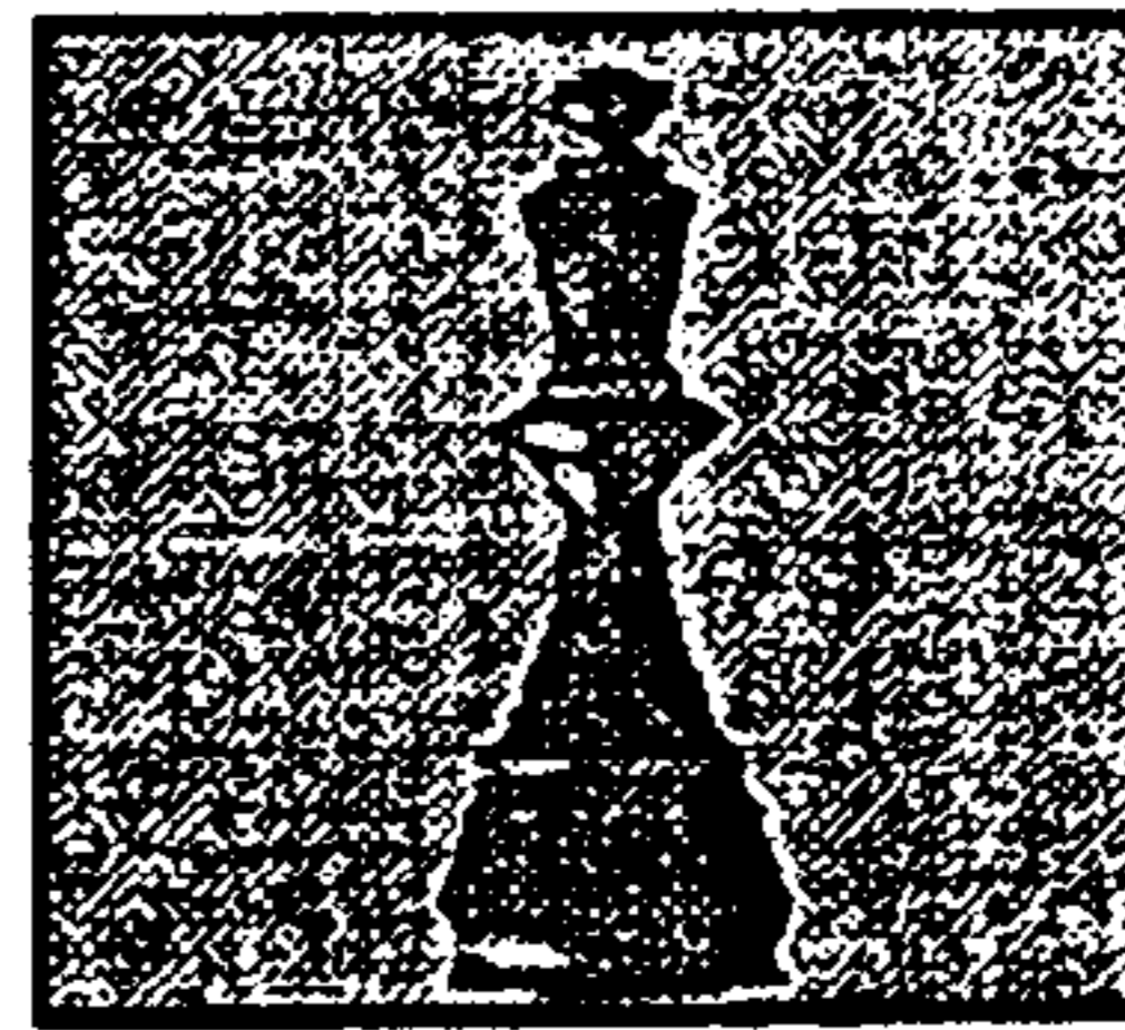
Fedor Shading
