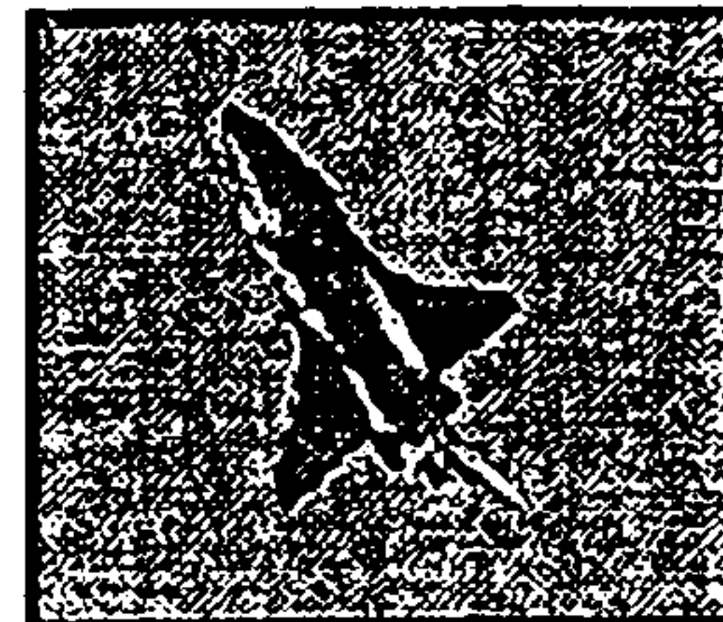
Fedor Shading
