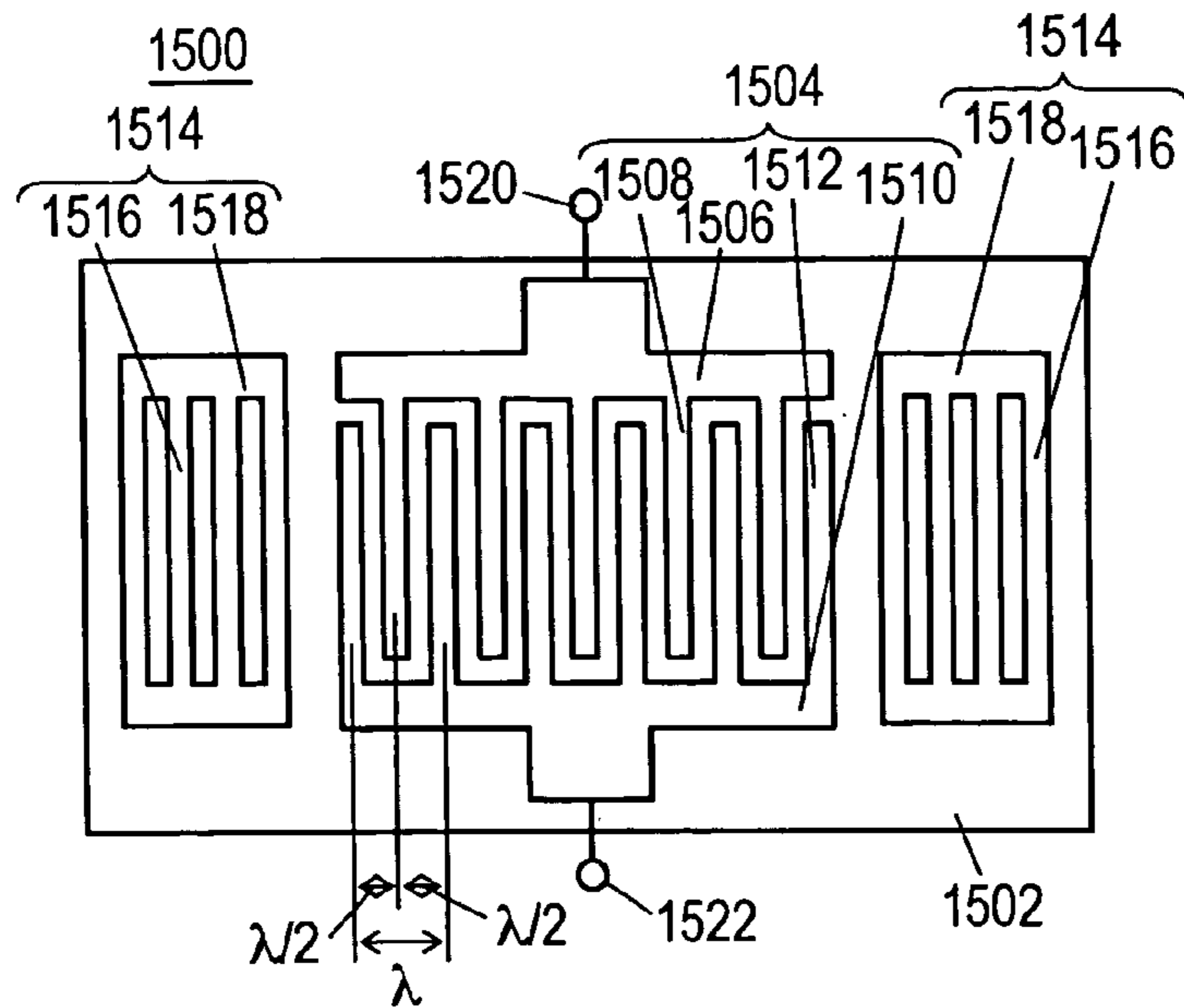
FIG. 15 PRIOR ART
