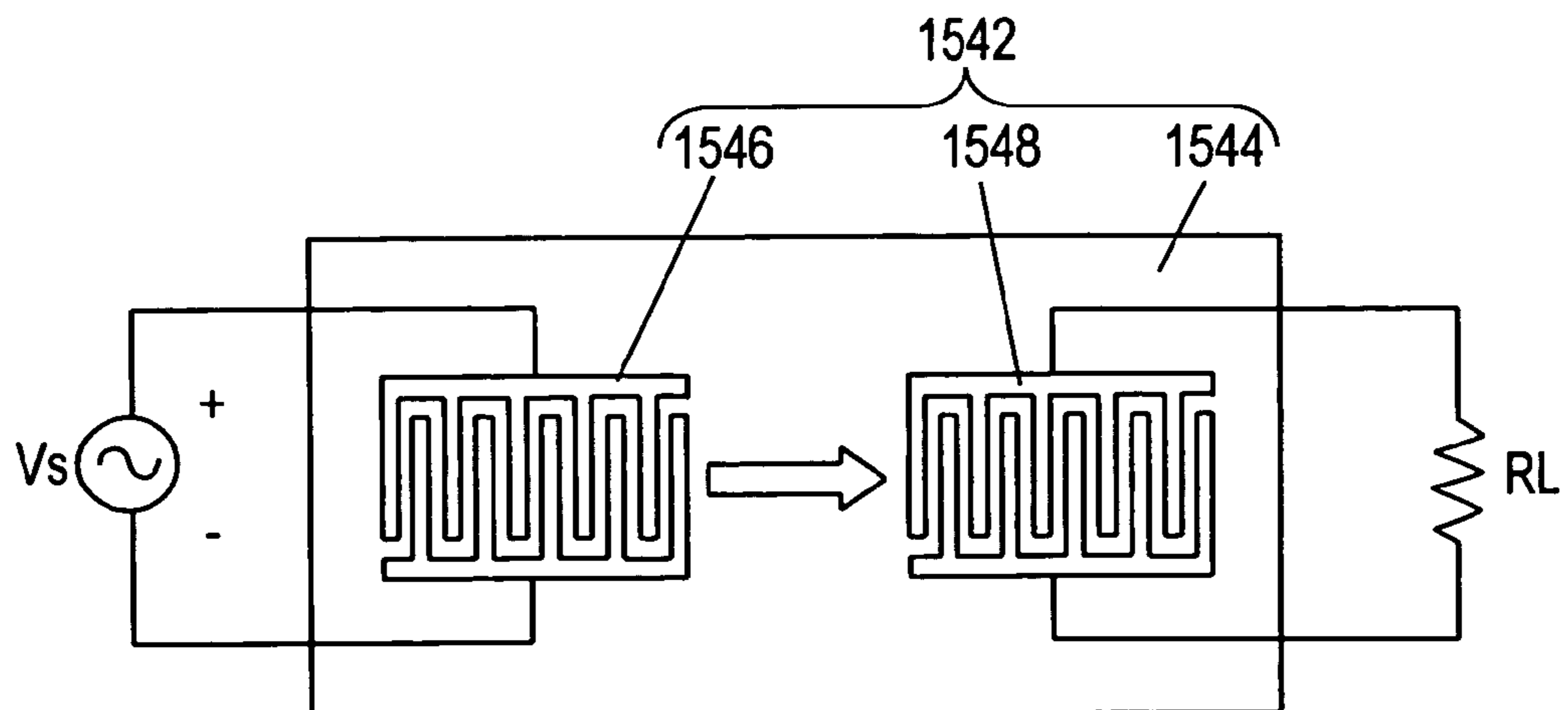
FIG. 18 PRIOR ART
