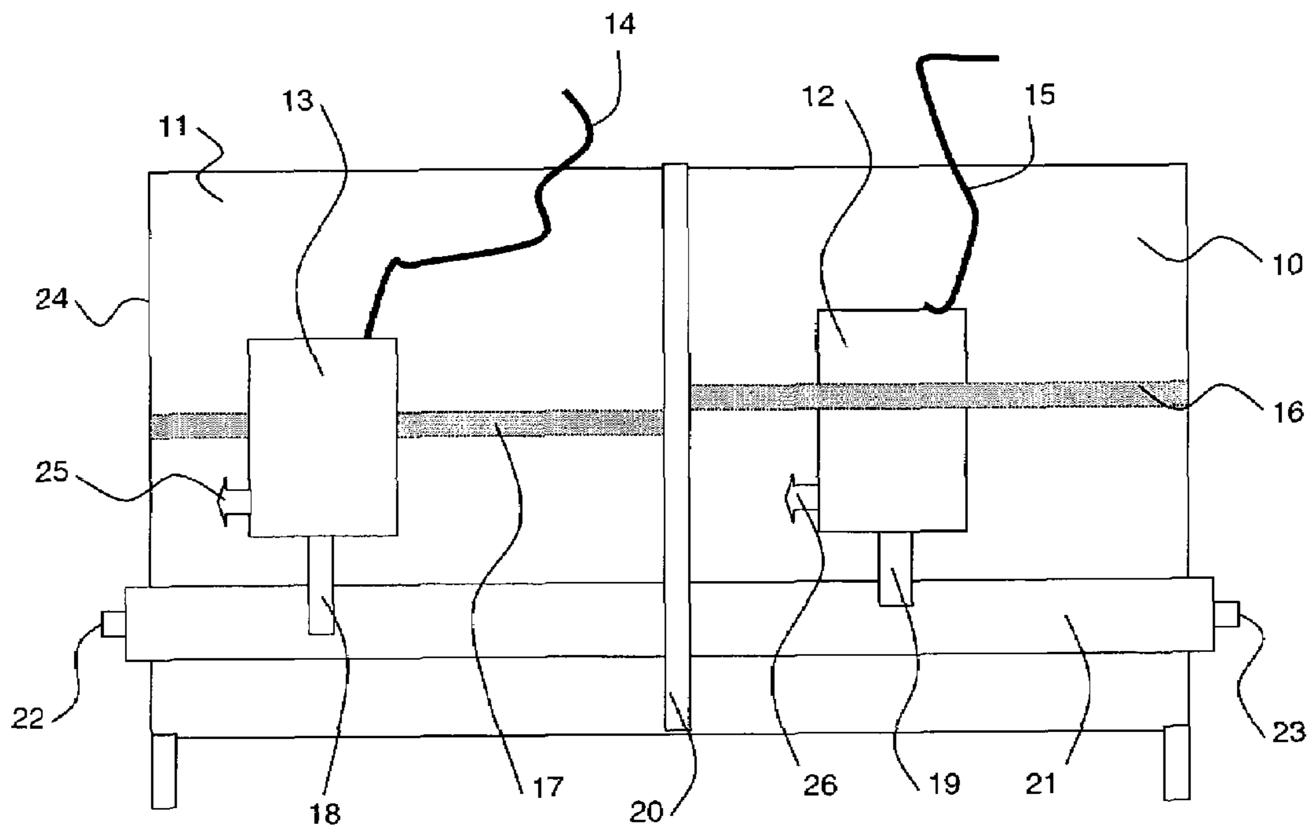
FIG. 2: Prior Art: Pre-matching tuner structure
