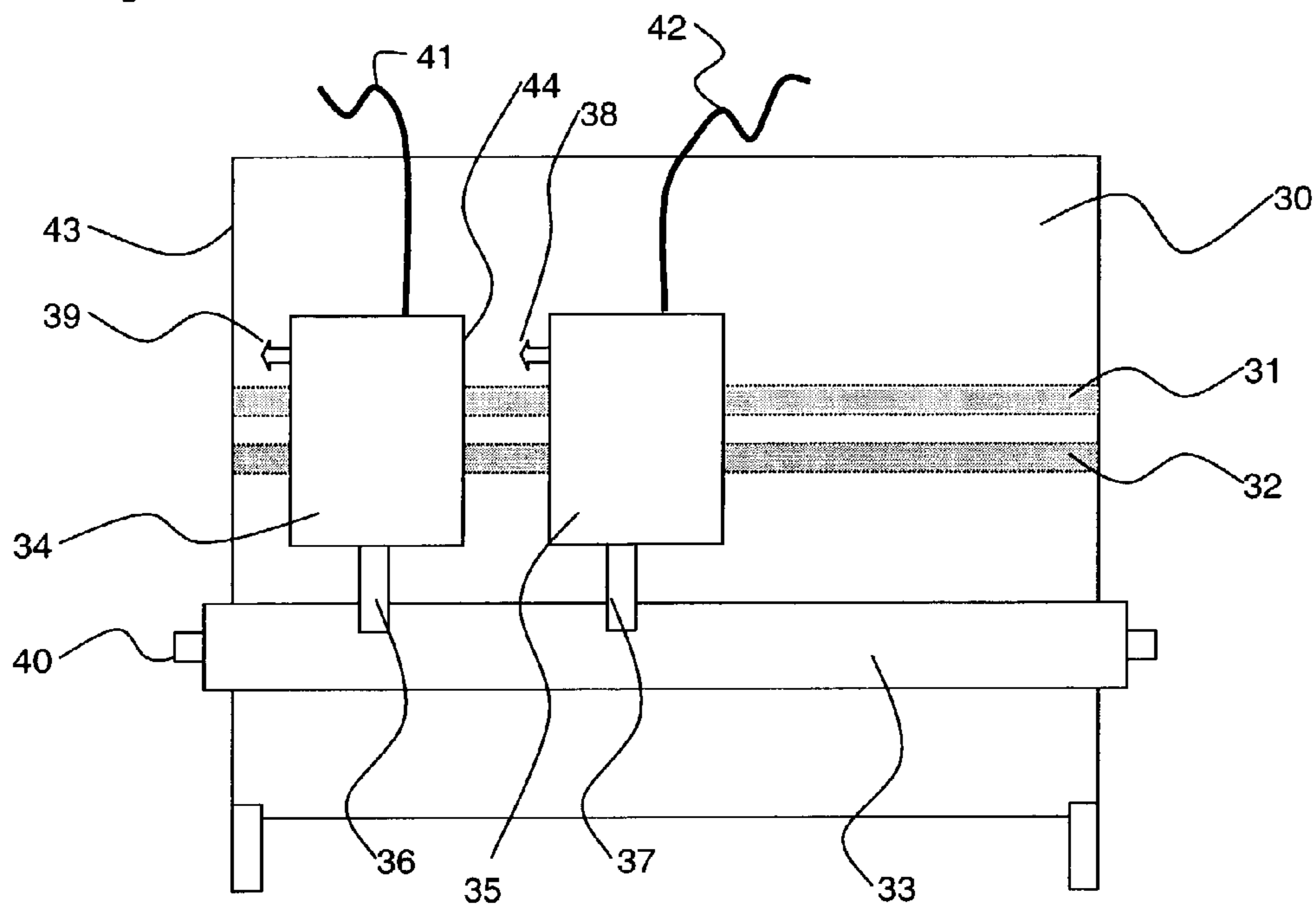
FIG. 3: Prior Art: Tuning mechanism of traditional pre-matching tuners with fixed pre-matching and tuning sections
