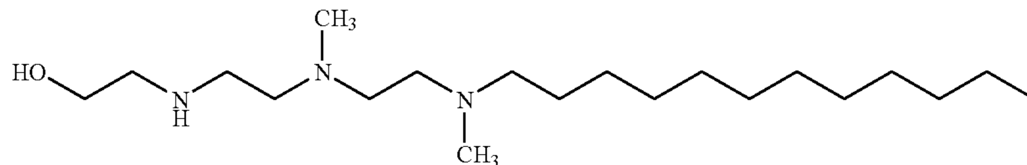
Triamine
