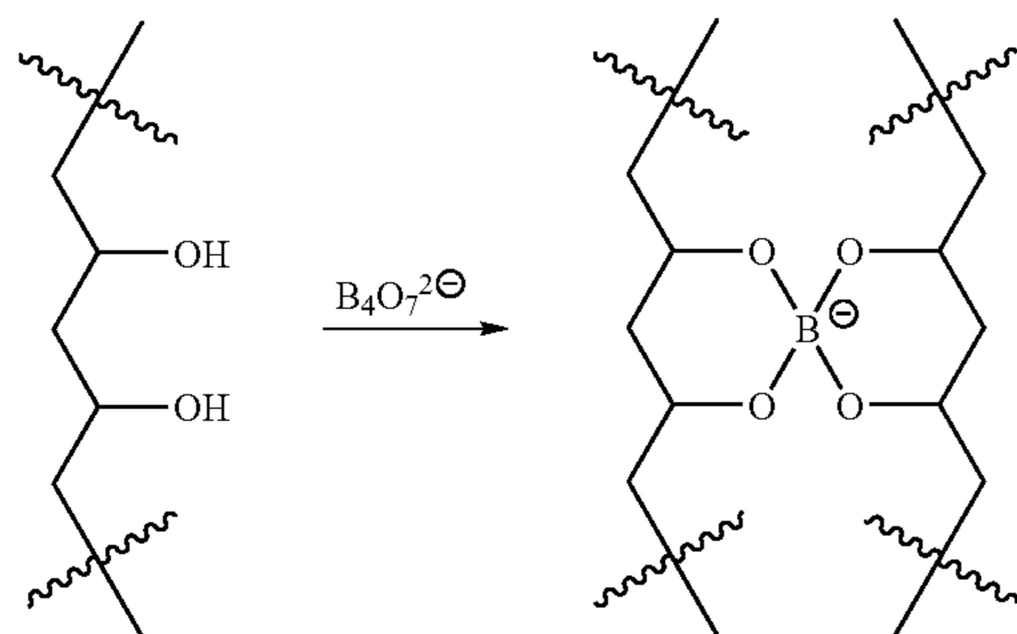
Borate-PVA complexation
