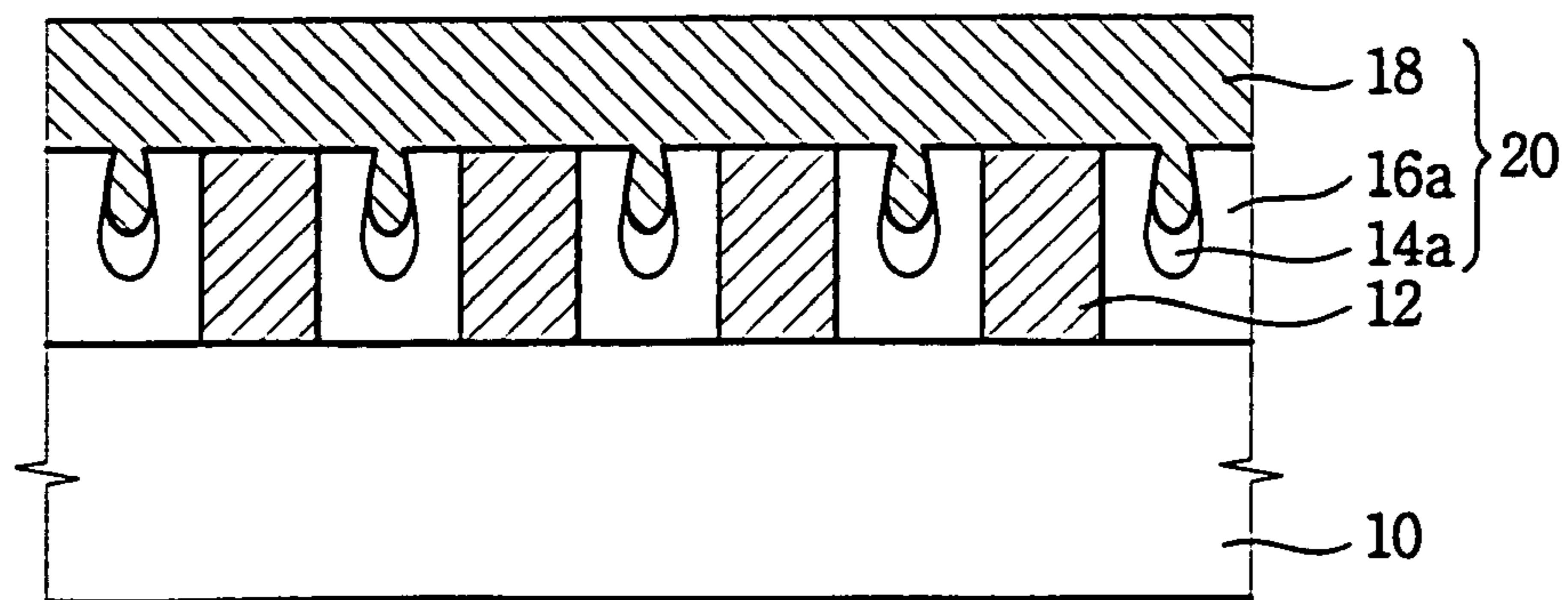
FIG. 1C (PRIOR ART)
