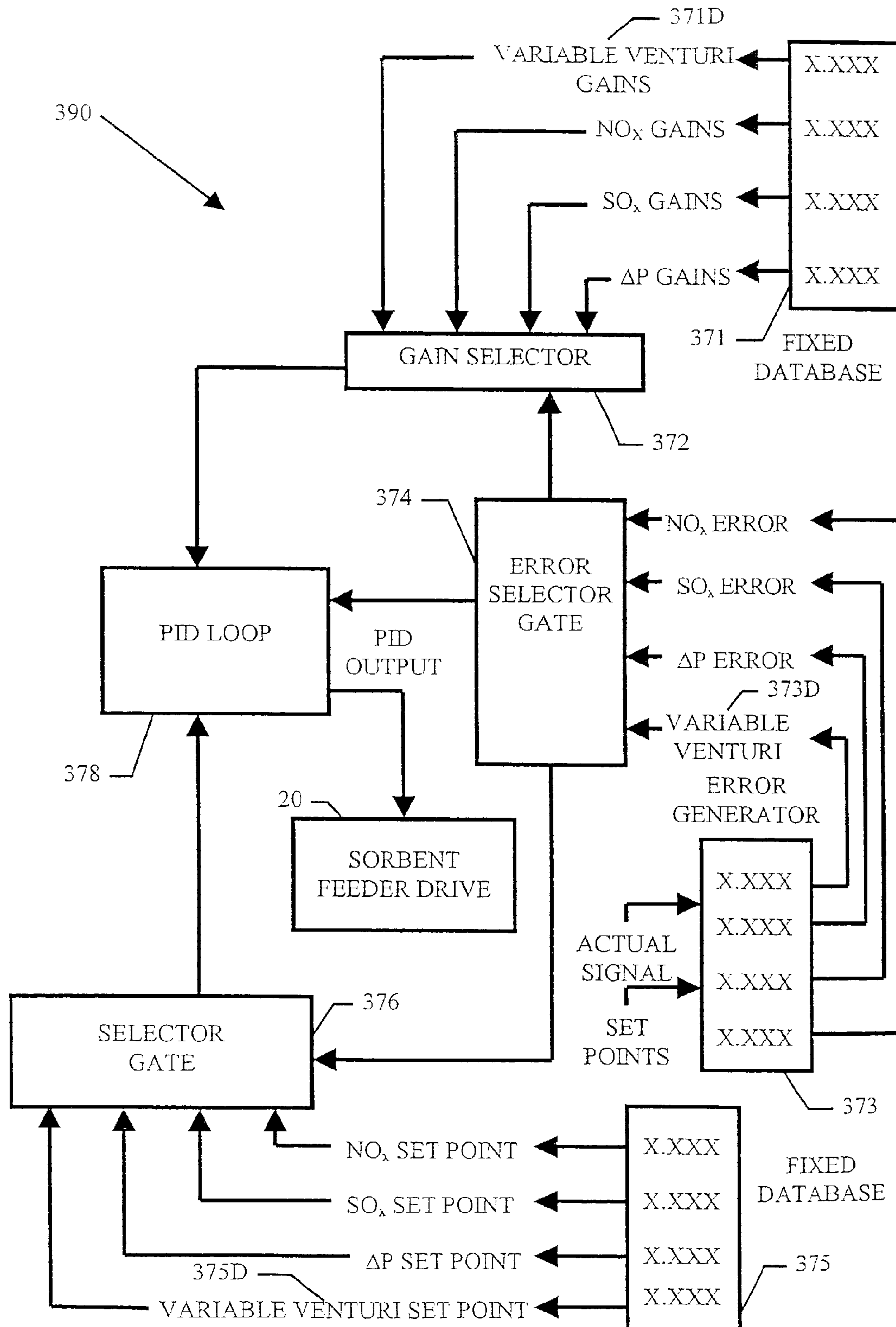
FIGURE 25 SOFTWARE CONTROL LOOP FOR SIMULTANEOUS \text{NO}_x , \text{SO}_x , \Delta\text{P} CONTROL, AND VARIABLE VENTURI POSITION CONTROL
