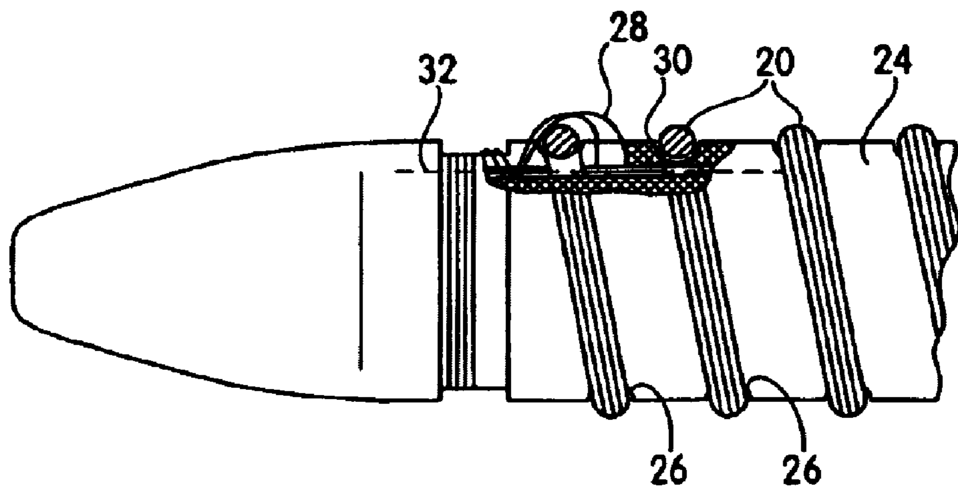
Fig. 5 (Prior Art)
