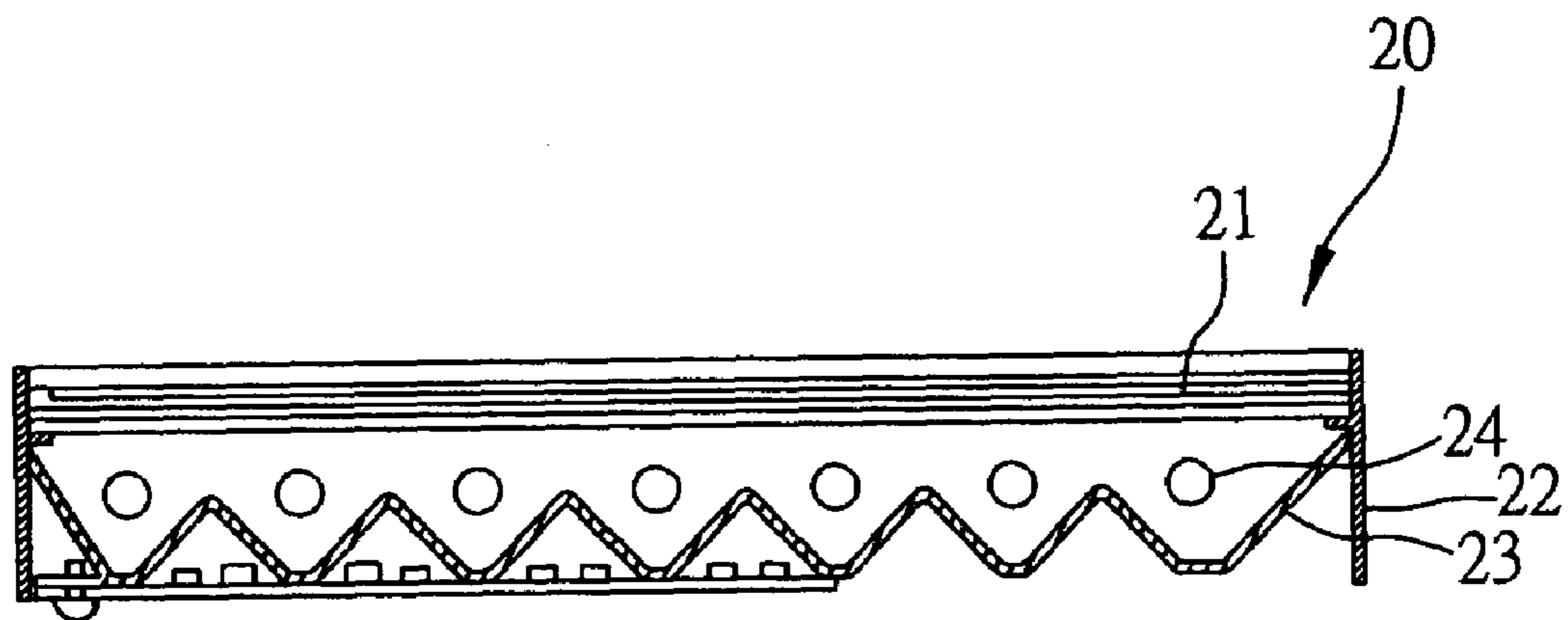
FIG. 2 (Prior Art)
