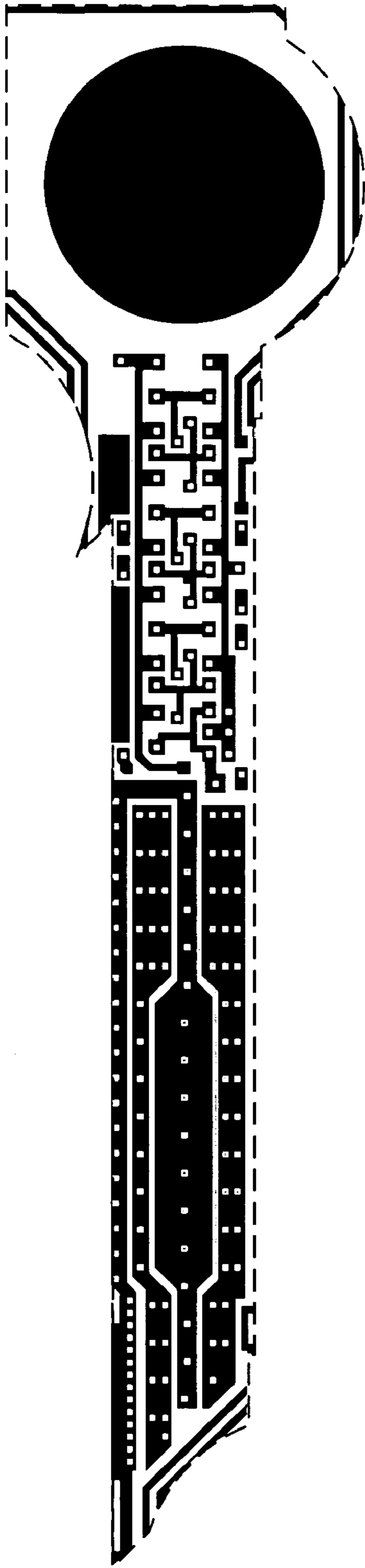
Metal 1 mask
