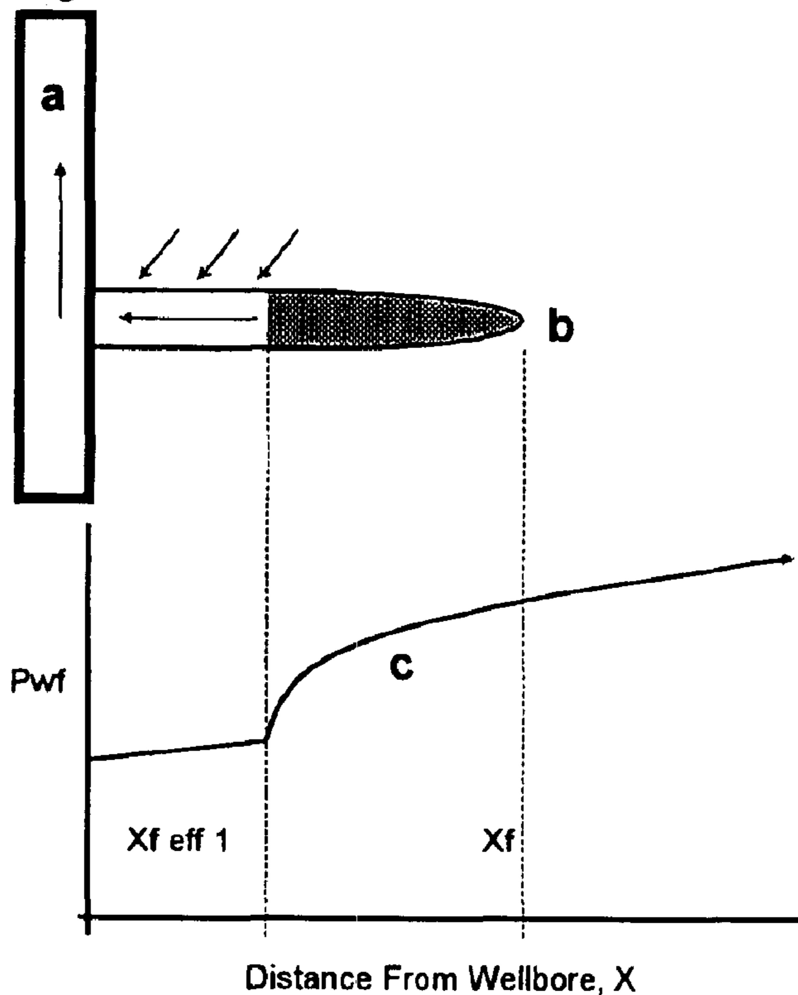
Figure 1A: Fracture-Stimulated Gas Well Before Process
