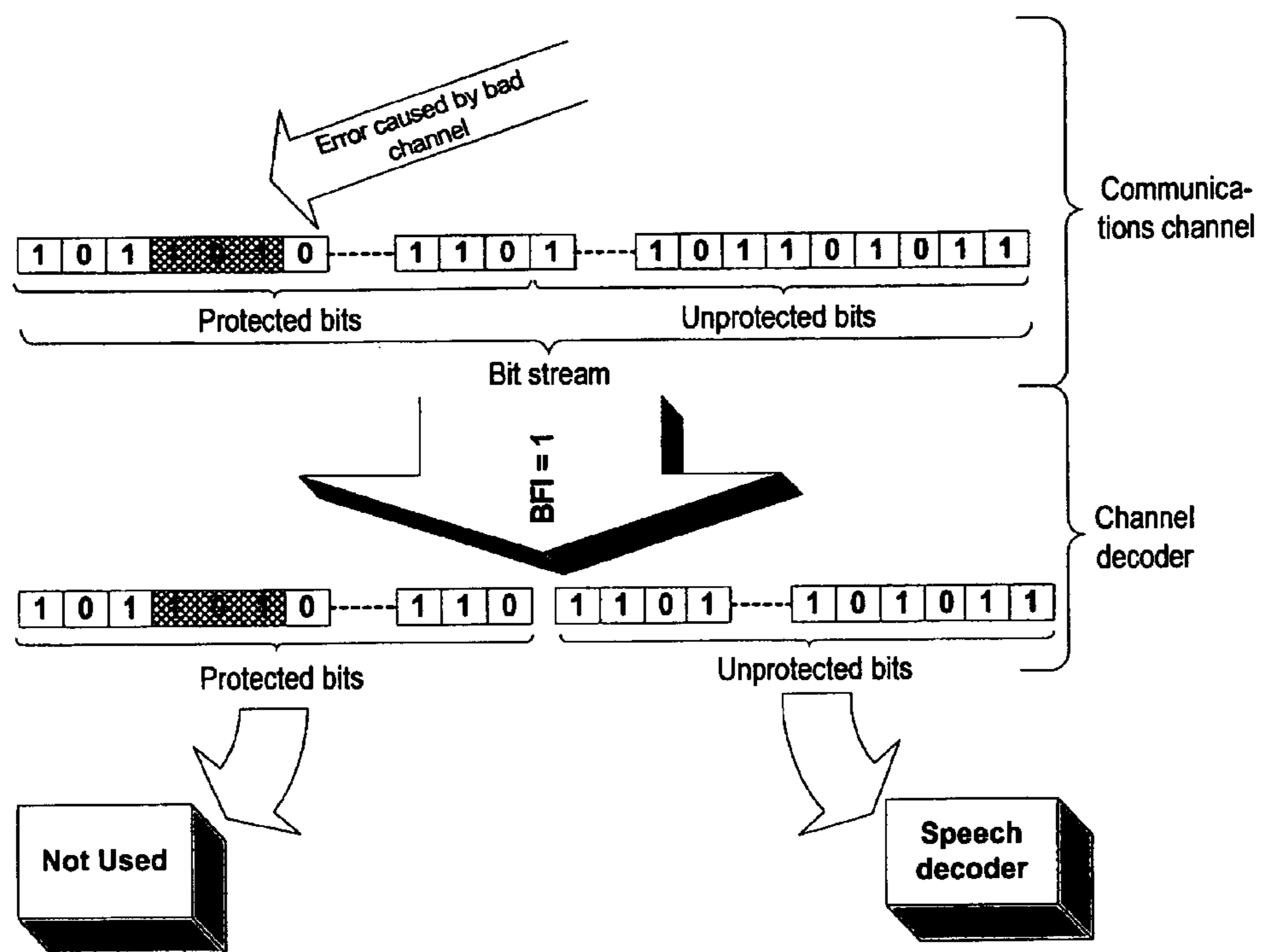
Fig. 6 (Prior art)
