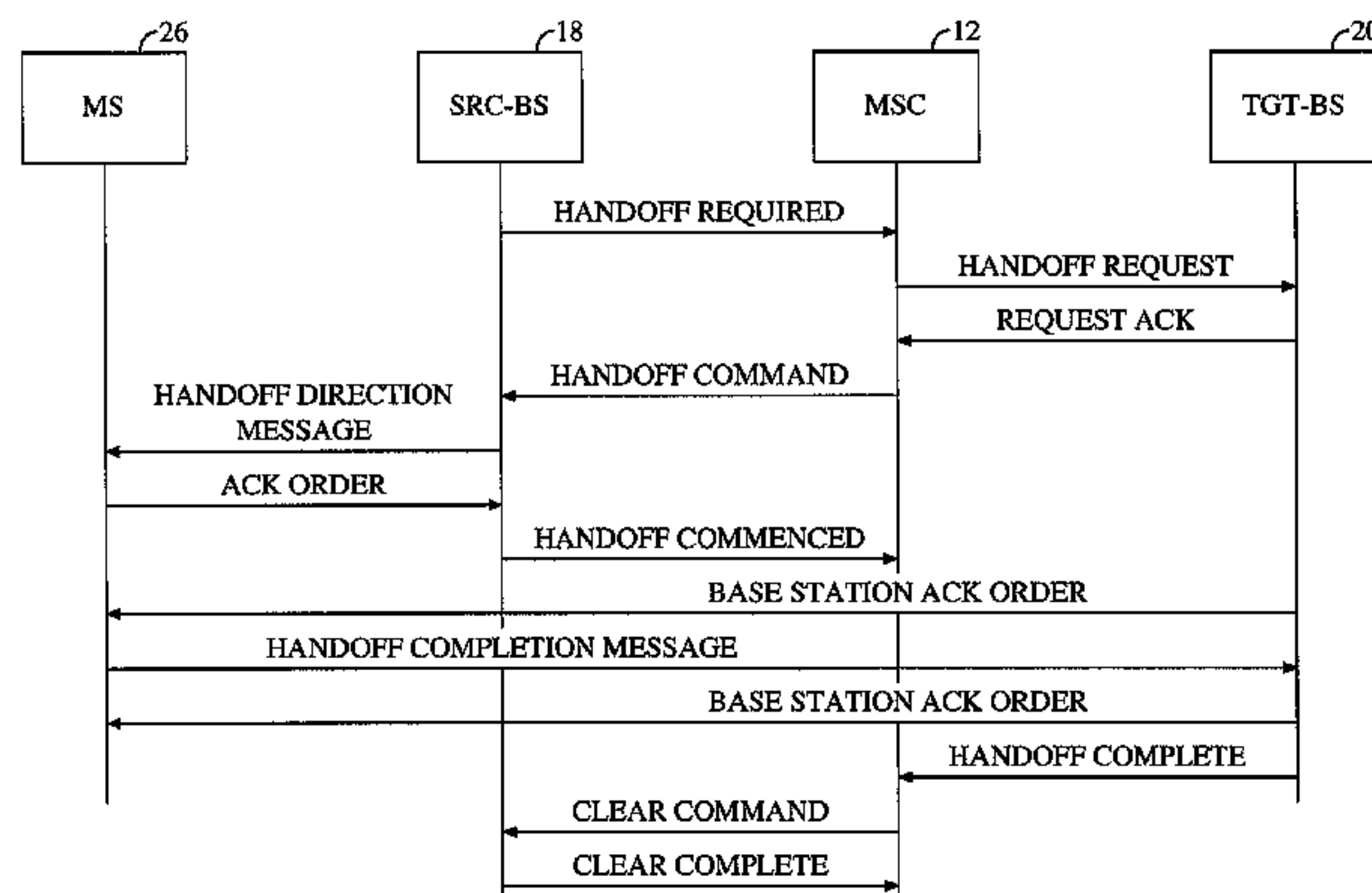
SUCCESSFUL IS-95 TO IS-95 HARD HANDOFF
