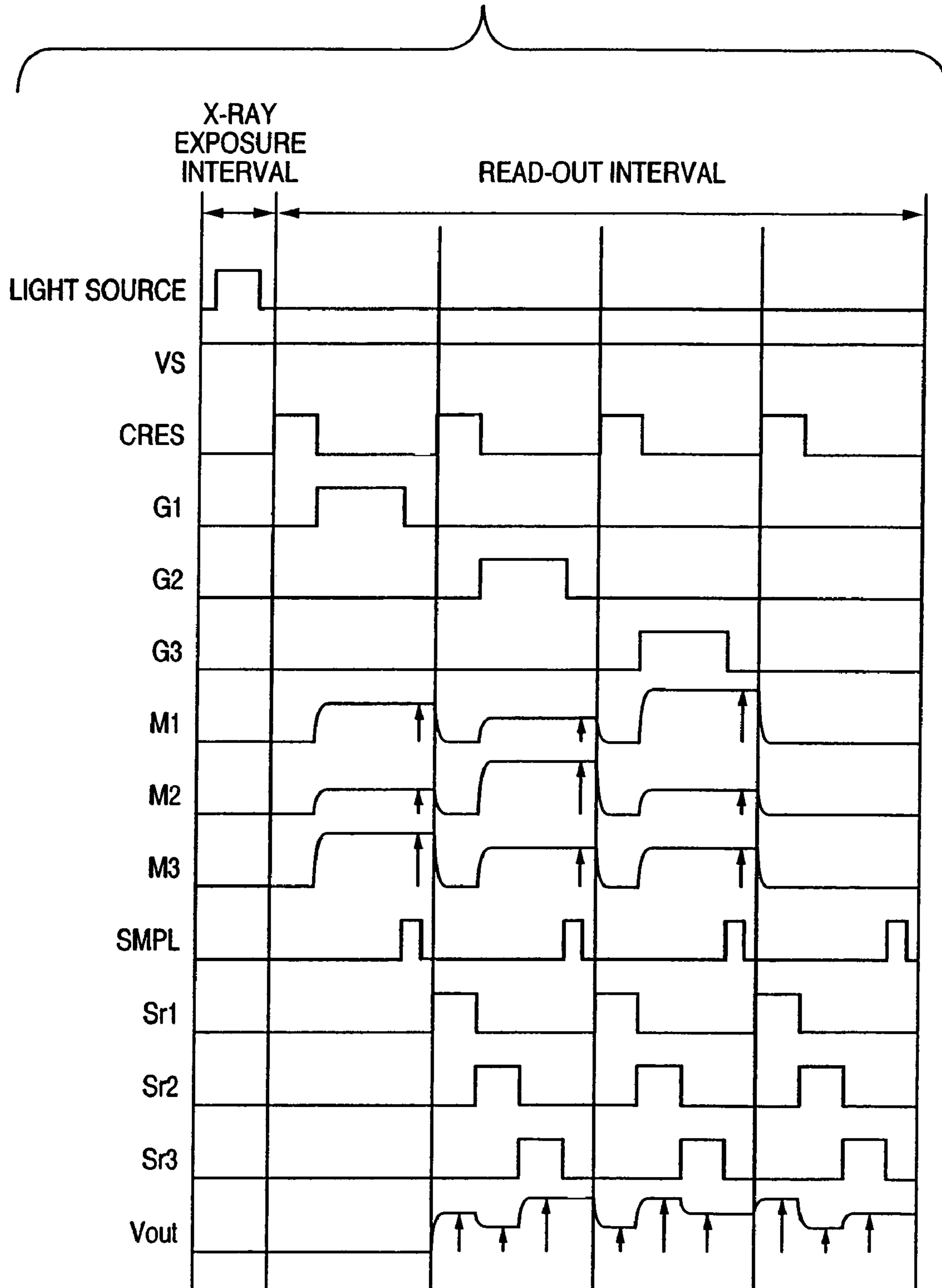
FIG. 7 (PRIOR ART)
