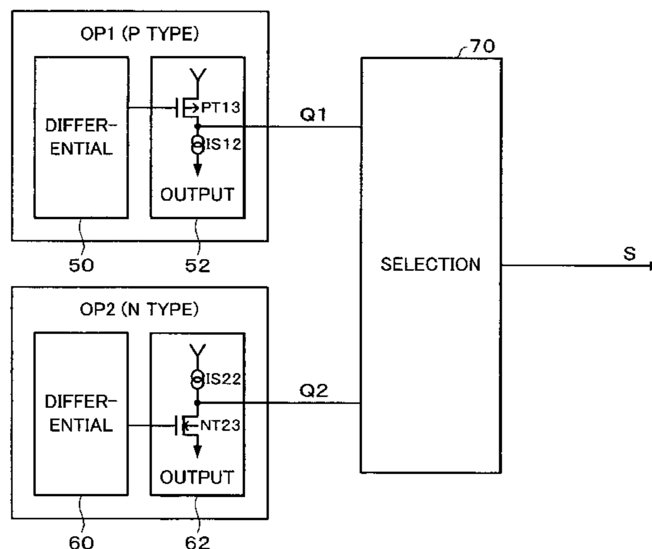
OPERATIONAL AMPLIFIER CIRCUIT
