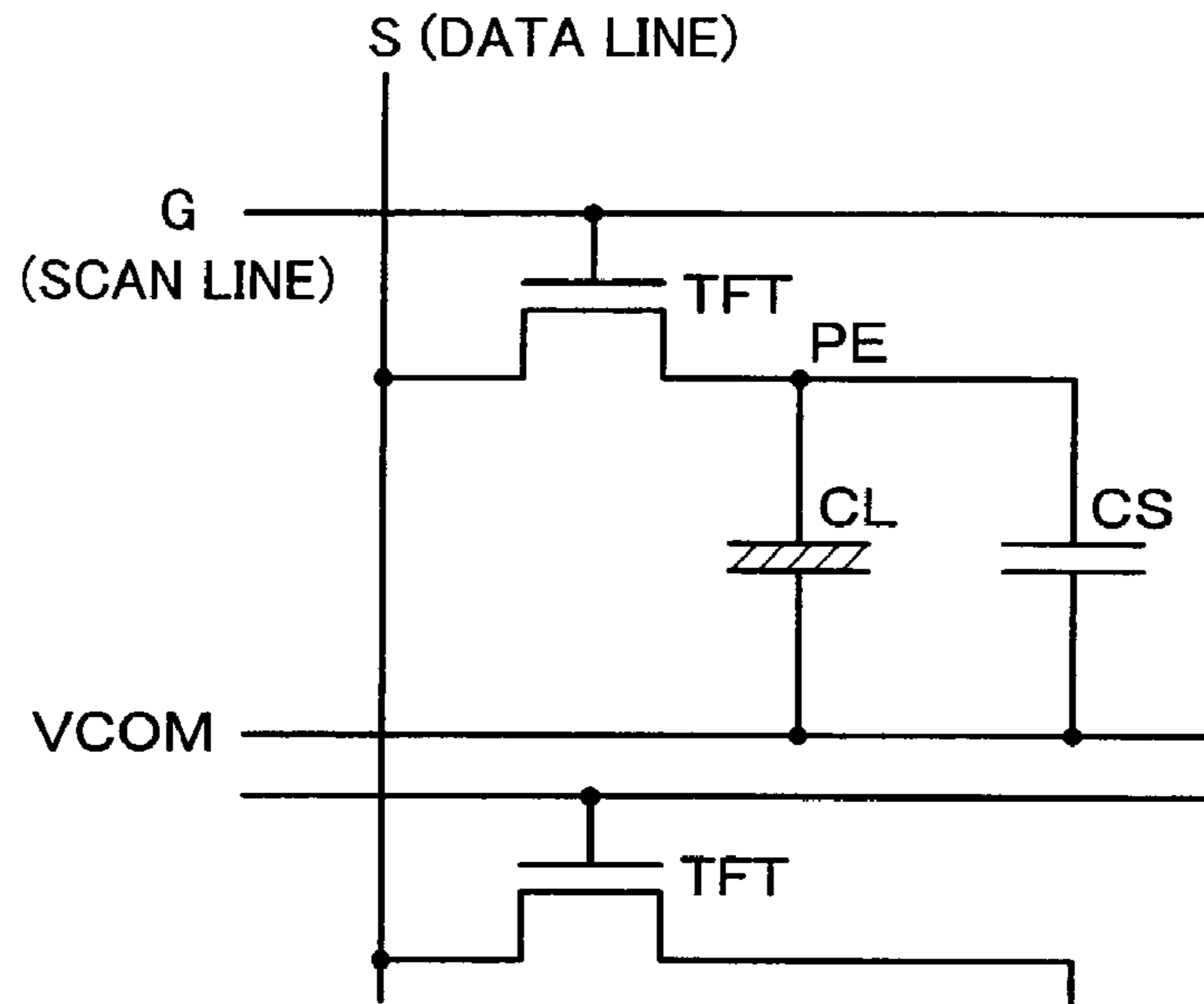
FIG. 12A STORAGE CAPACITANCE METHOD
