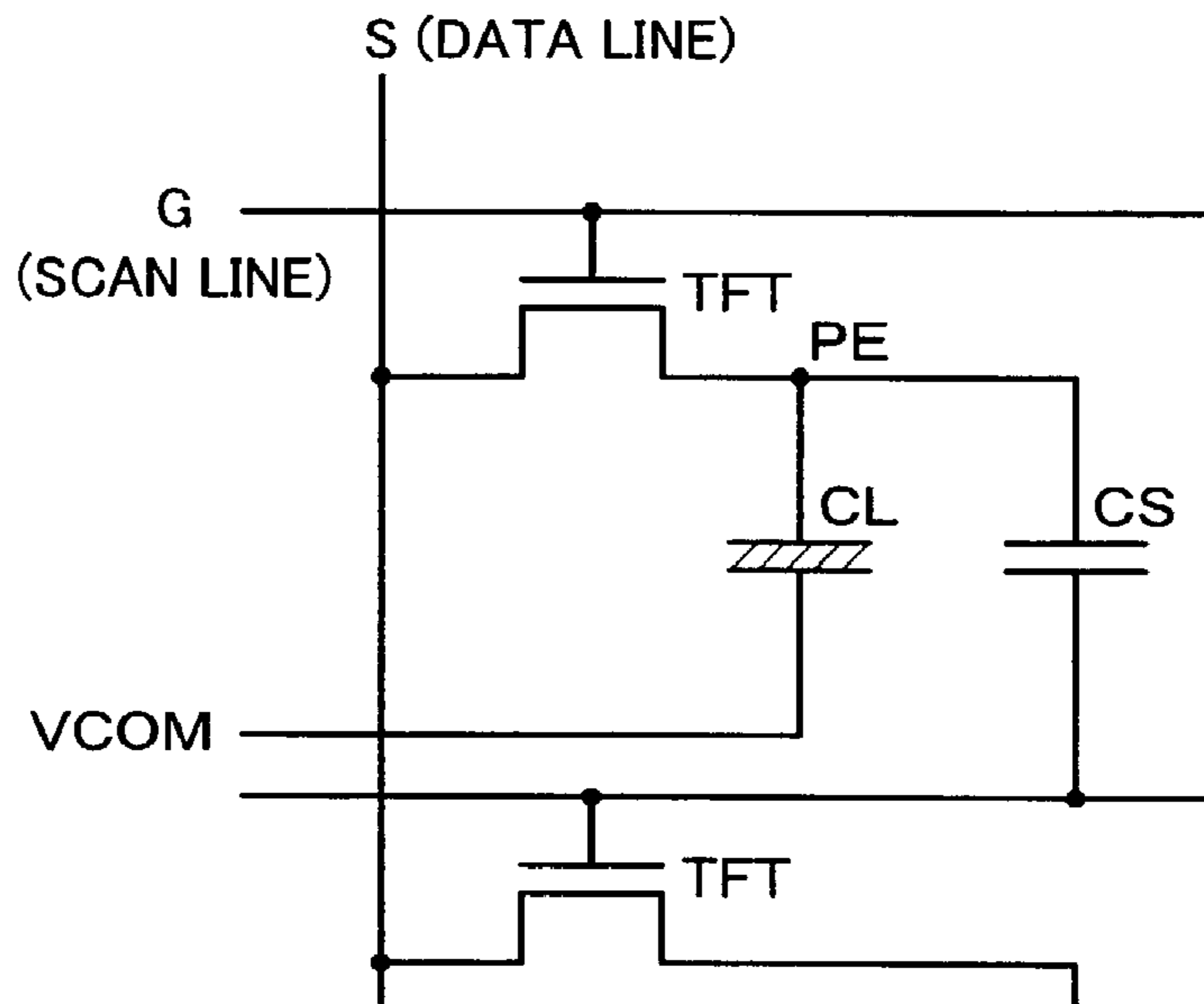
FIG. 12B ADDITIONAL CAPACITANCE METHOD
