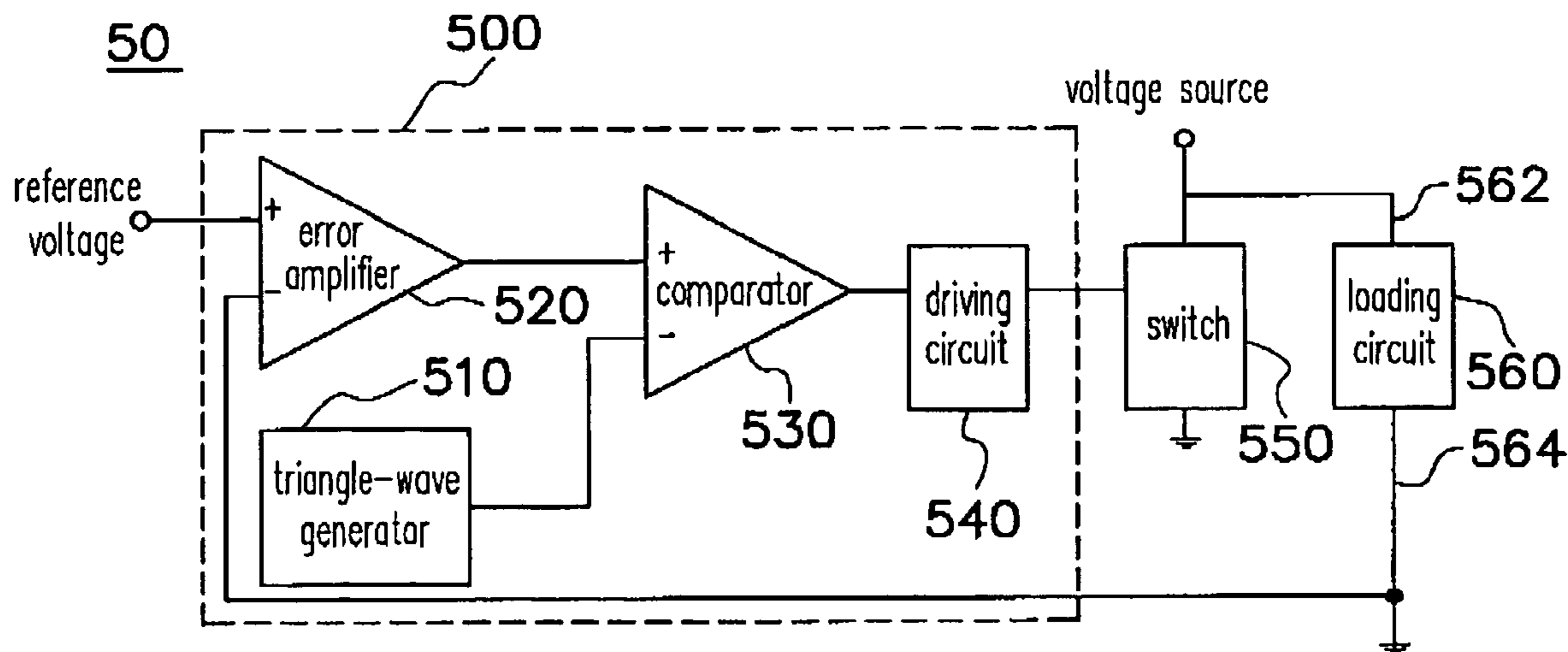
FIG. 5 (PRIOR ART)
