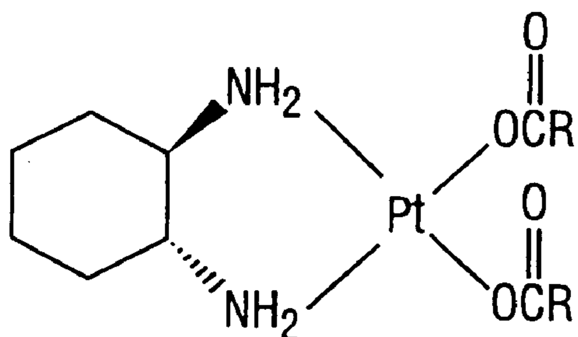
DACH Platinum(II) Complex
