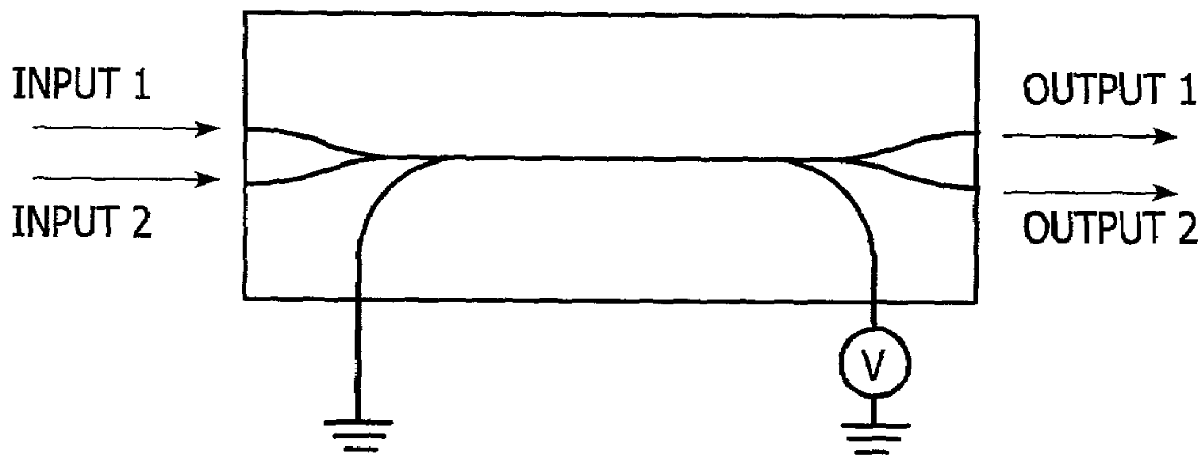
DIRECTIONAL COUPLER
