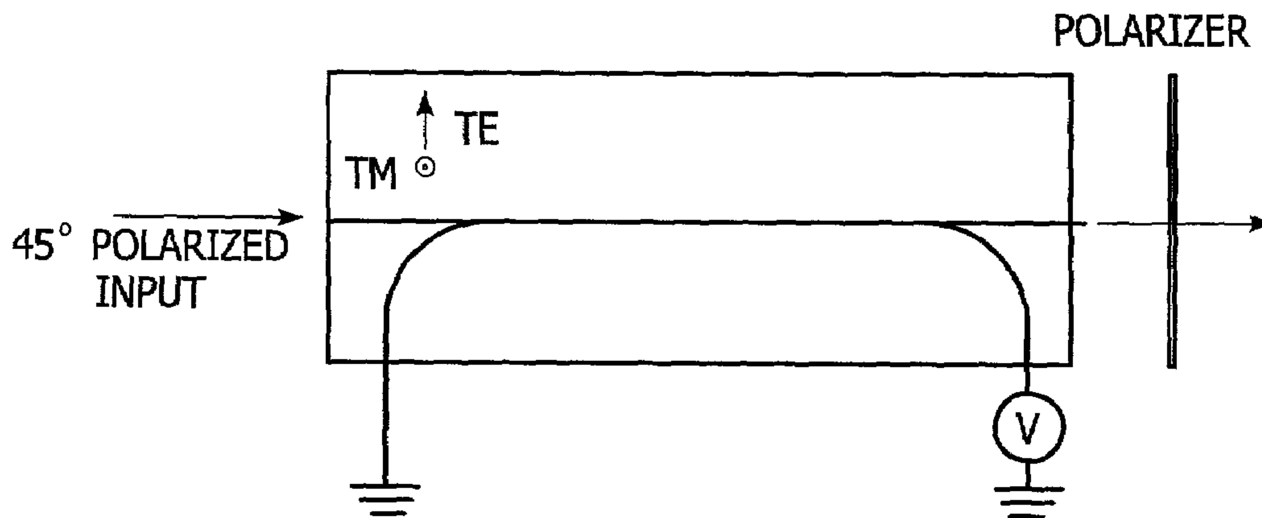
BIREFRINGENT MODULATOR
