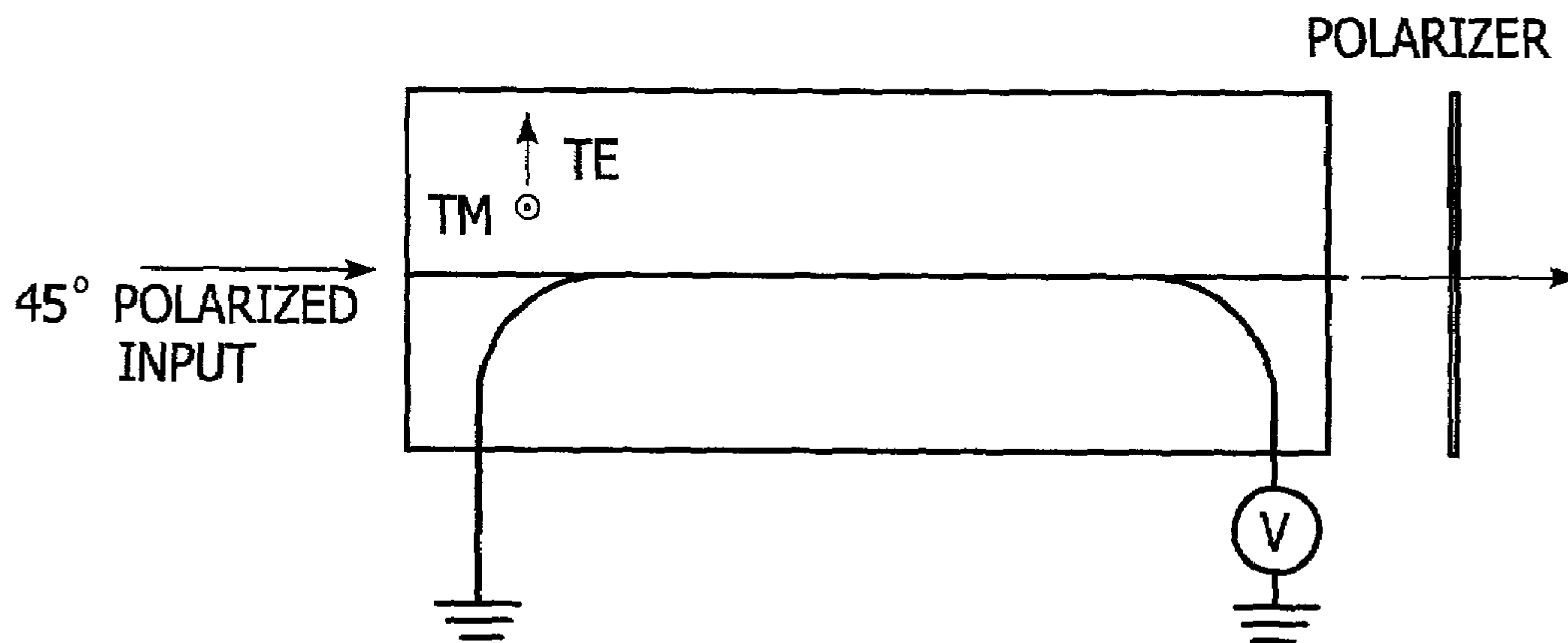
BIREFRINGENT MODULATOR
