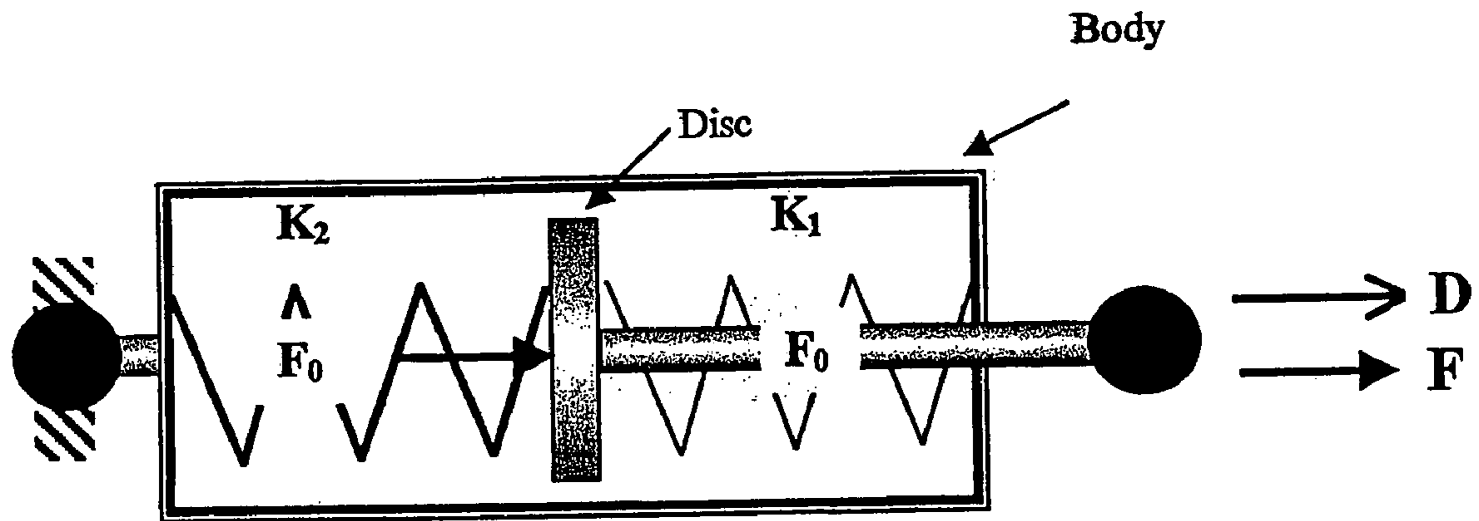
Free-body diagram
