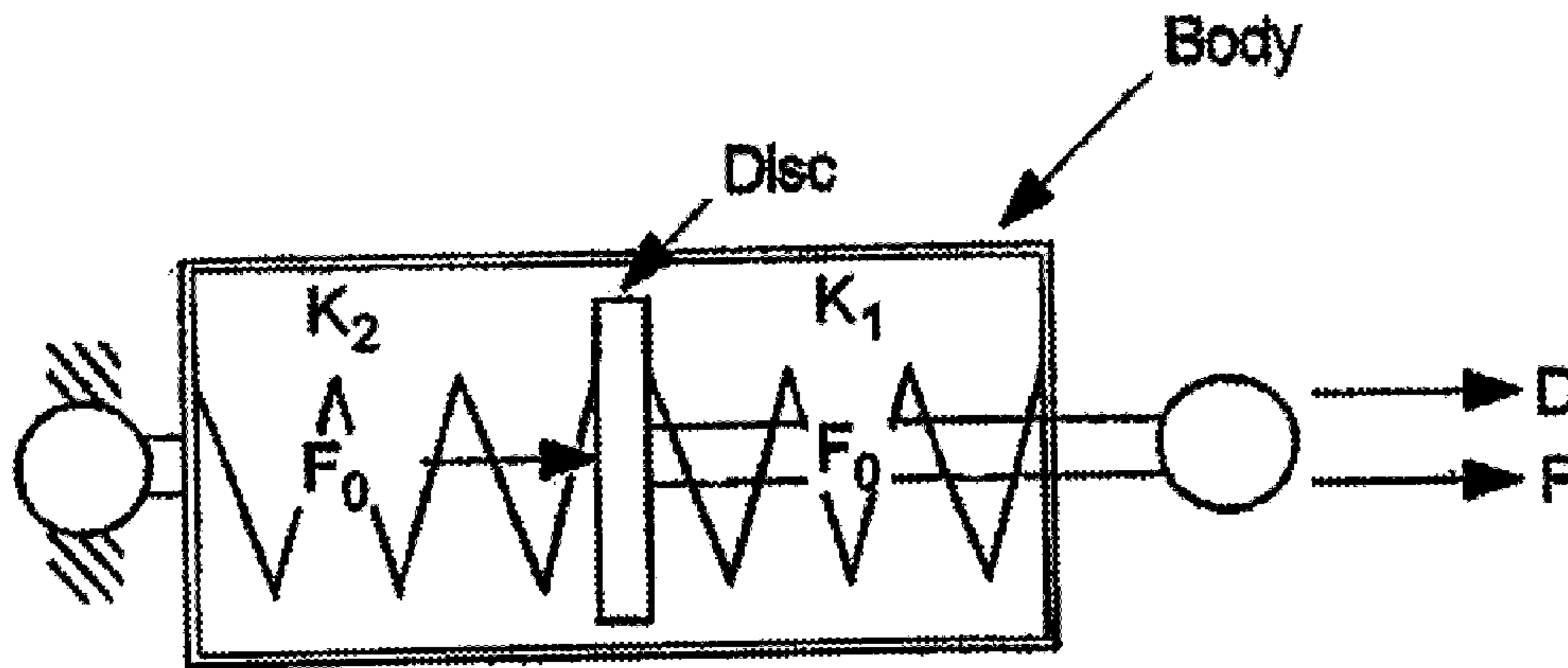
Free-body diagram
