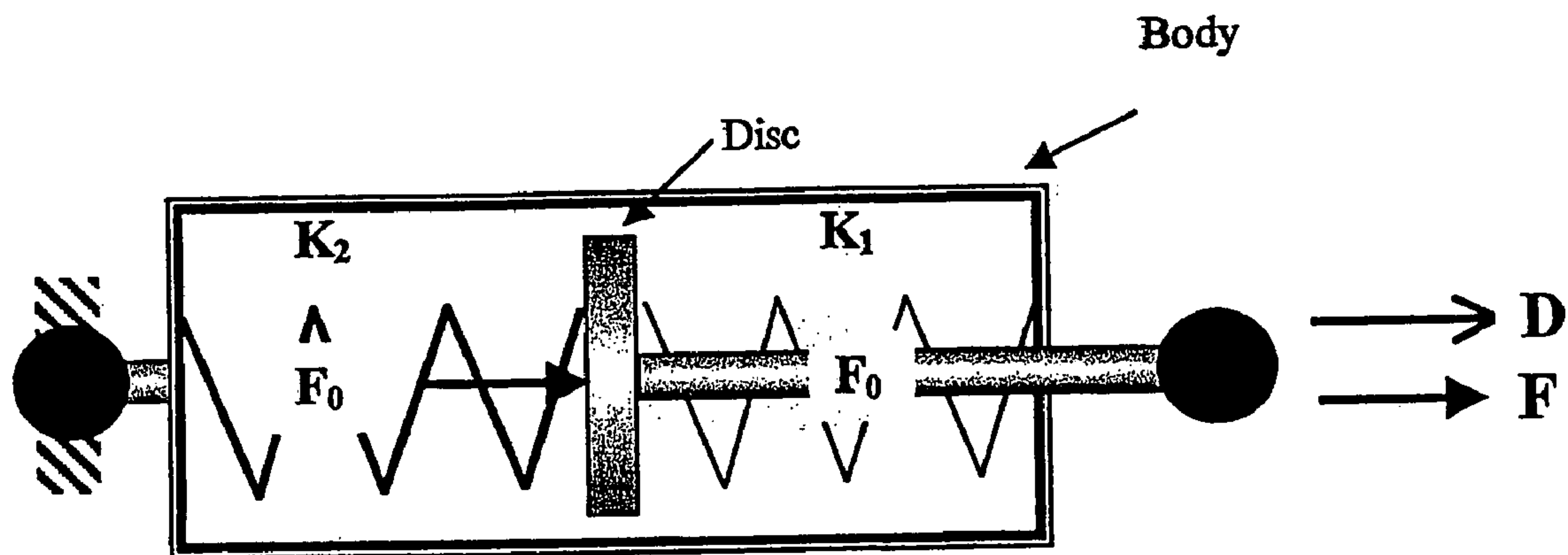
Free-body diagram
