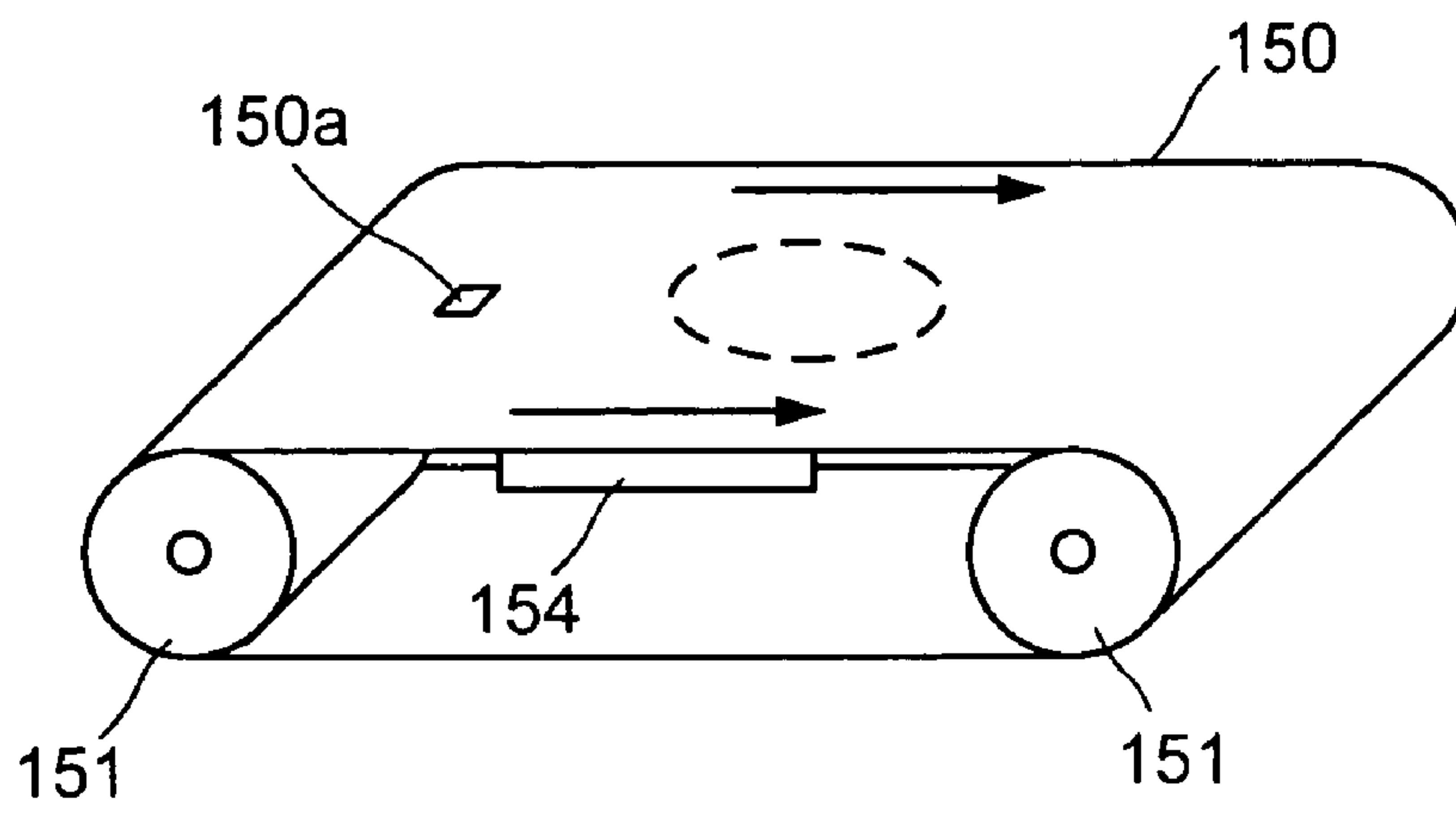
FIG. 1C (prior art)
