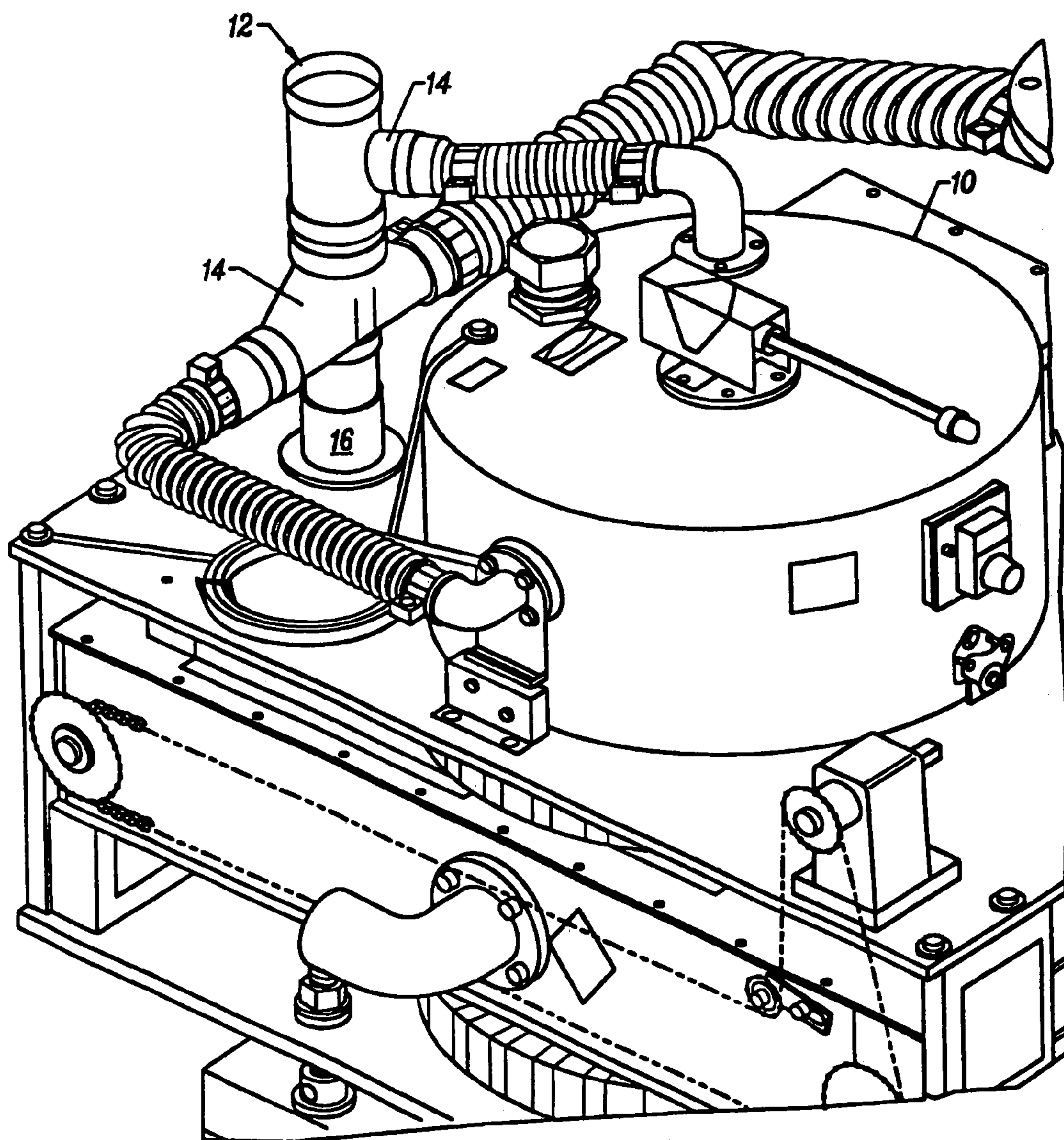
FIG. 1 (Prior Art)
