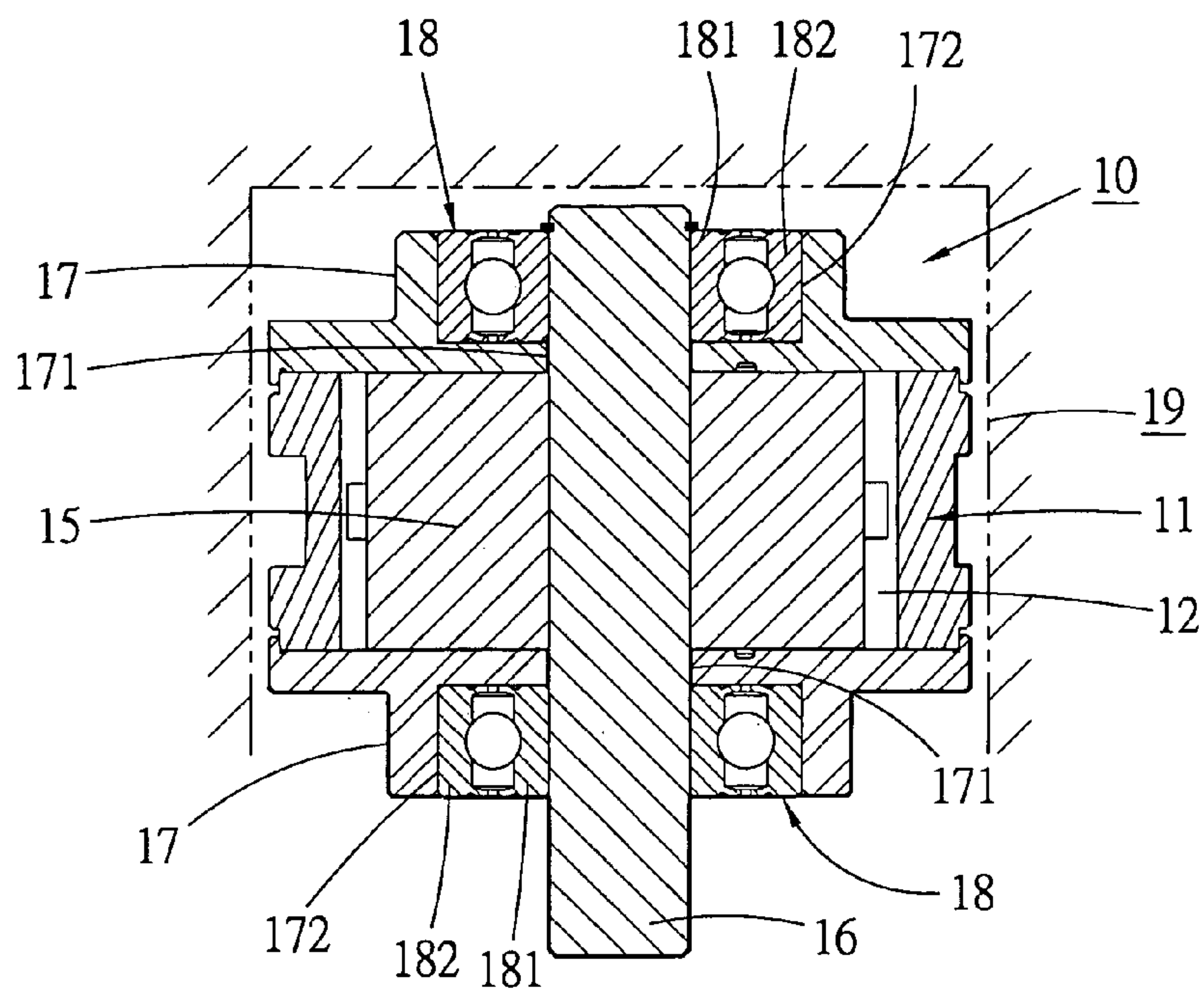
Fig. 1 Prior Art
