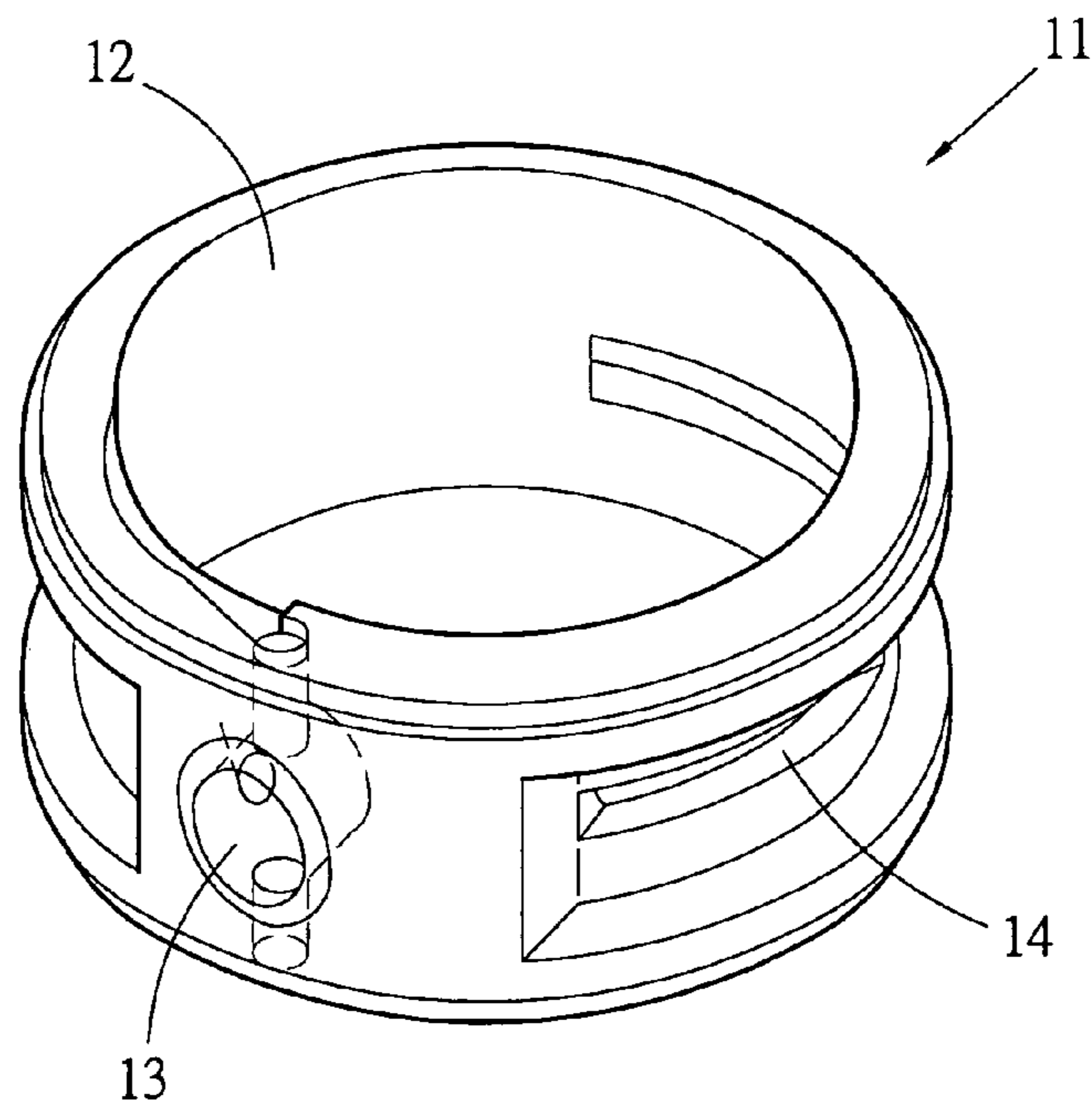
Fig. 2 Prior Art
