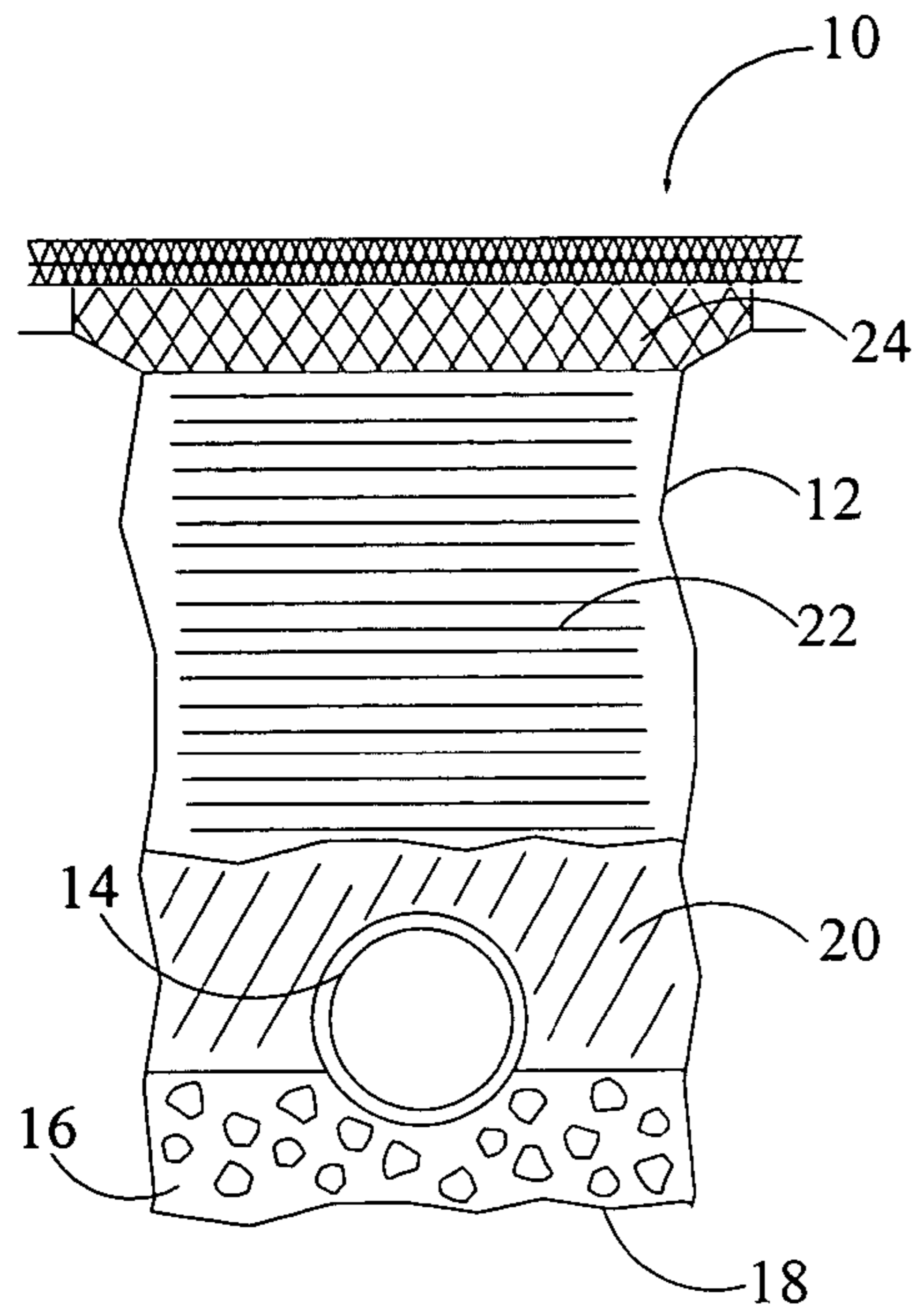
Fig. 1 (Prior Art)
