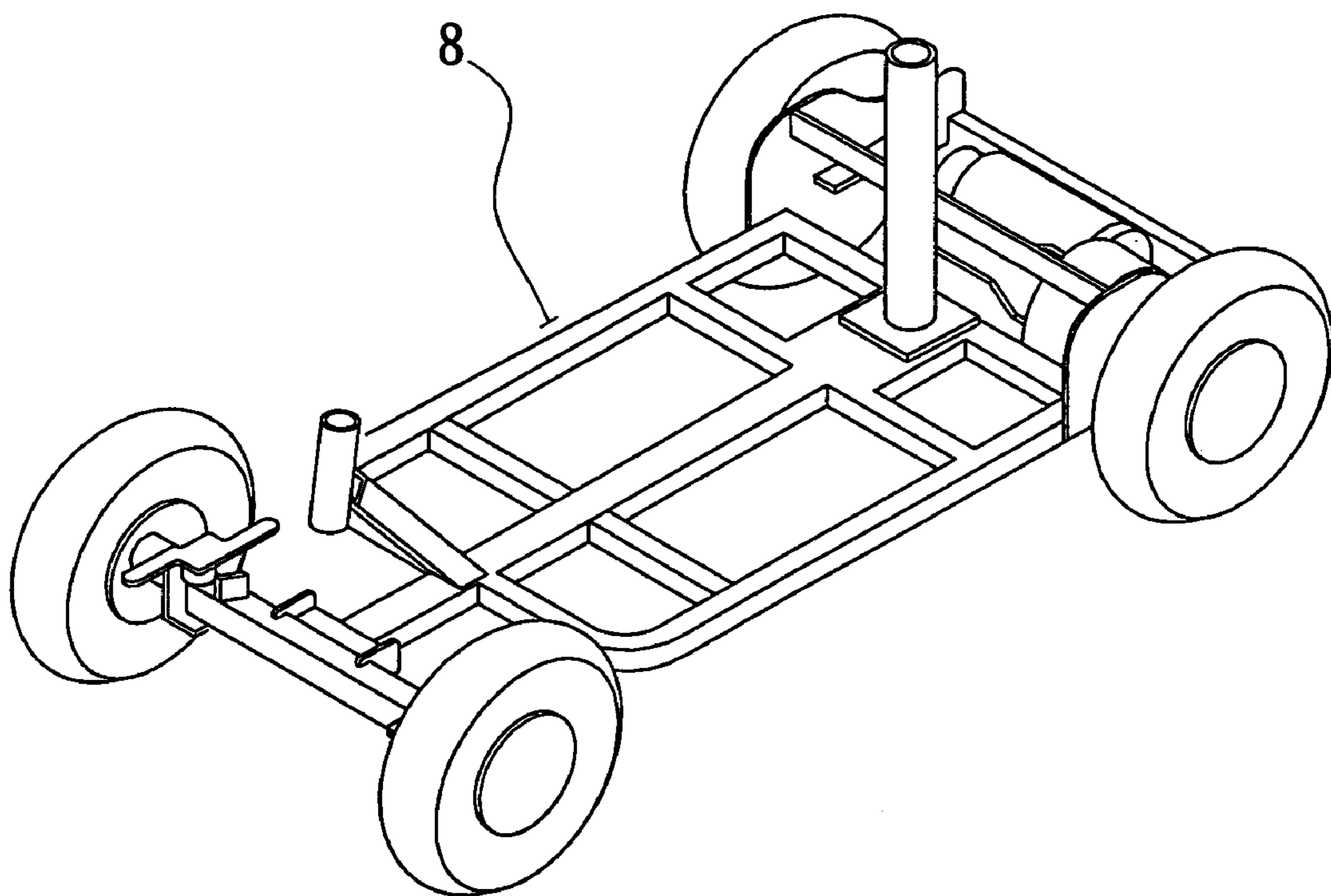
FIG. 10 (PRIOR ART)
