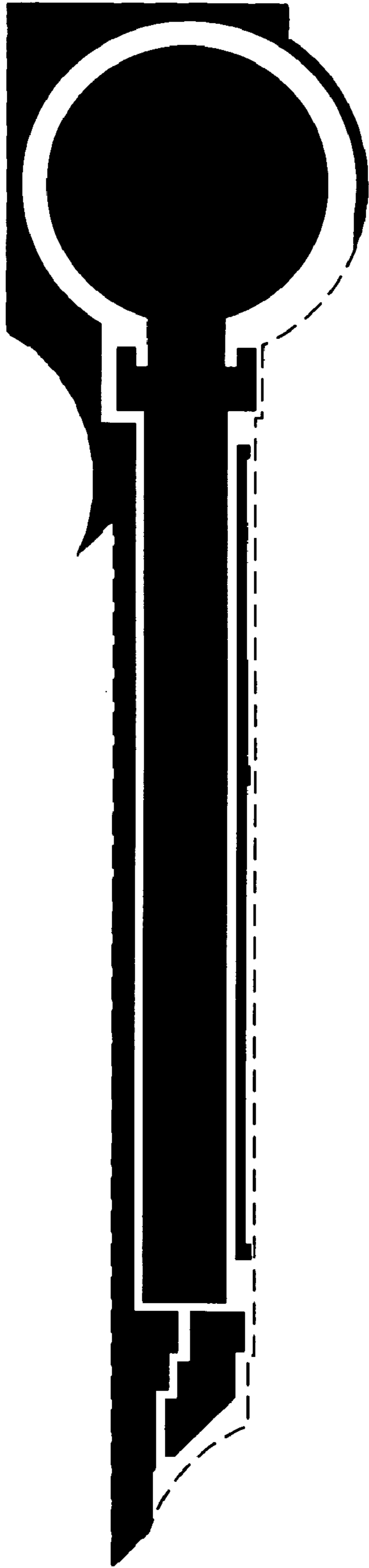
Metal 3 mask
