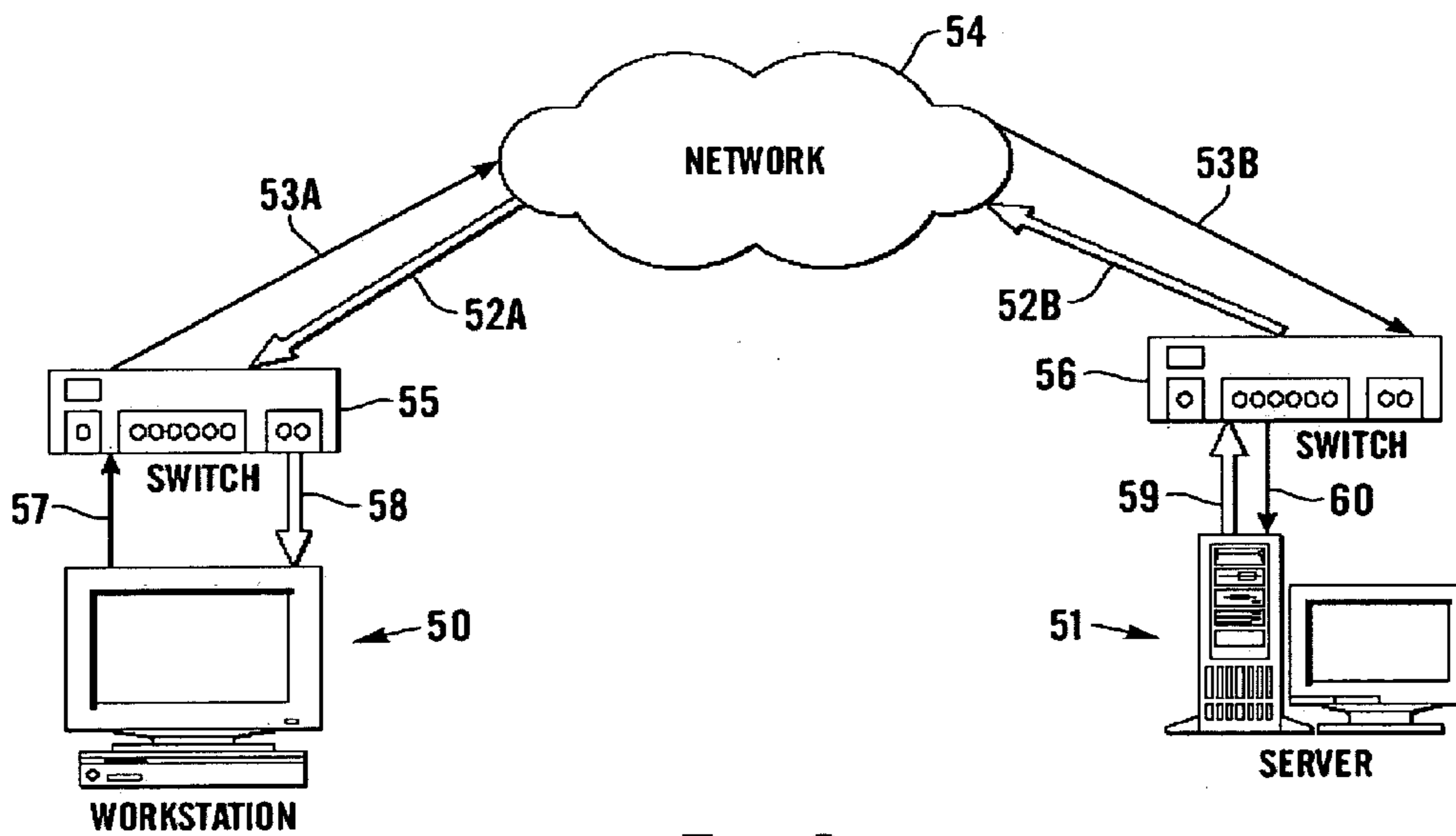
Fig.3 PRIOR ART
