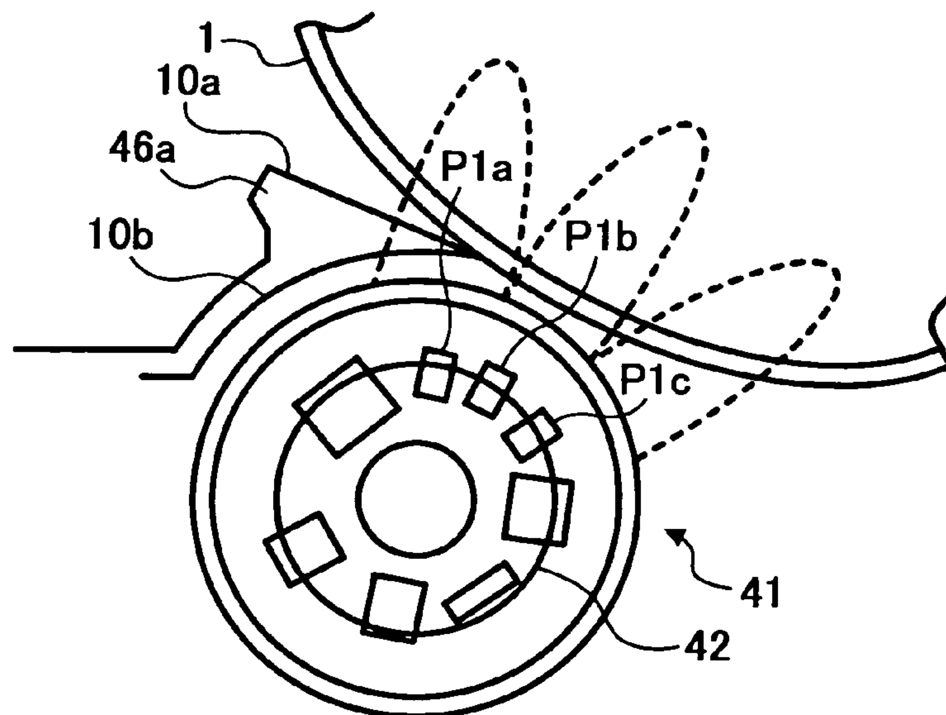
MAIN MAGNETIC POLE ANGLE OF 0 DEGREE
