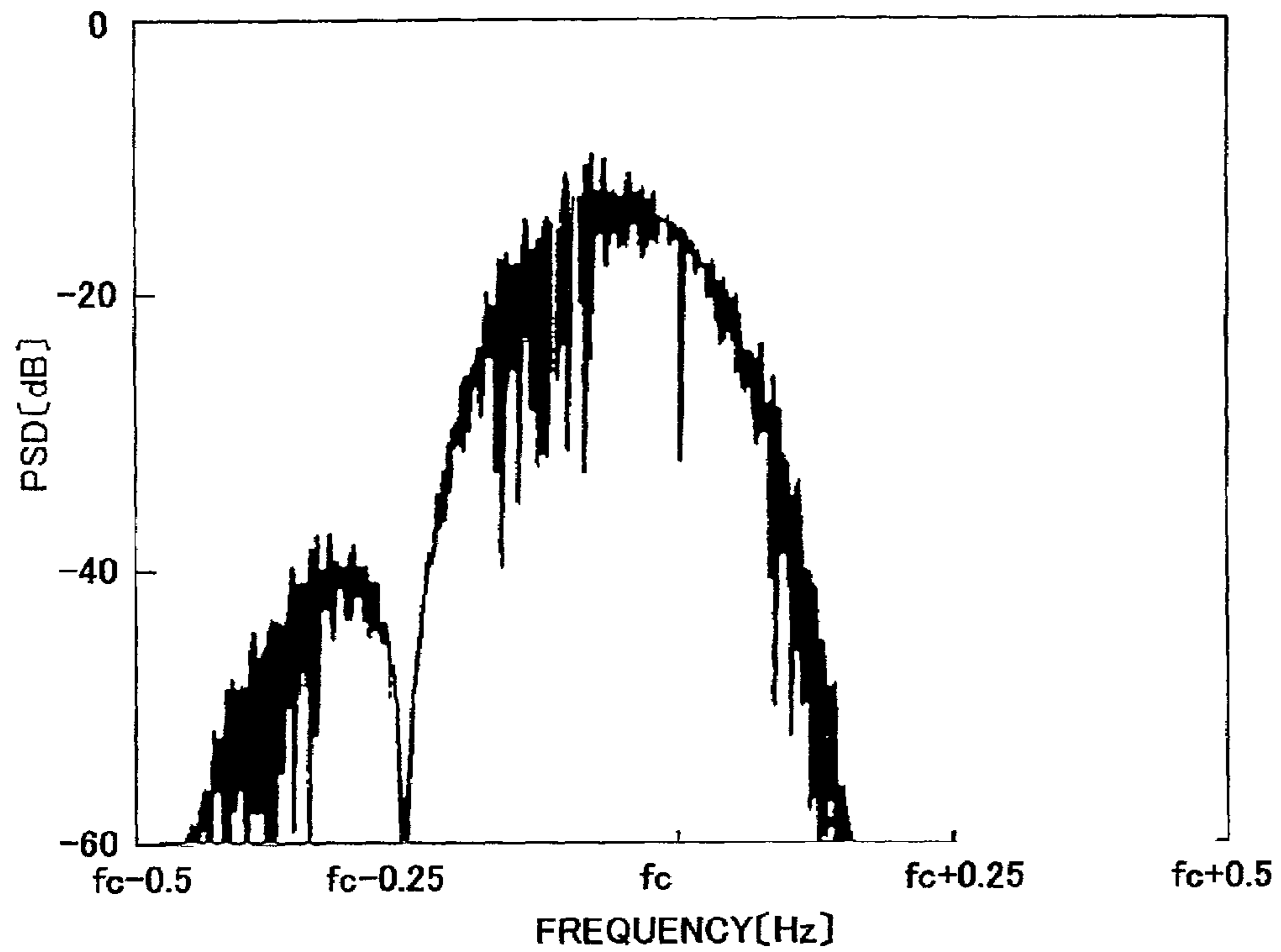
POWER SPECTRAL DENSITY CHARACTERISTIC
