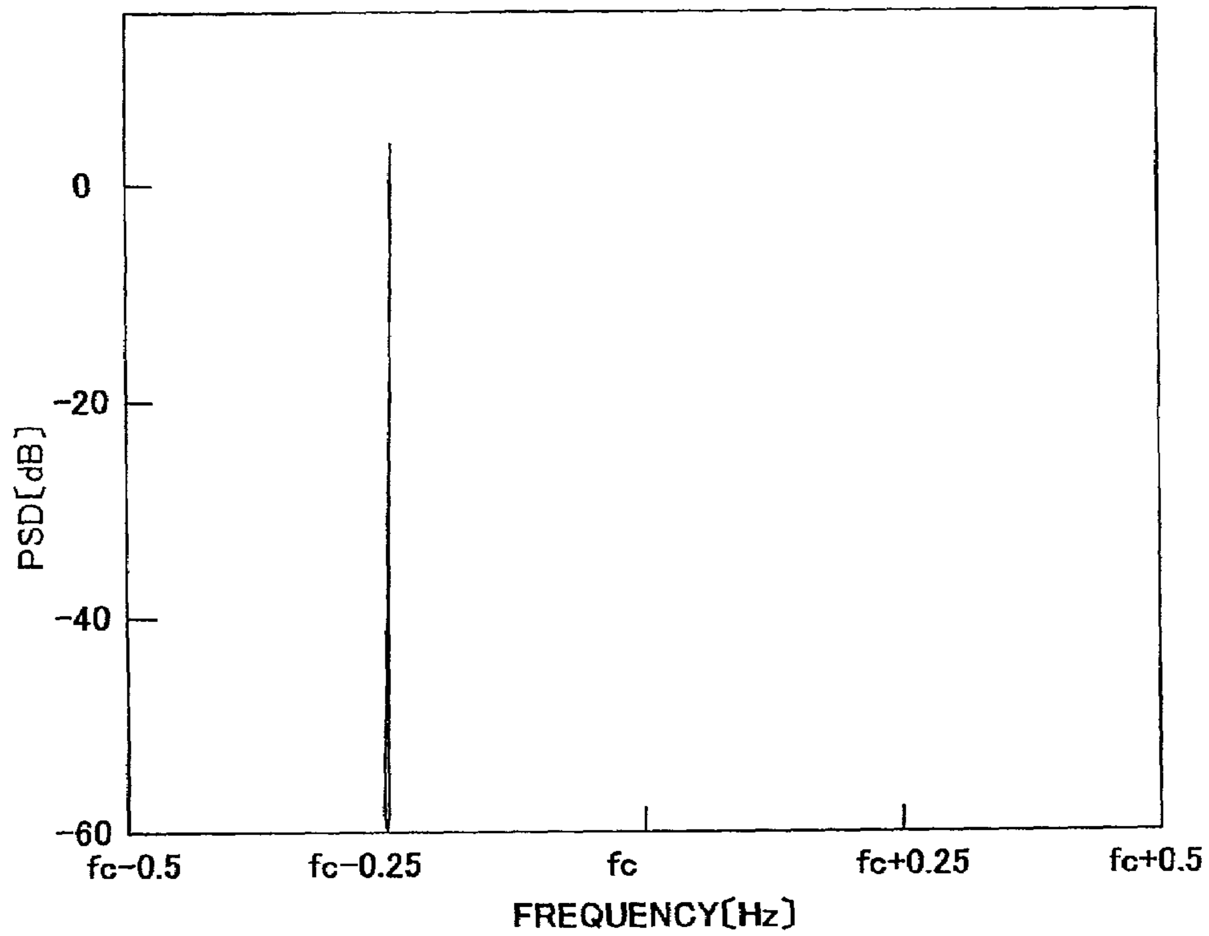
POWER SPECTRAL DENSITY CHARACTERISTIC
