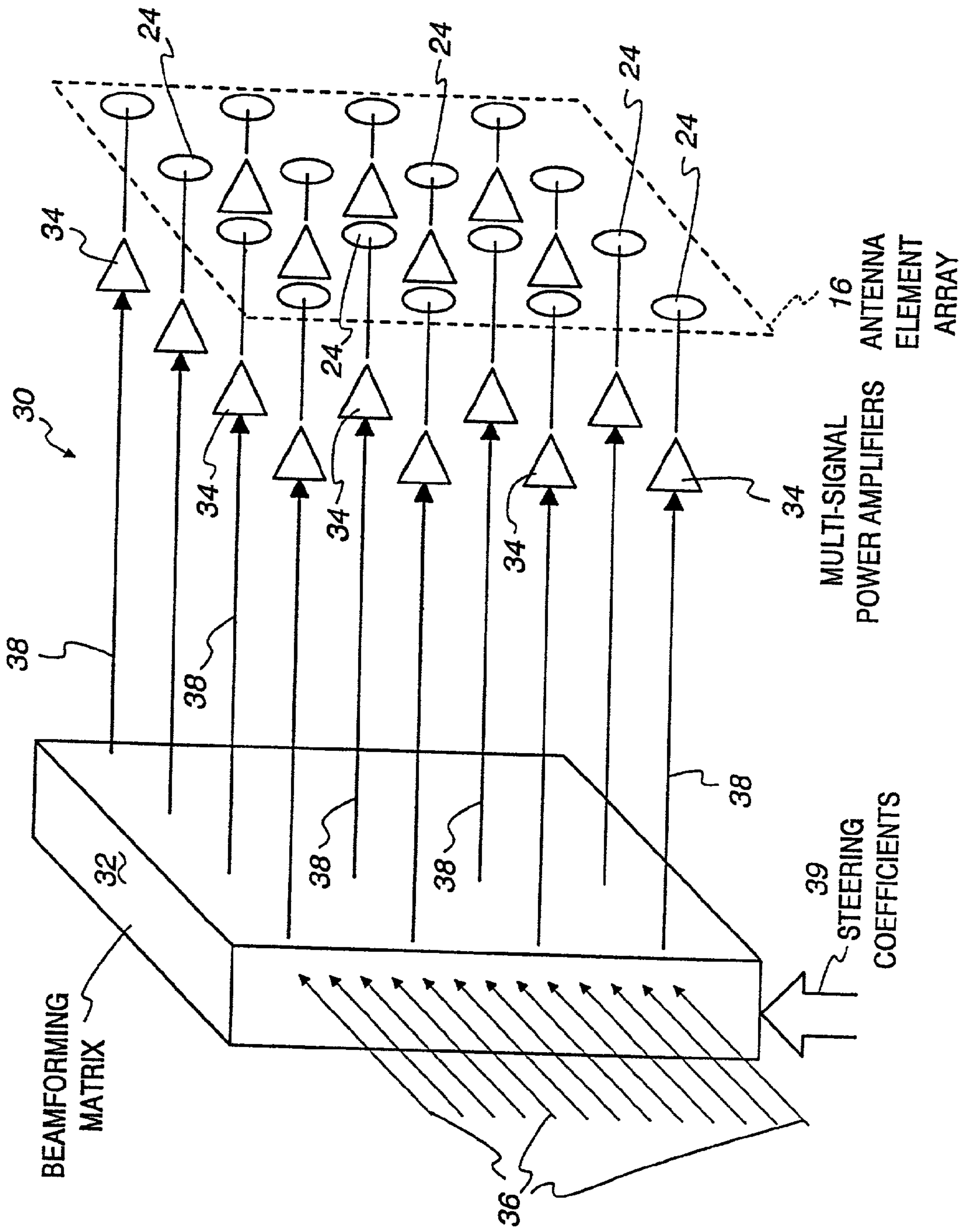
Fig. 2 (Prior Art)
