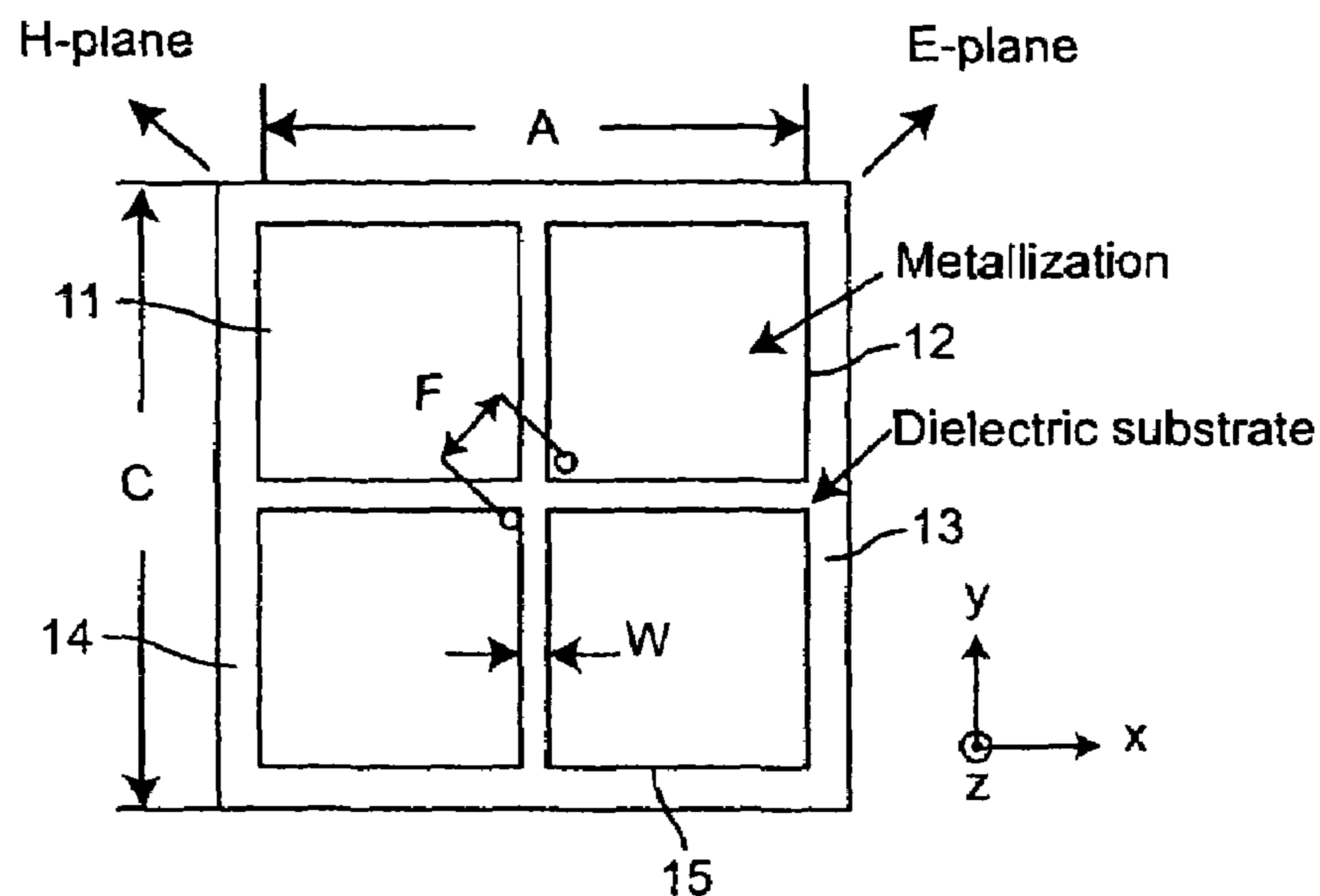
Figure 17A PRIOR ART
