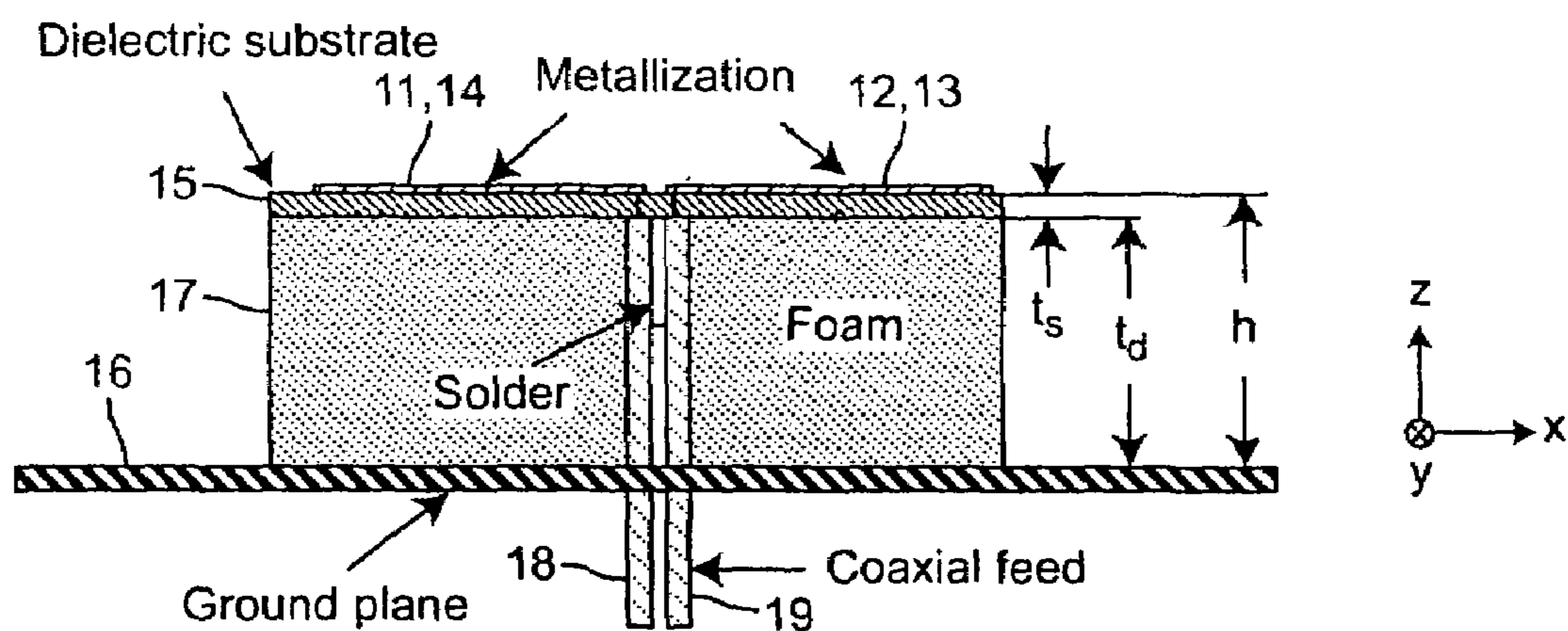
Figure 17B PRIOR ART
