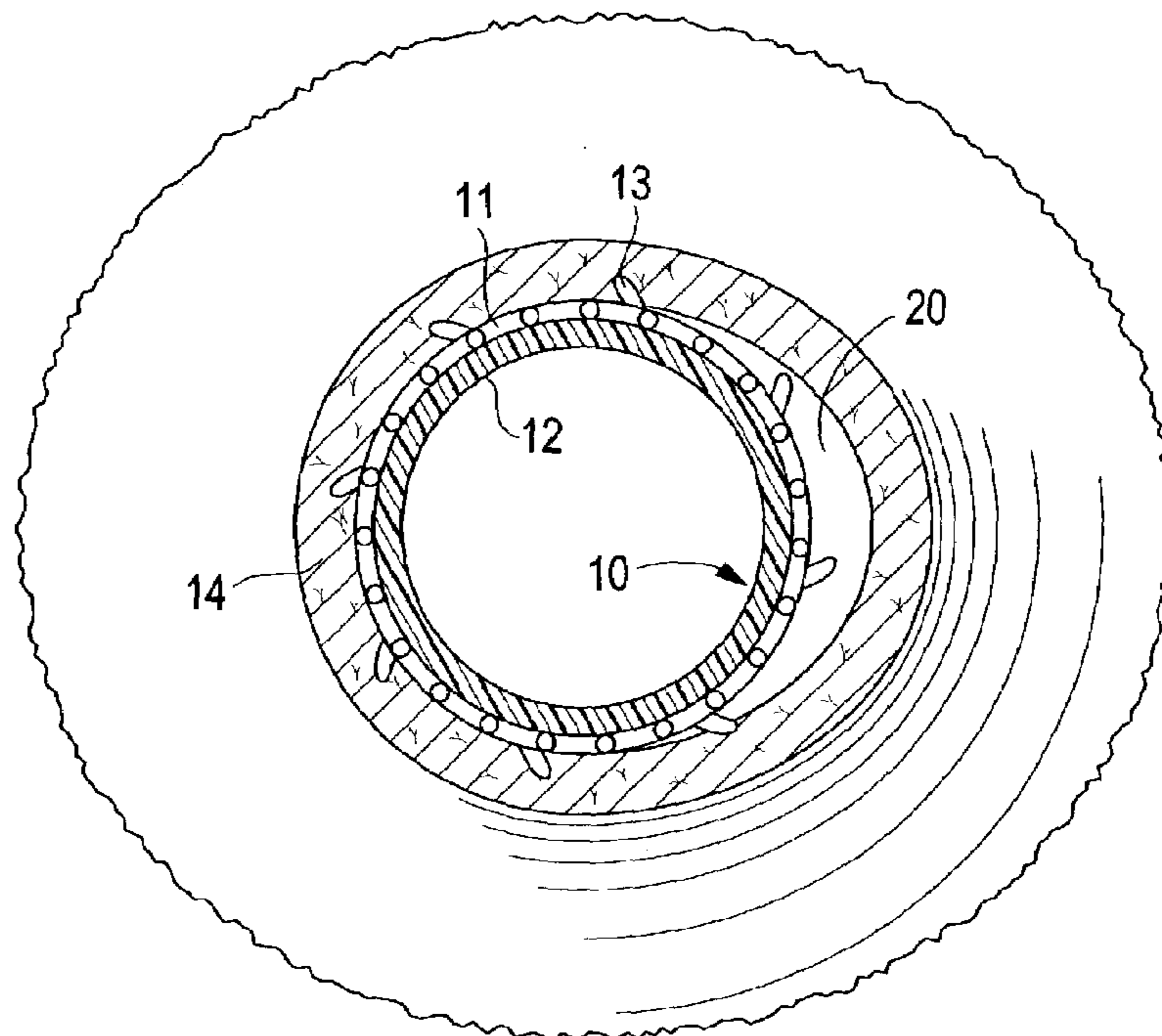
FIG. 2 PRIOR ART
