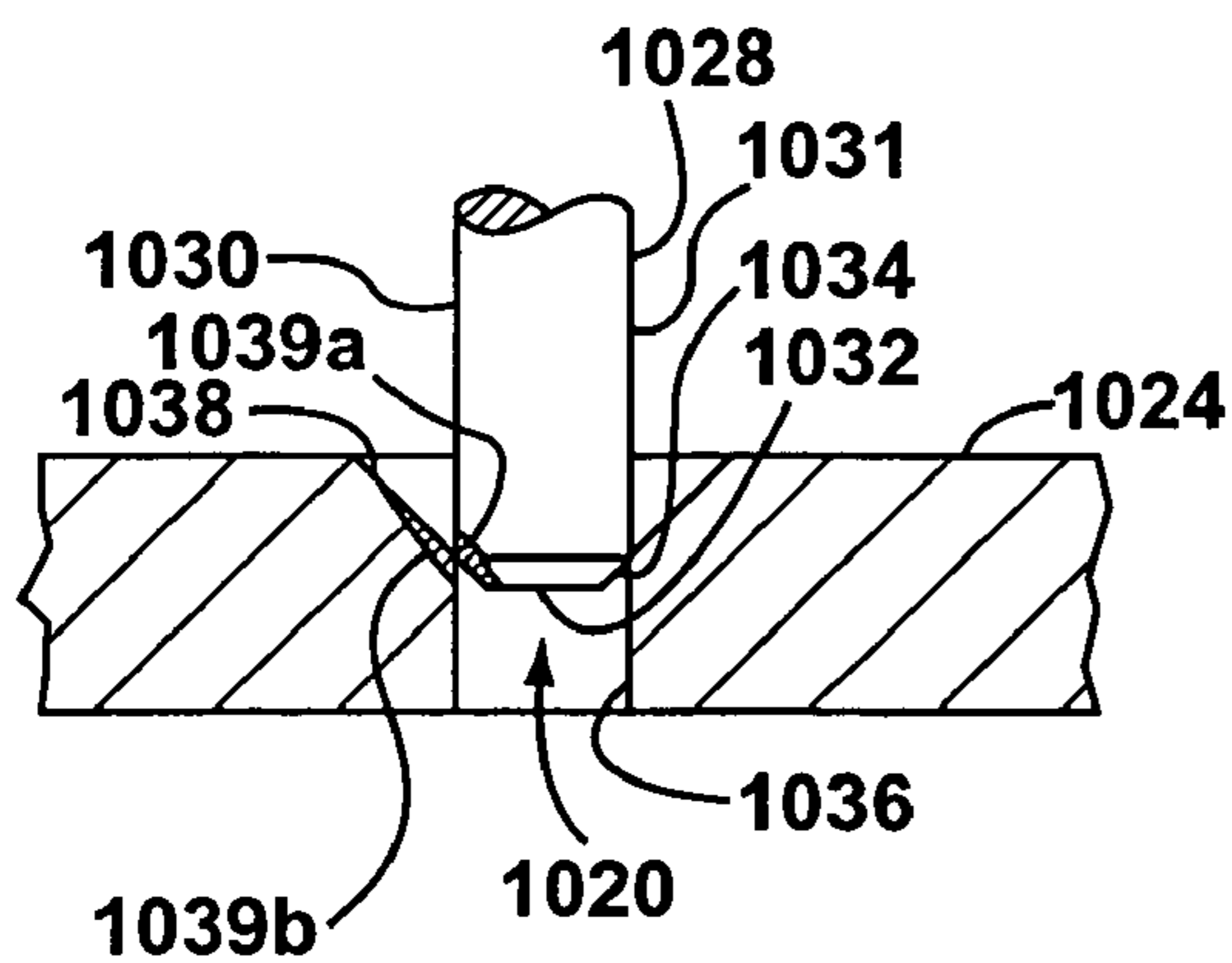
FIG. 2c (PRIOR ART)
