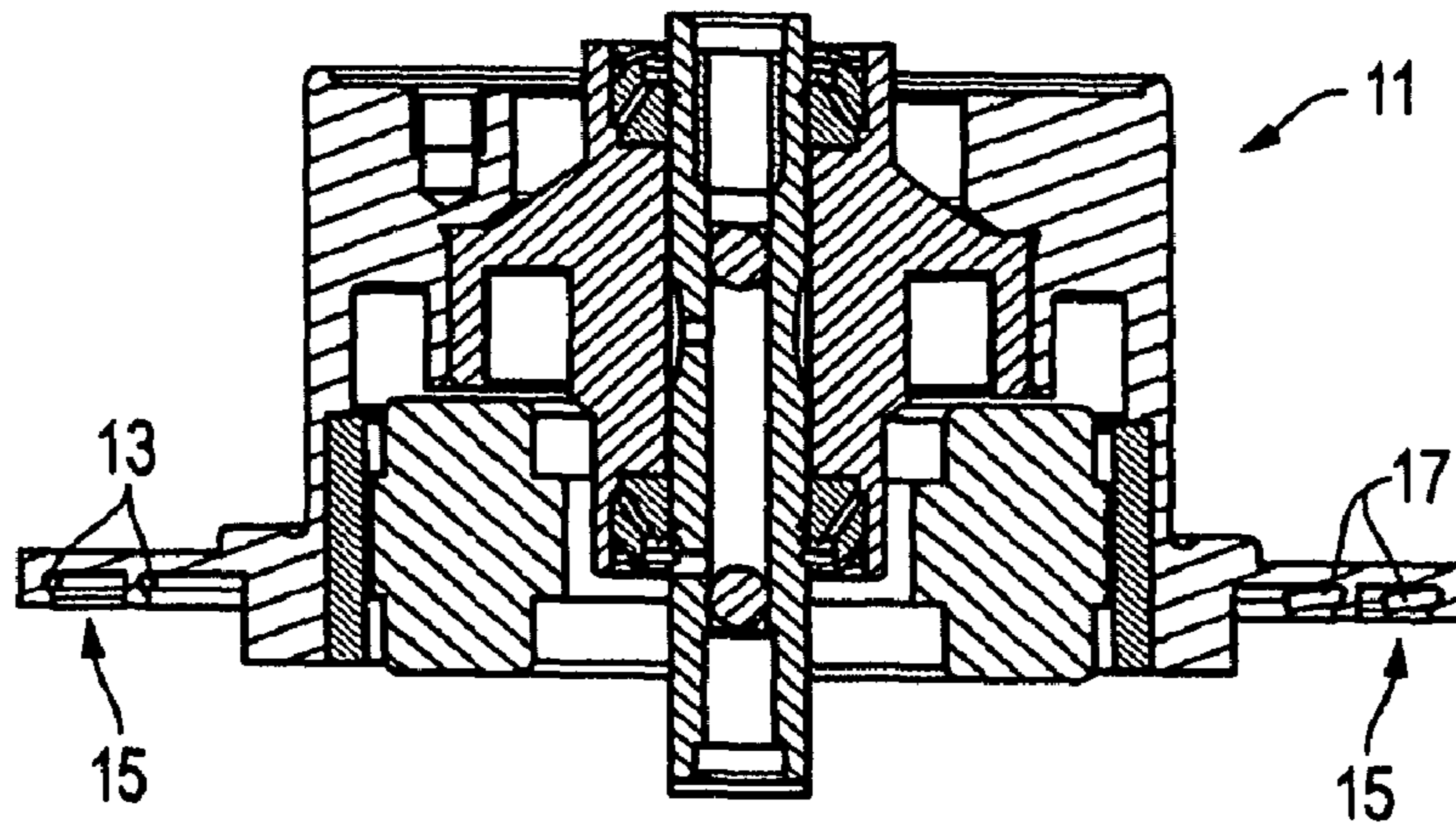
FIG. 1 (Prior Art)
