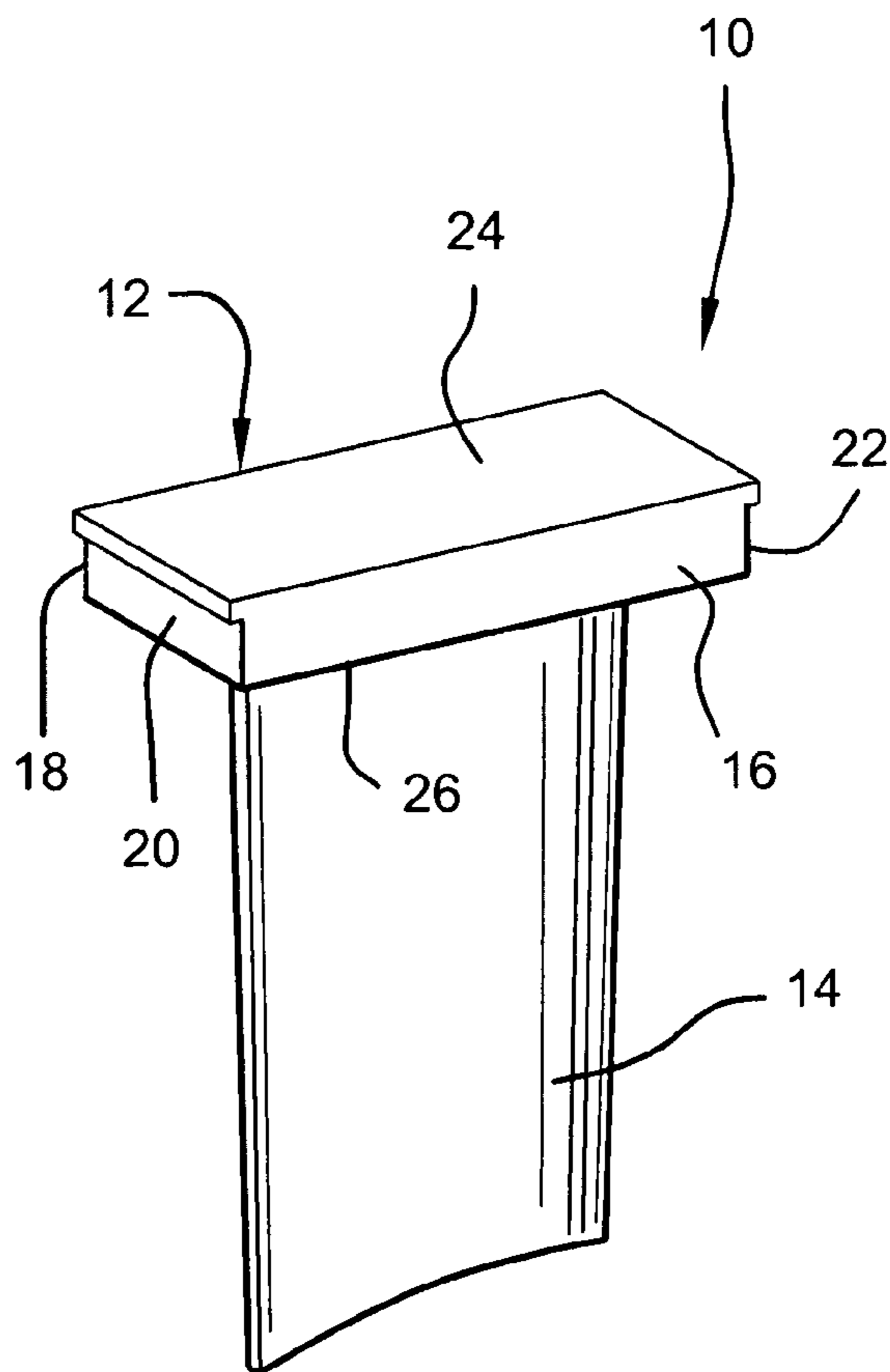
Fig. 2 (Prior Art)
