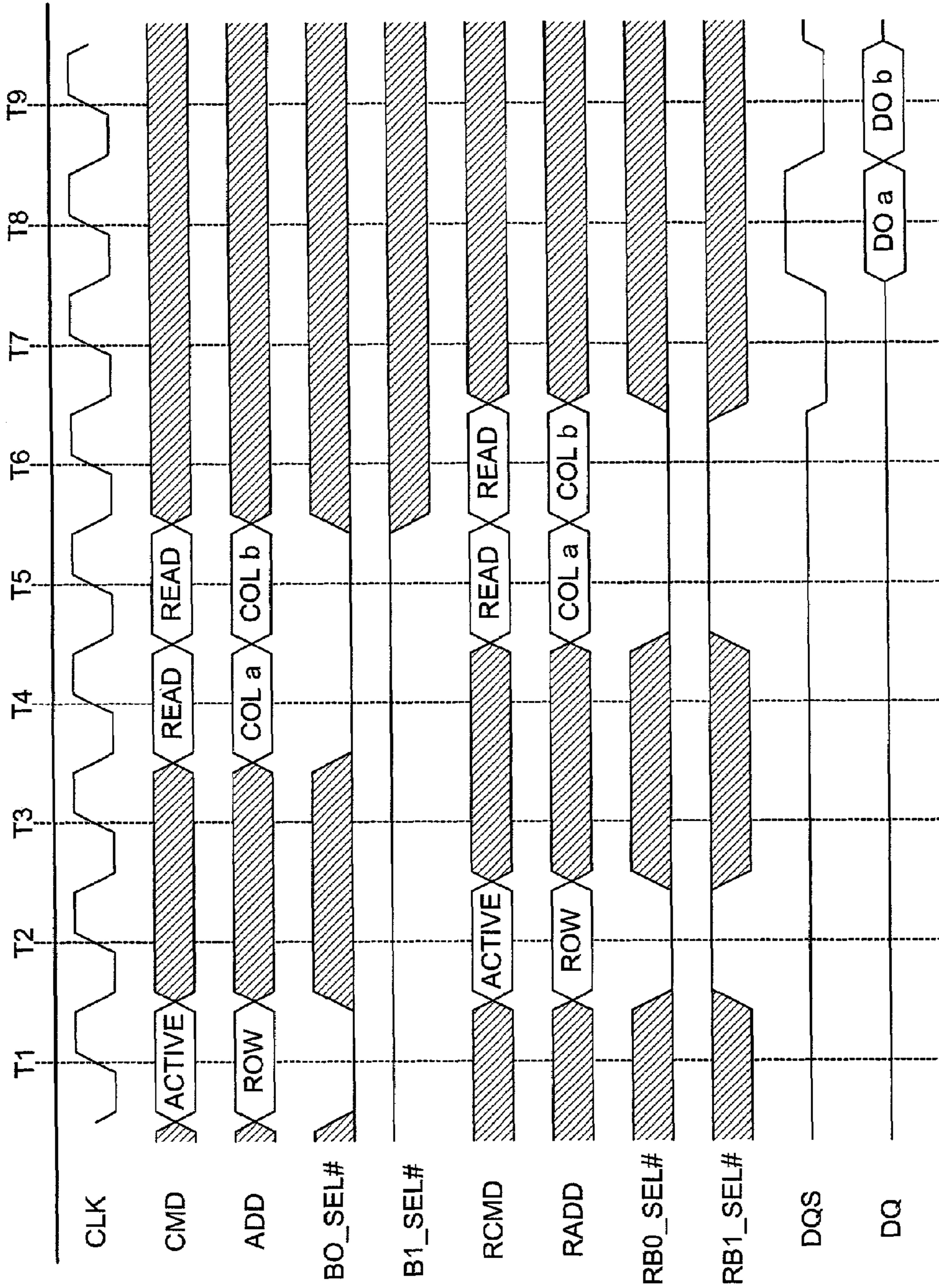
Fig. 3 (Prior Art)
