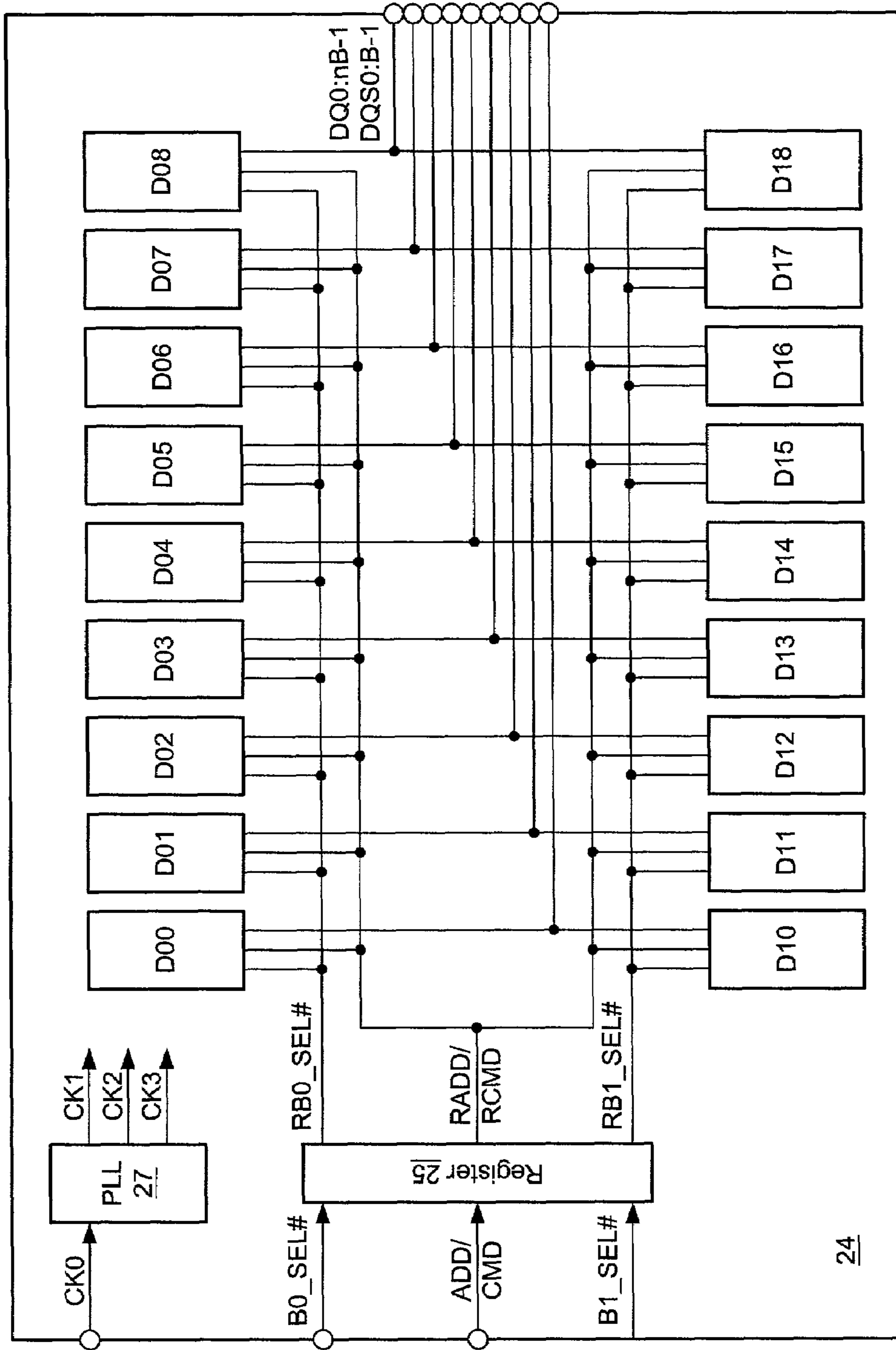
Fig. 2 (Prior Art)
