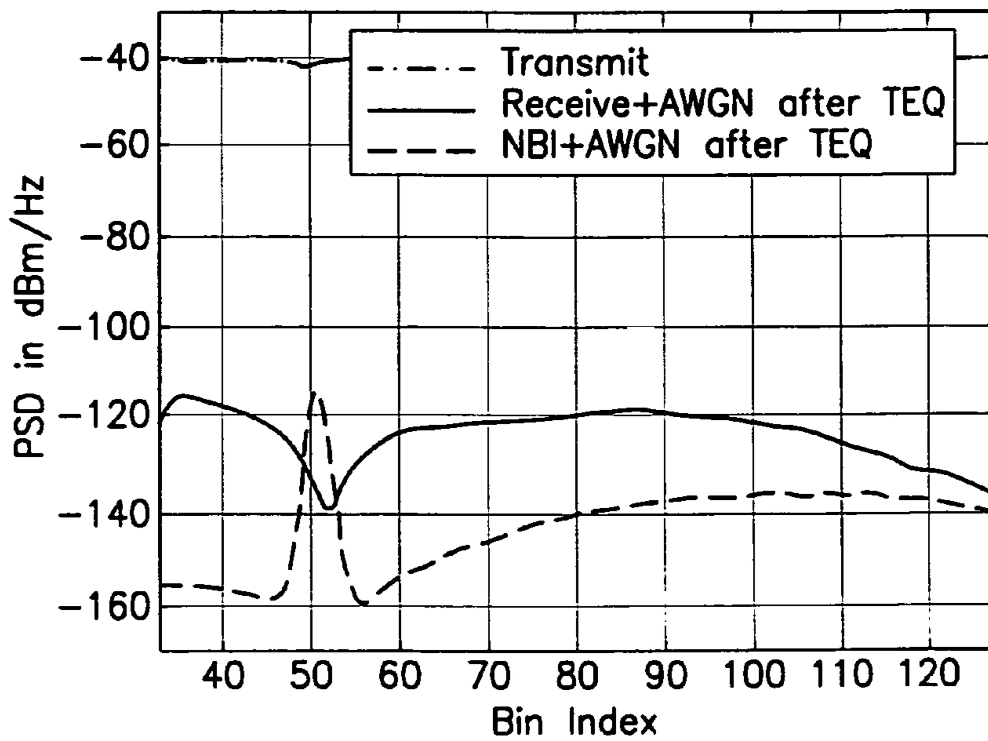
Long Loop With NBI Signal And Noise PSD'S After TEQ
