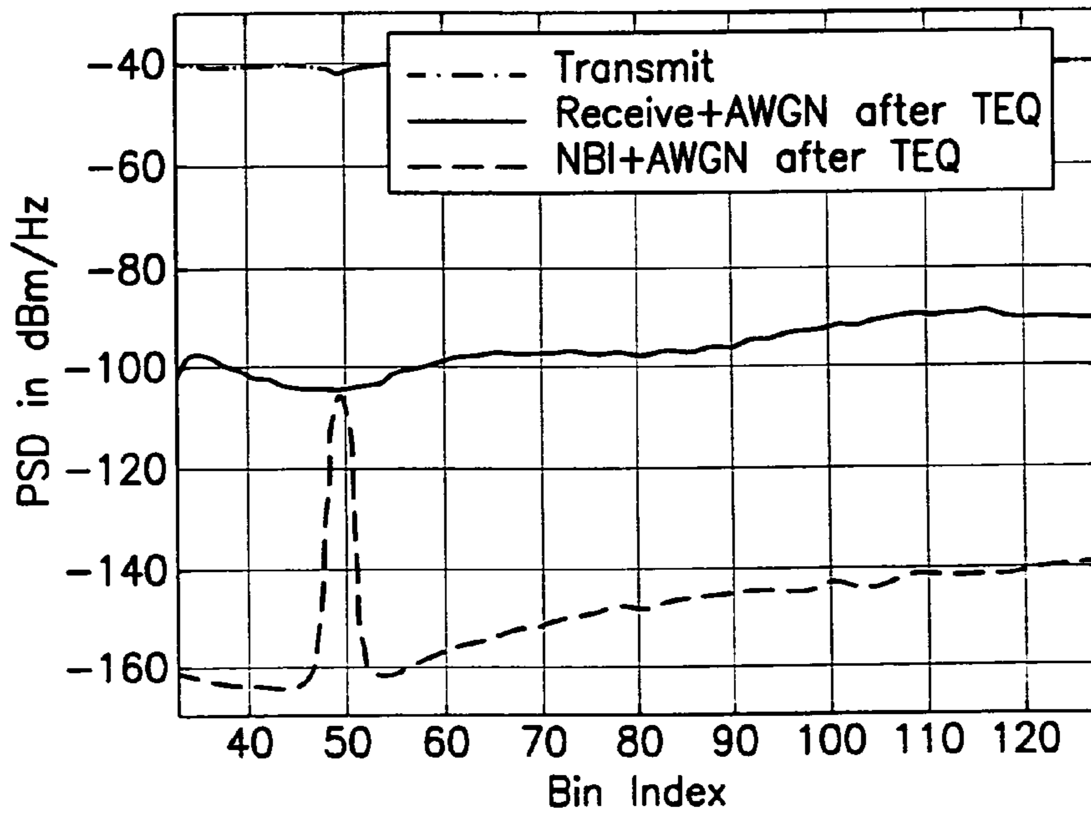
Medium Loop with NBI Signal And Noise PSD'S After TEQ
