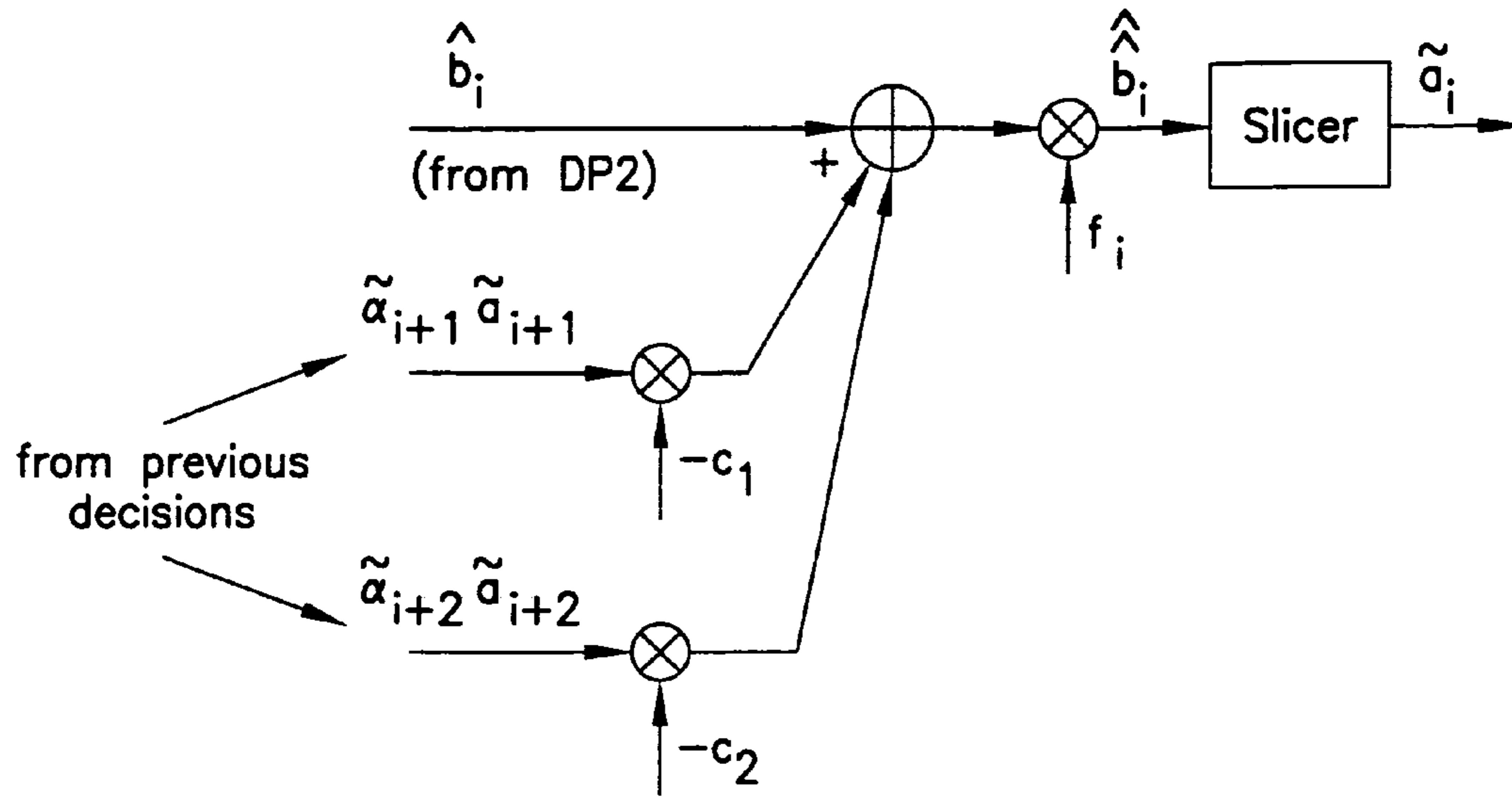
DFE with 2 feedback taps
