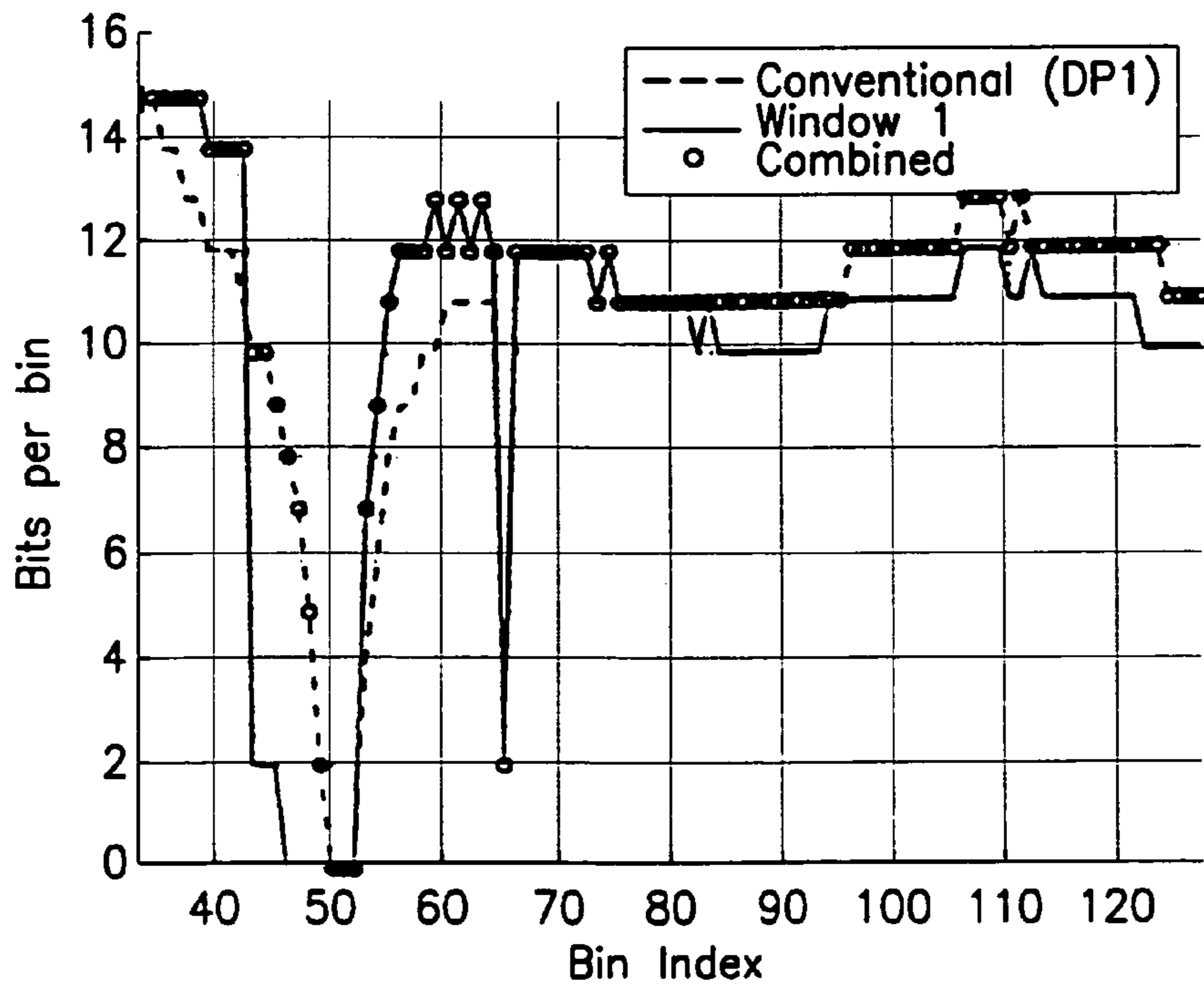
Medium Loop With NBI Bit-Allocation Profile
