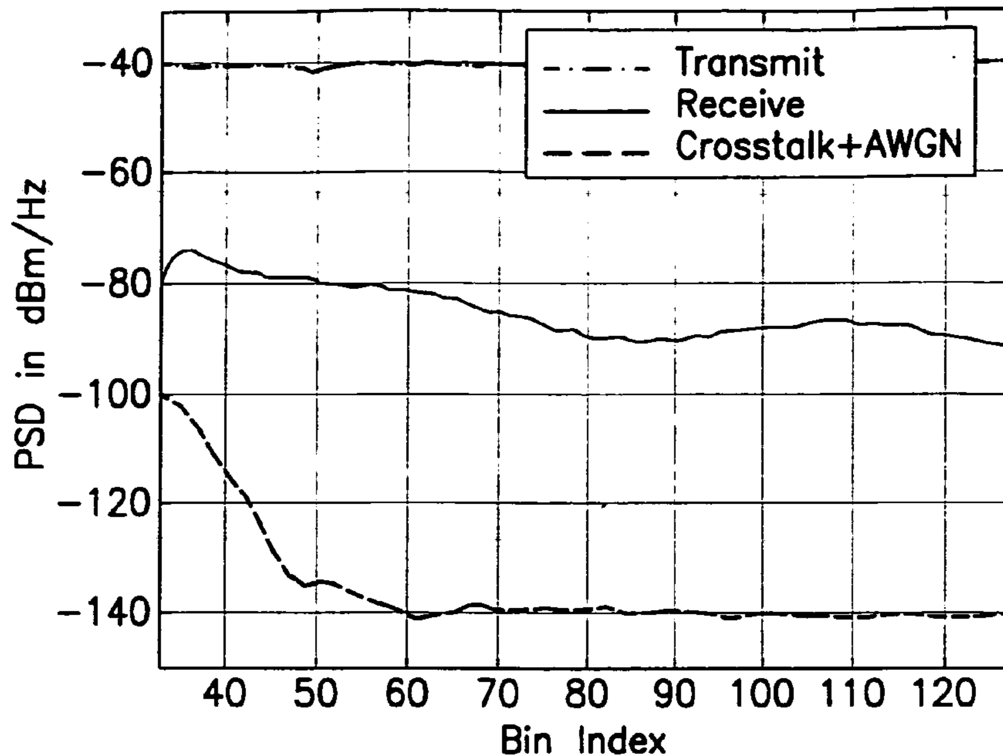
Medium Loop With Crosstalk Signal And Noise PSD'S Before TEQ
