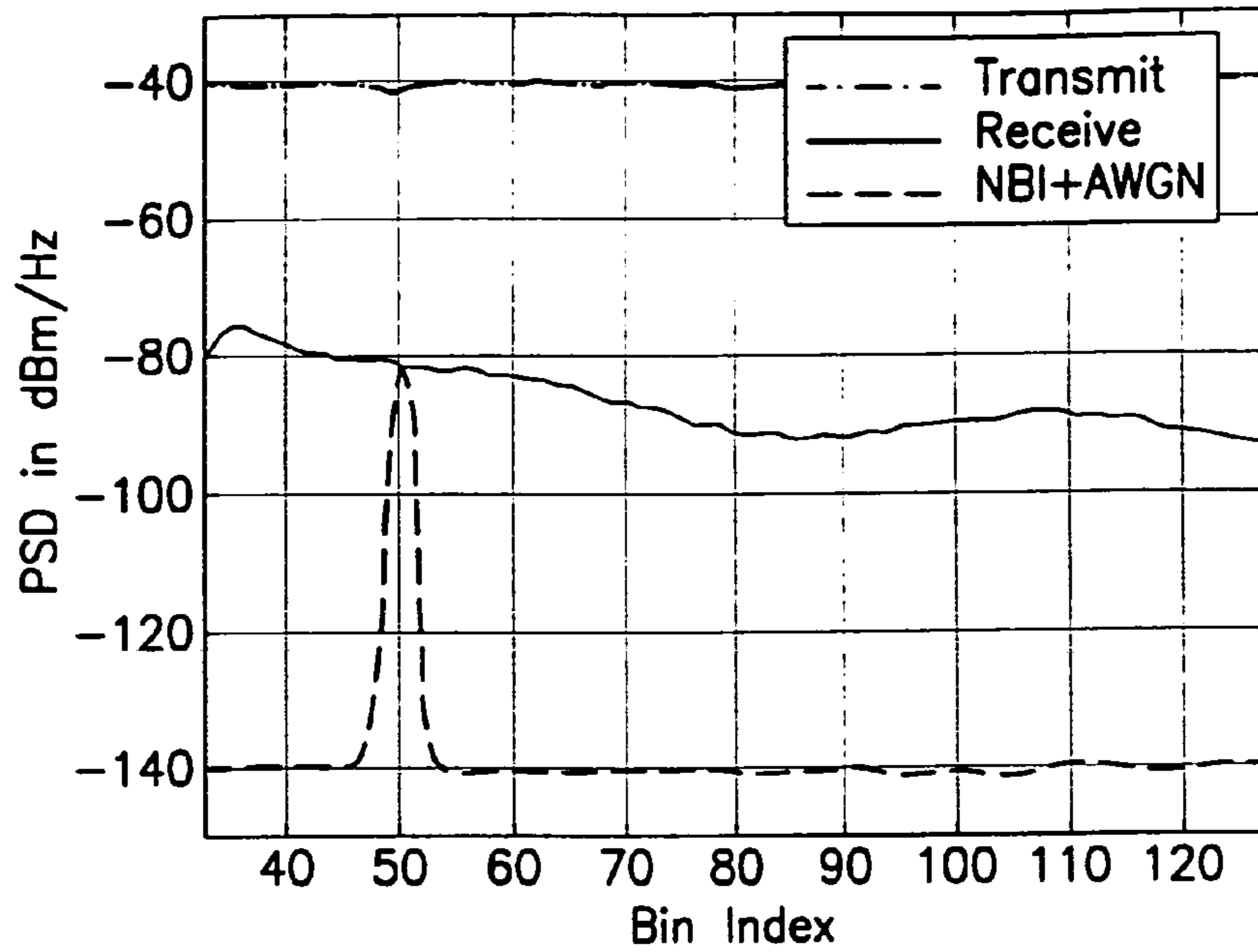
Medium Loop with NBI Signal And Noise PSD'S Before TEQ
