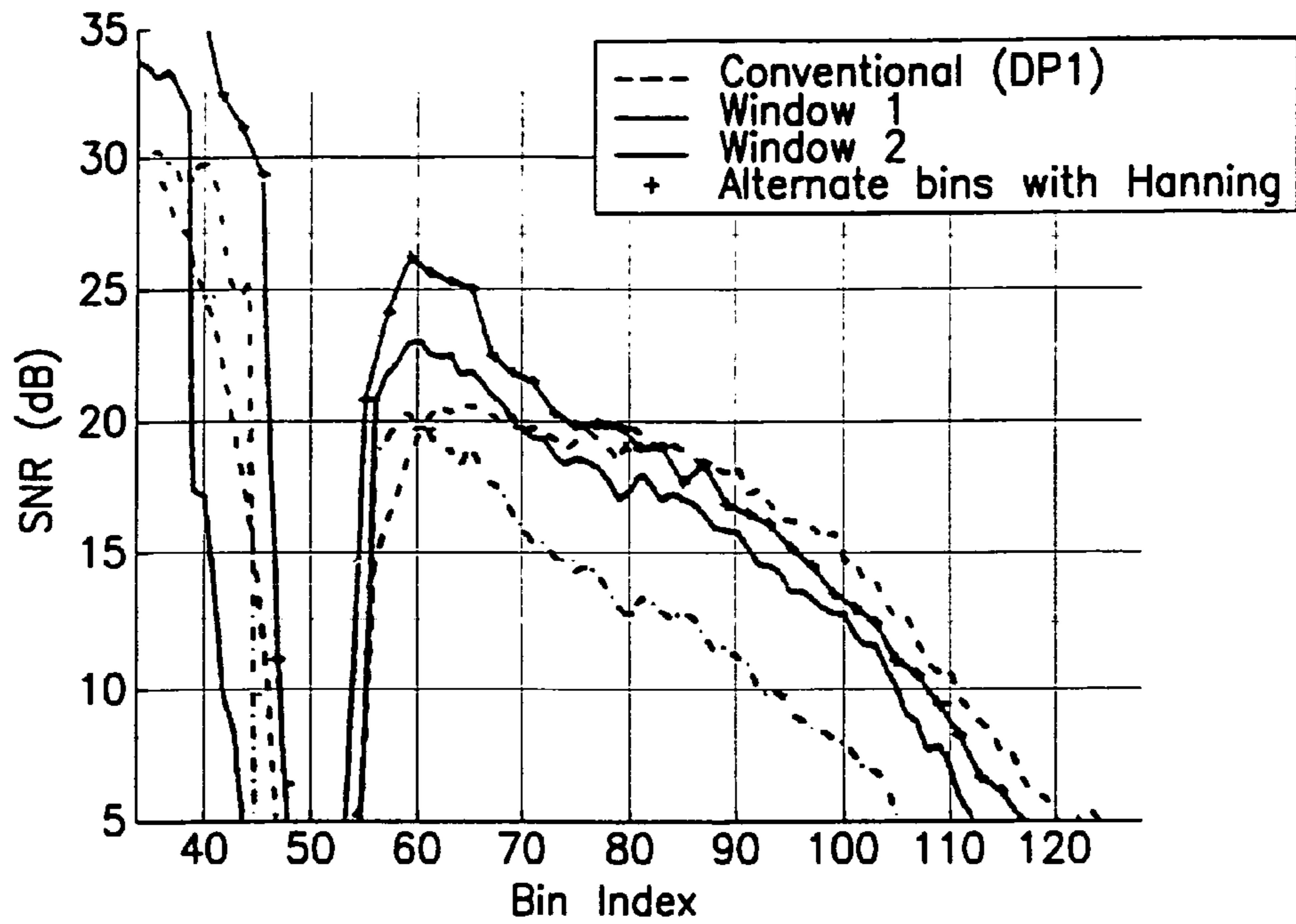
Long Loop With NBI Profile
