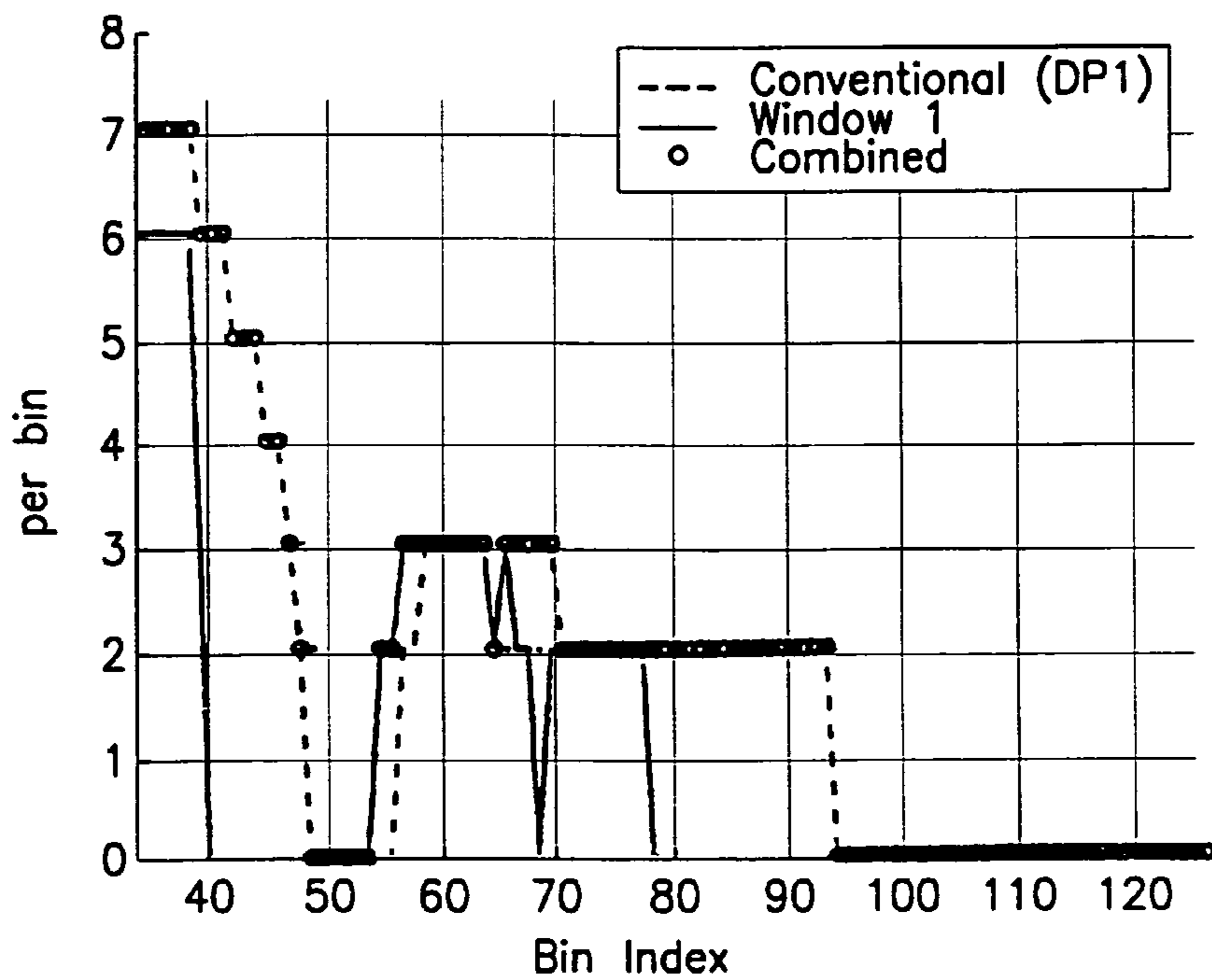
Long Loop With NBI Bit-Allocation Profile
