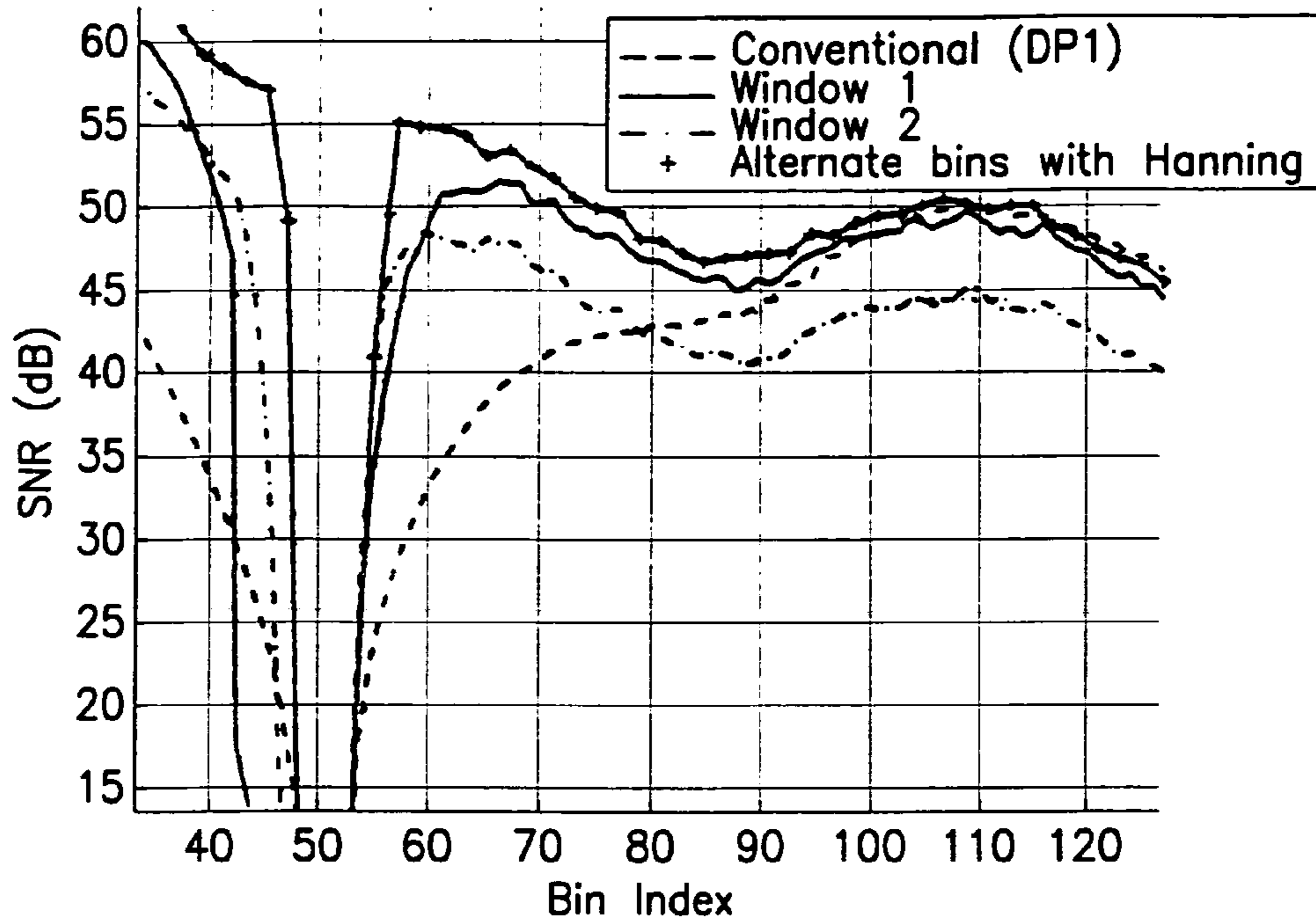
Medium Loop With NBI SNR Profile
