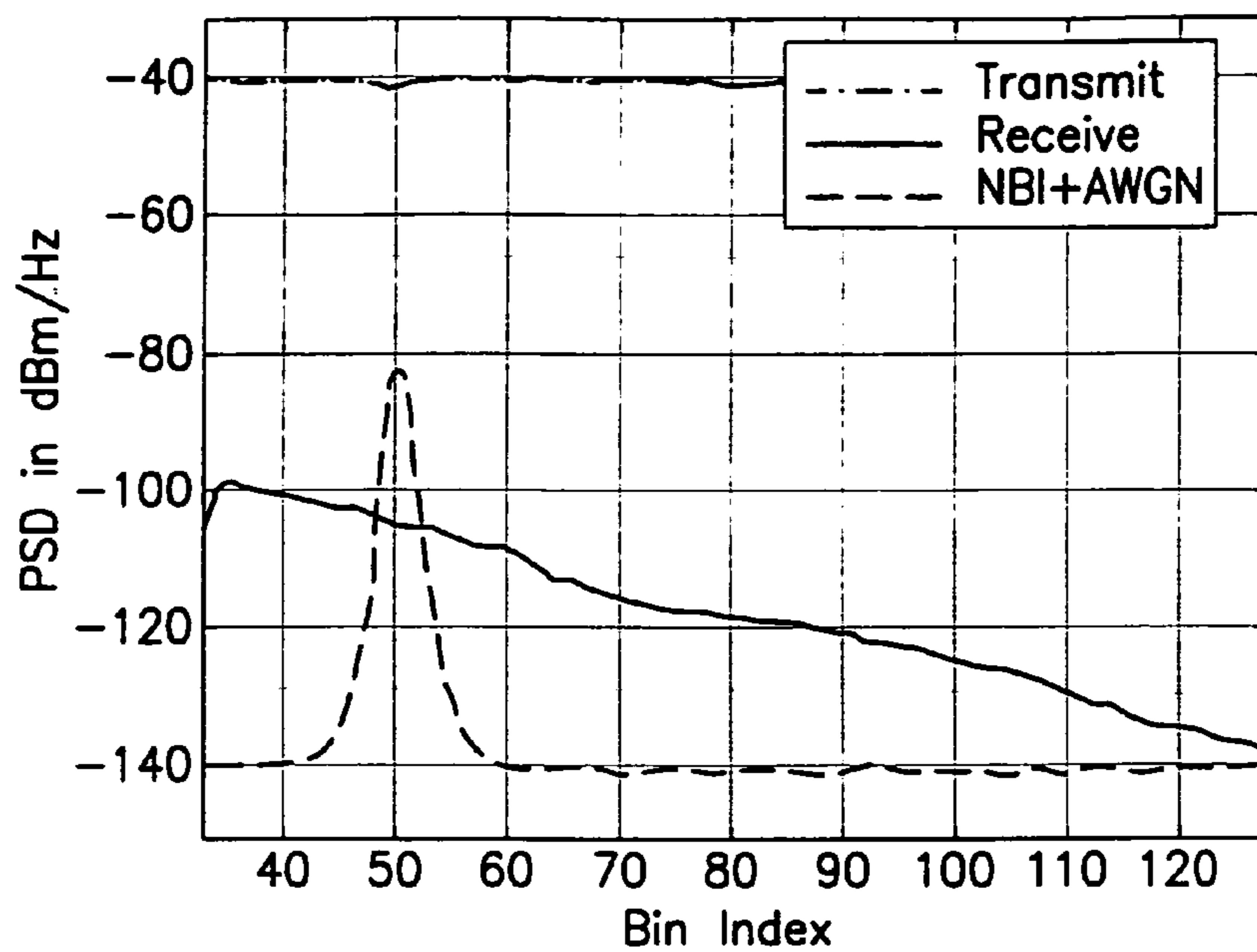
Long Loop With NBI Signal And Noise PSD'S Before TEQ
