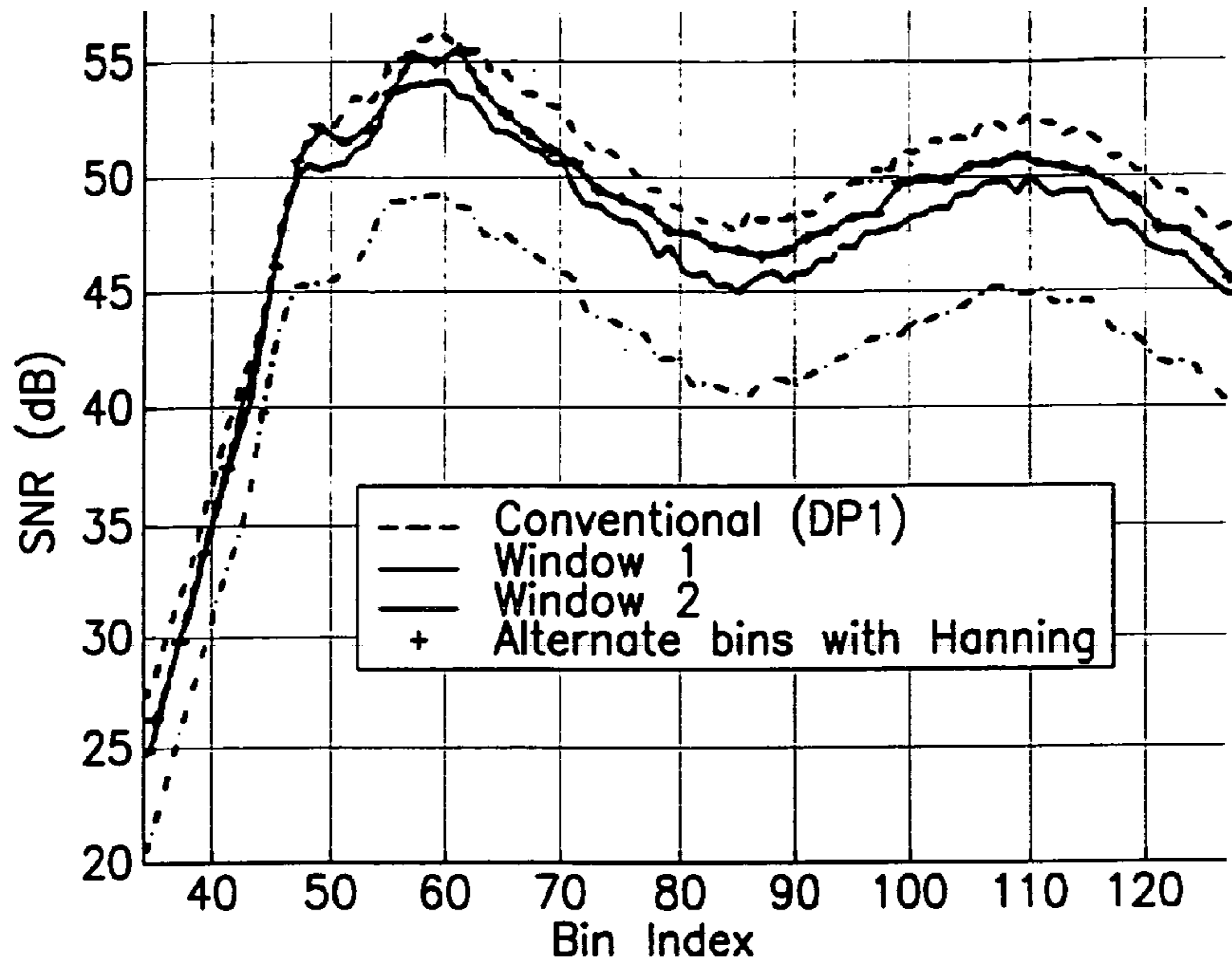
Medium Loop With Crosstalk SNR Profile
