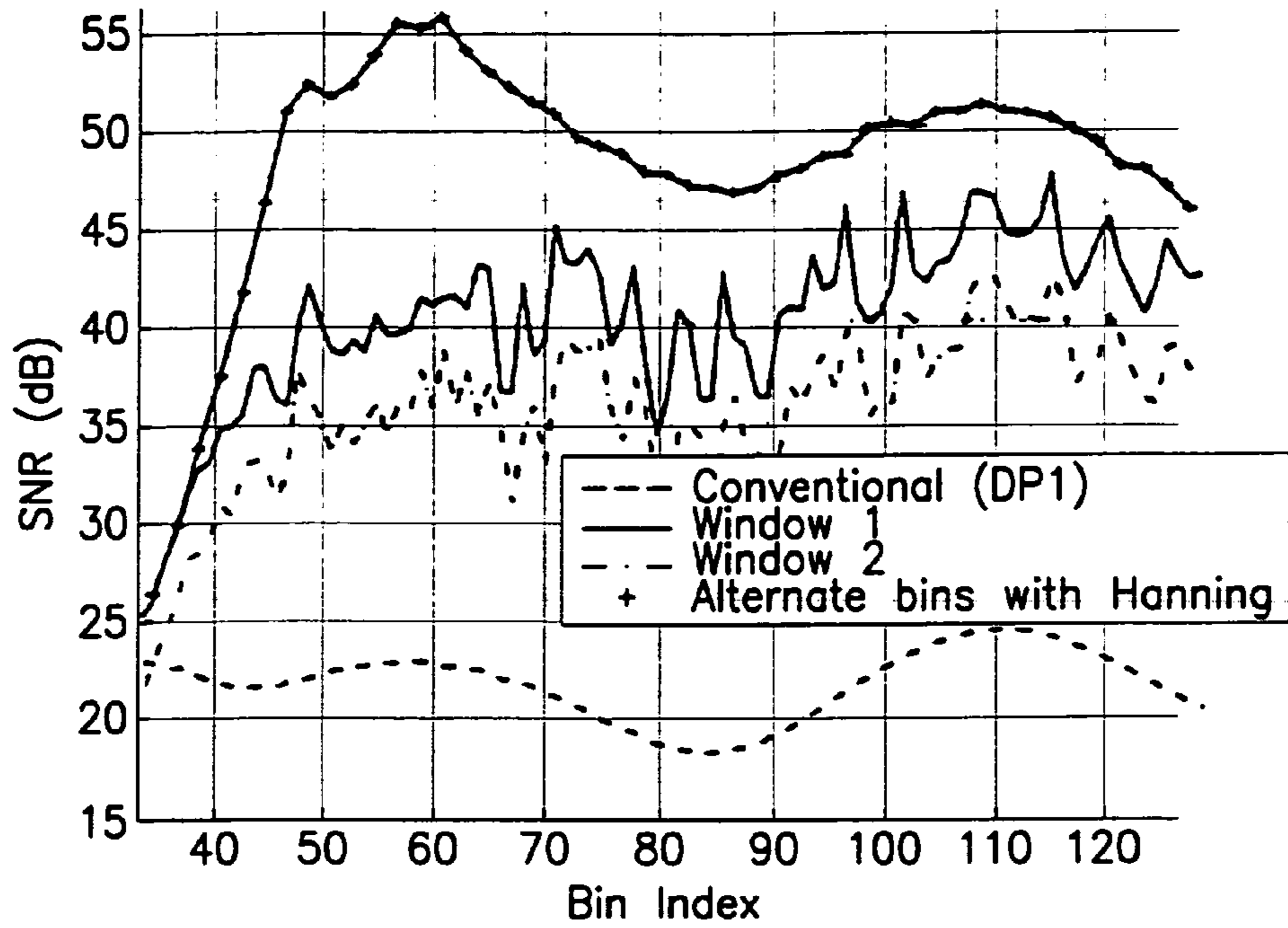
Medium Loop With Crosstalk Without TEQ SNR Profile
