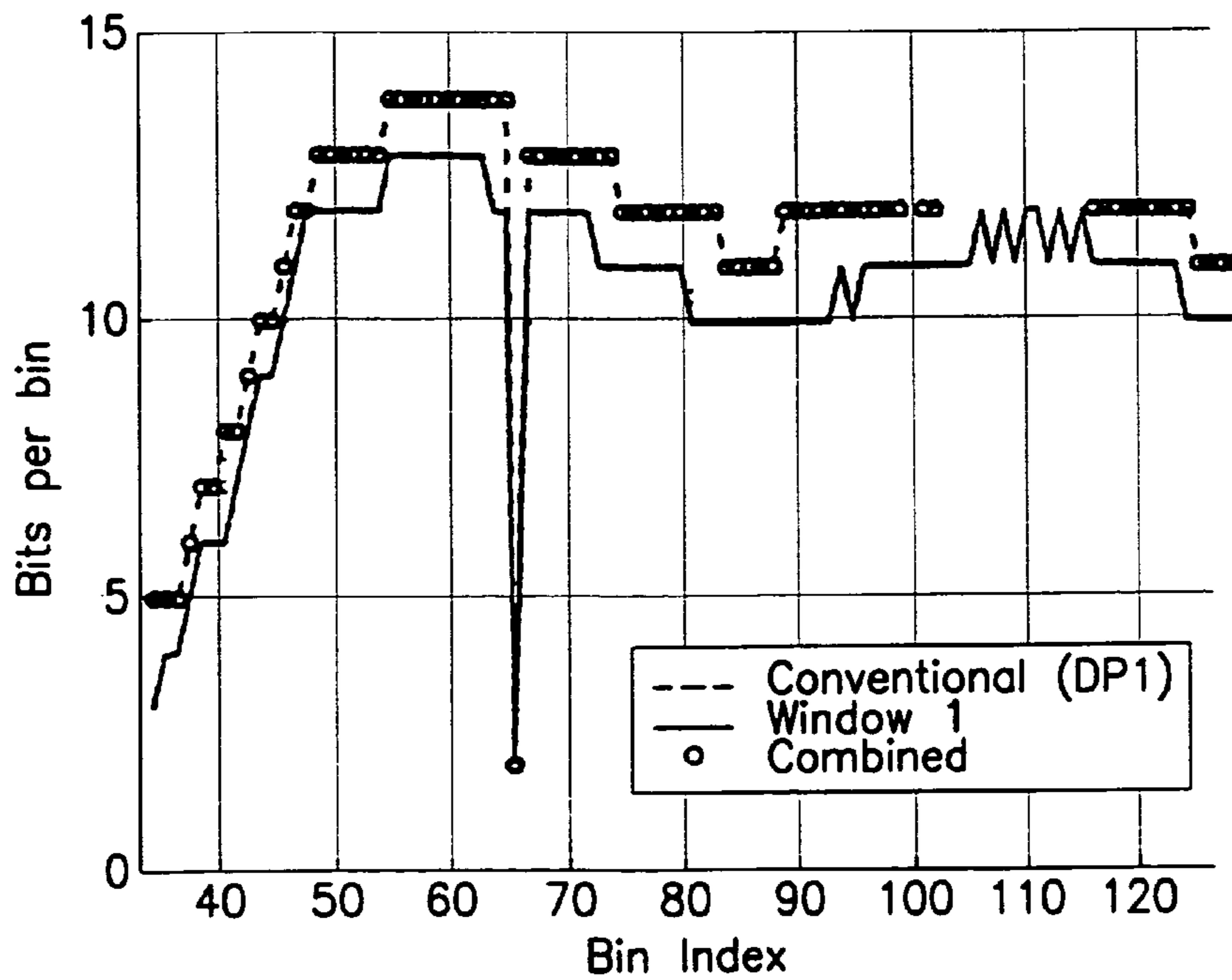
Medium Loop With Crosstalk Bit Allocation Profile
