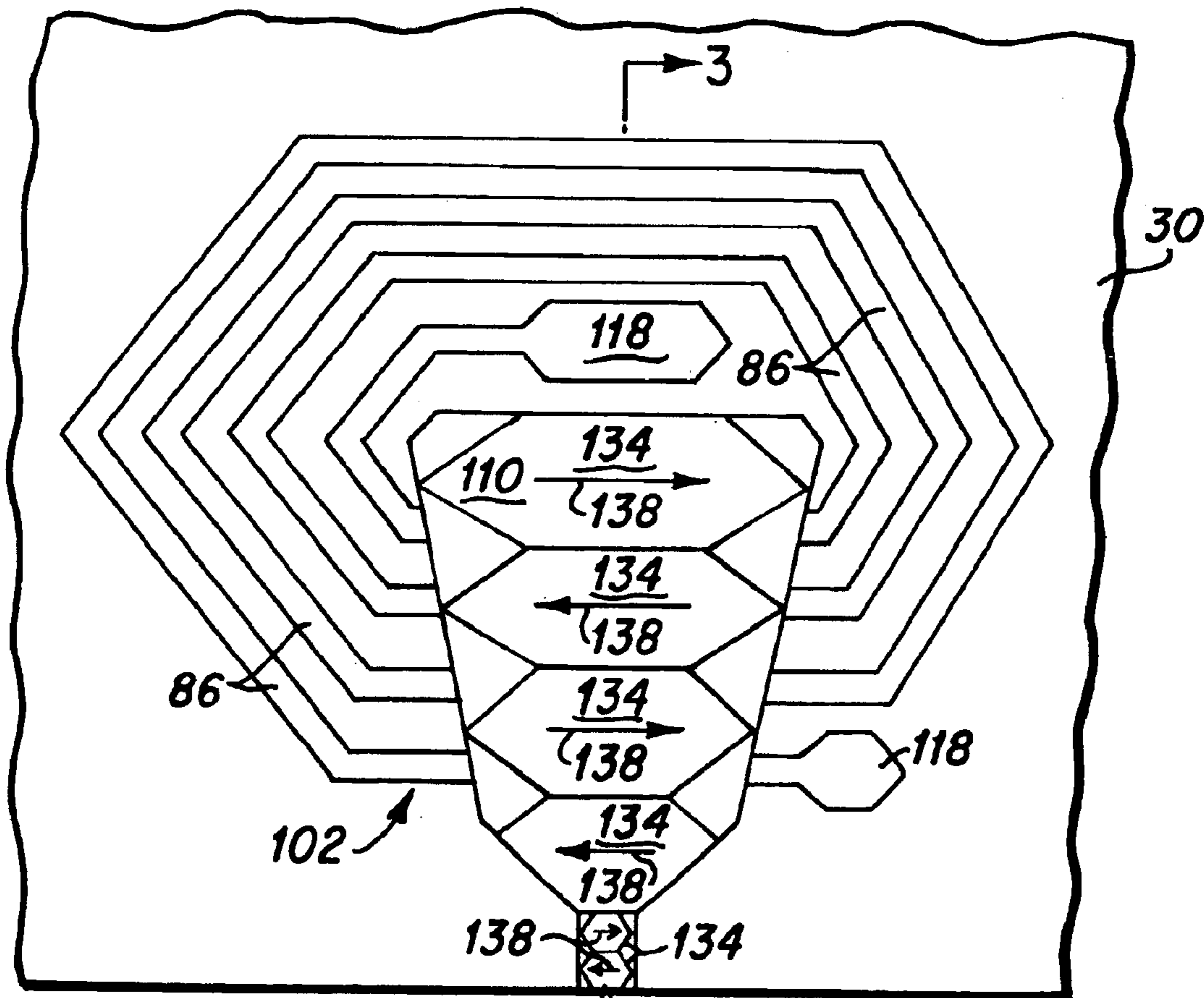
Fig.2 (PRIOR ART)
