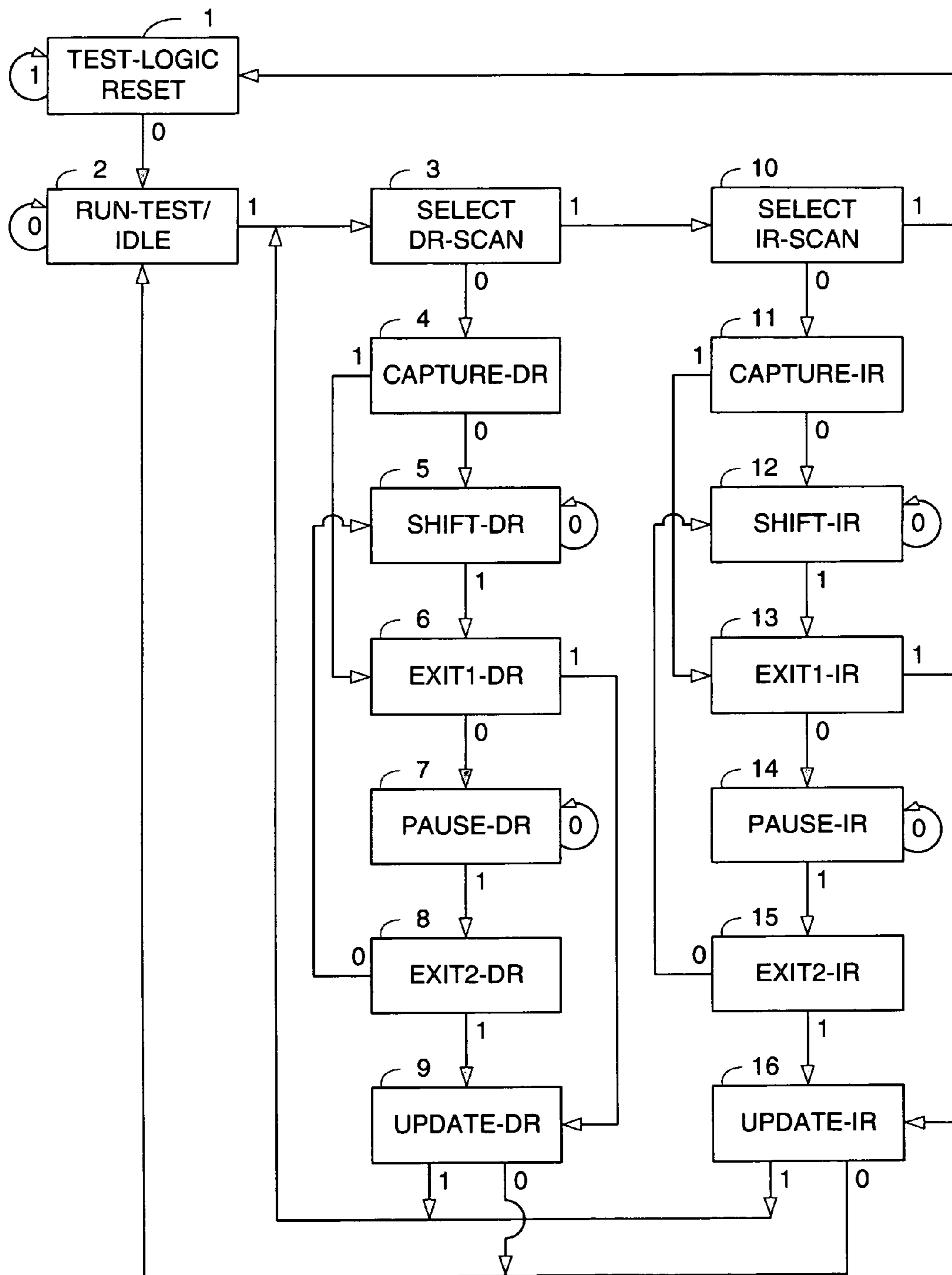
FIG. 2 (PRIOR ART)
