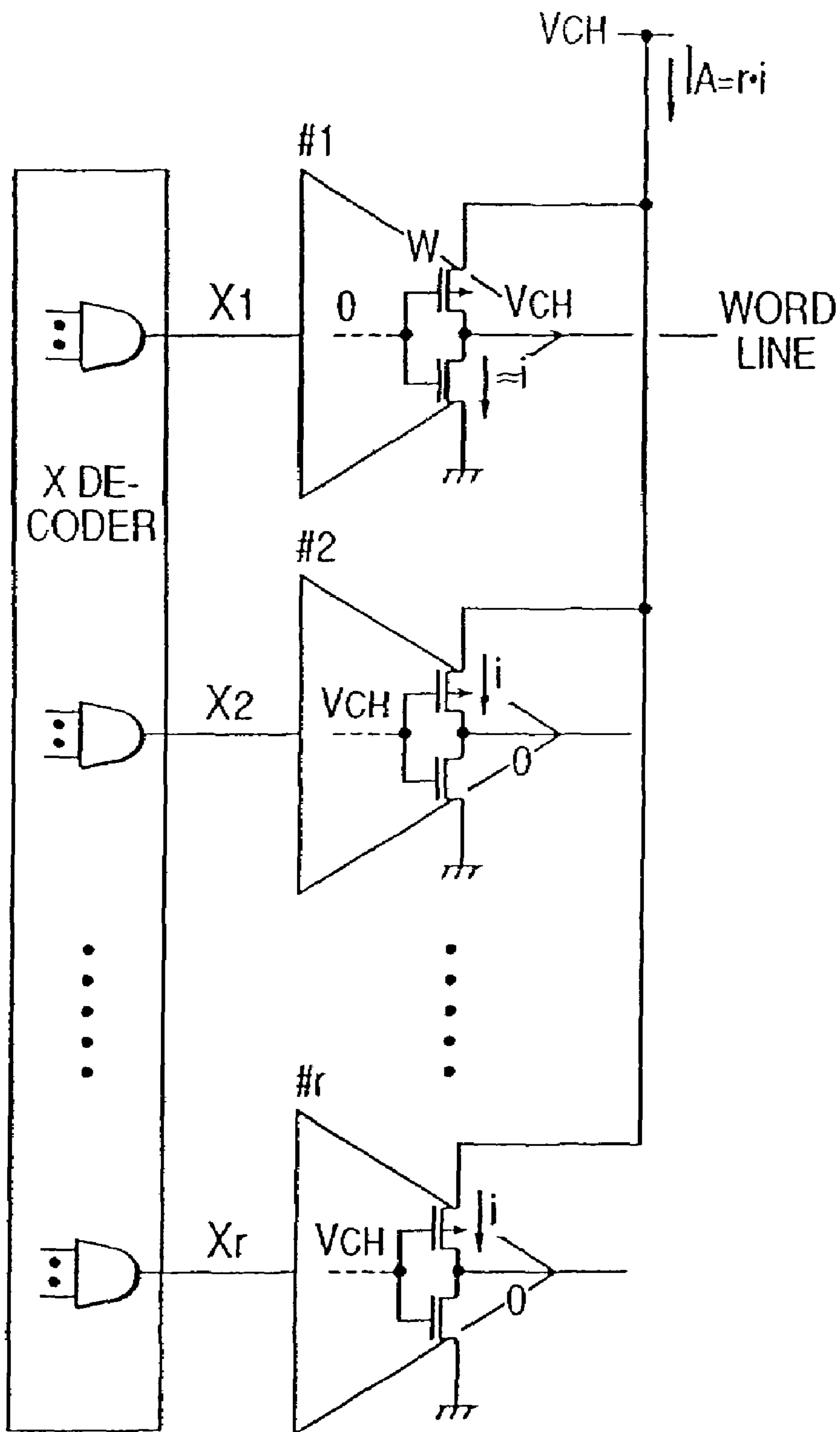
FIG. 24 PRIOR ART
