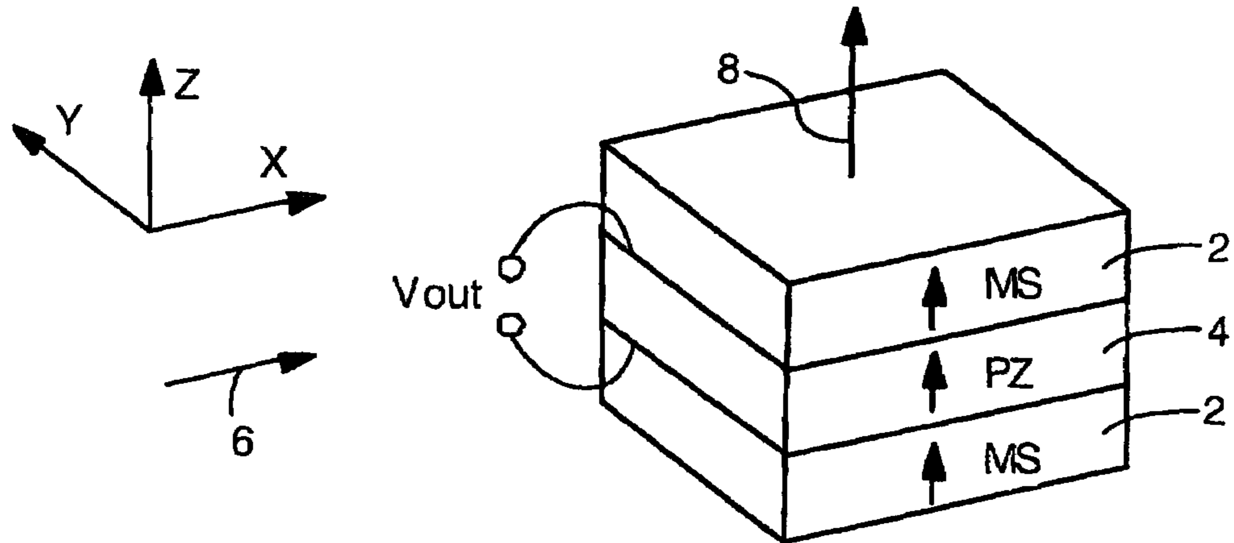
Fig. 1 Prior Art
