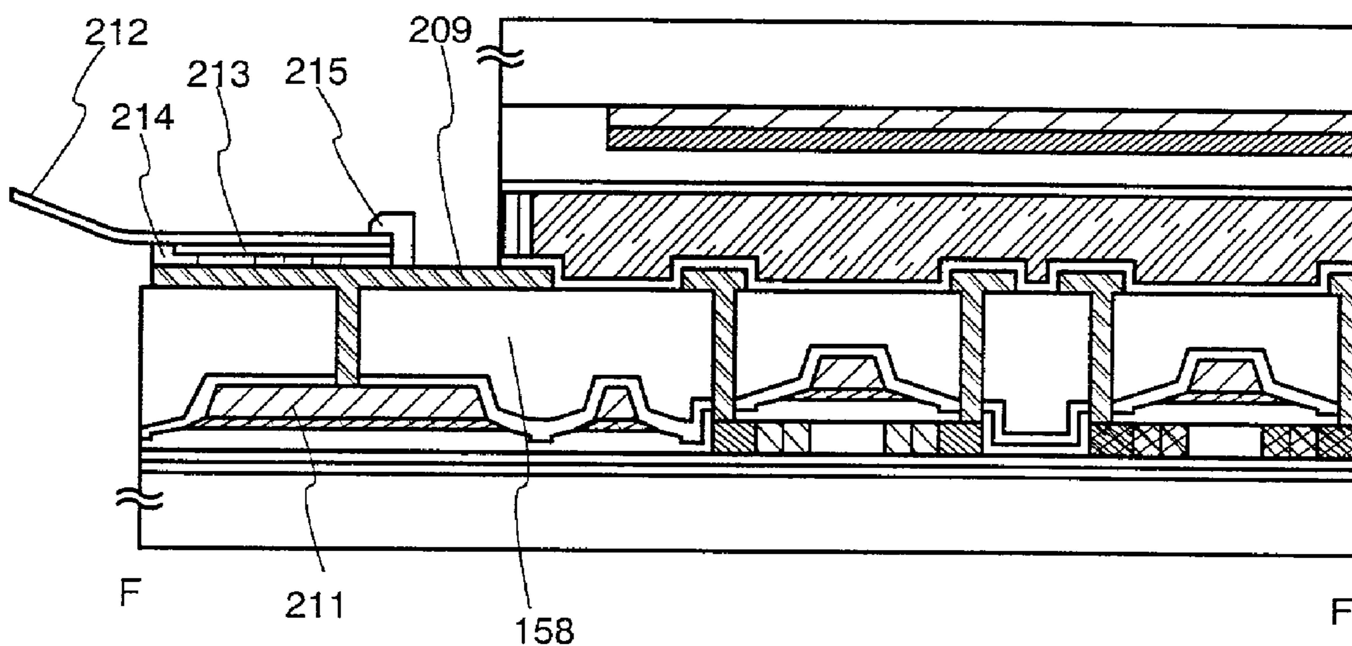
FIG. 8A cross sectional view of F-F'
