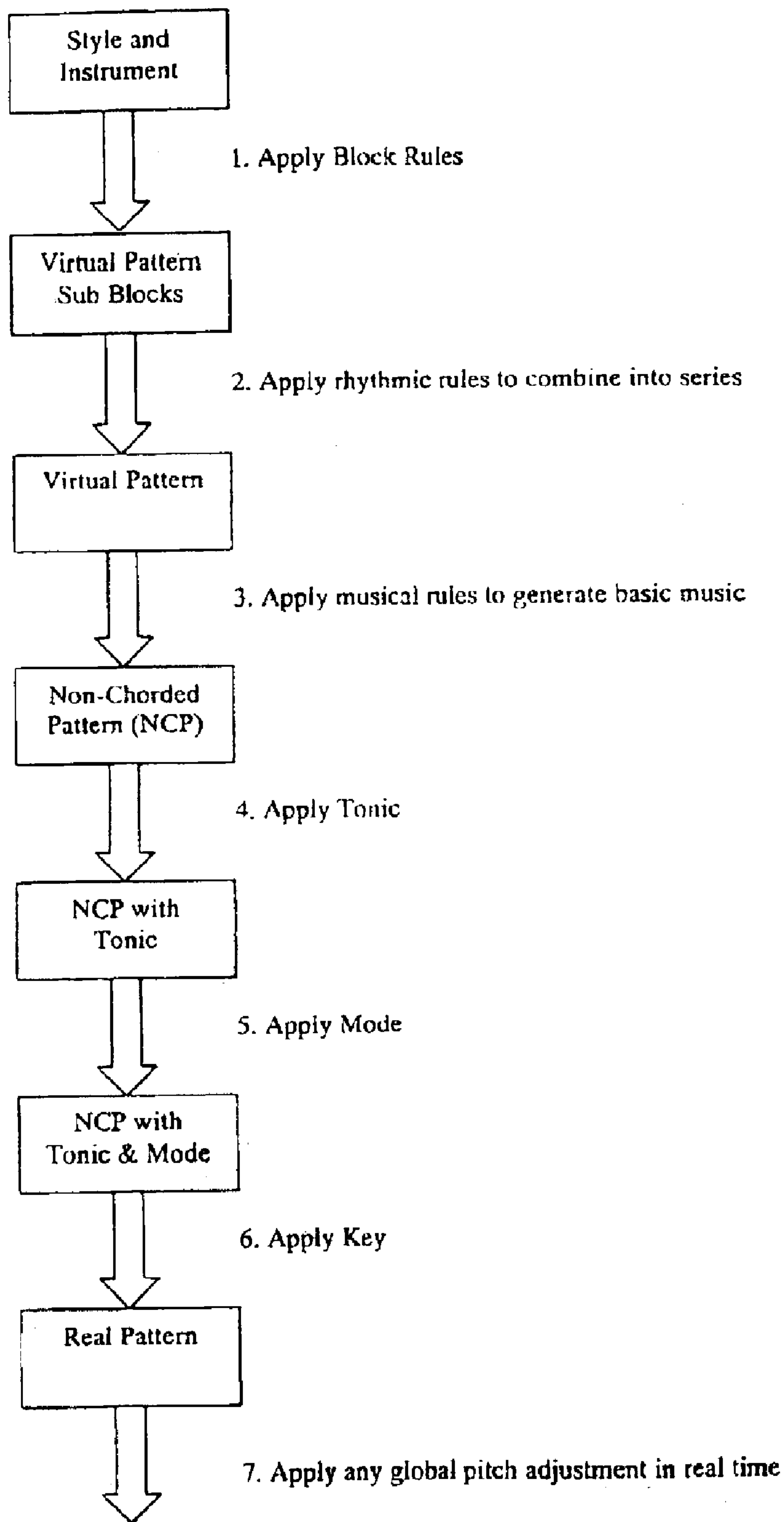
Figure 16 General Musical Generation Flow
