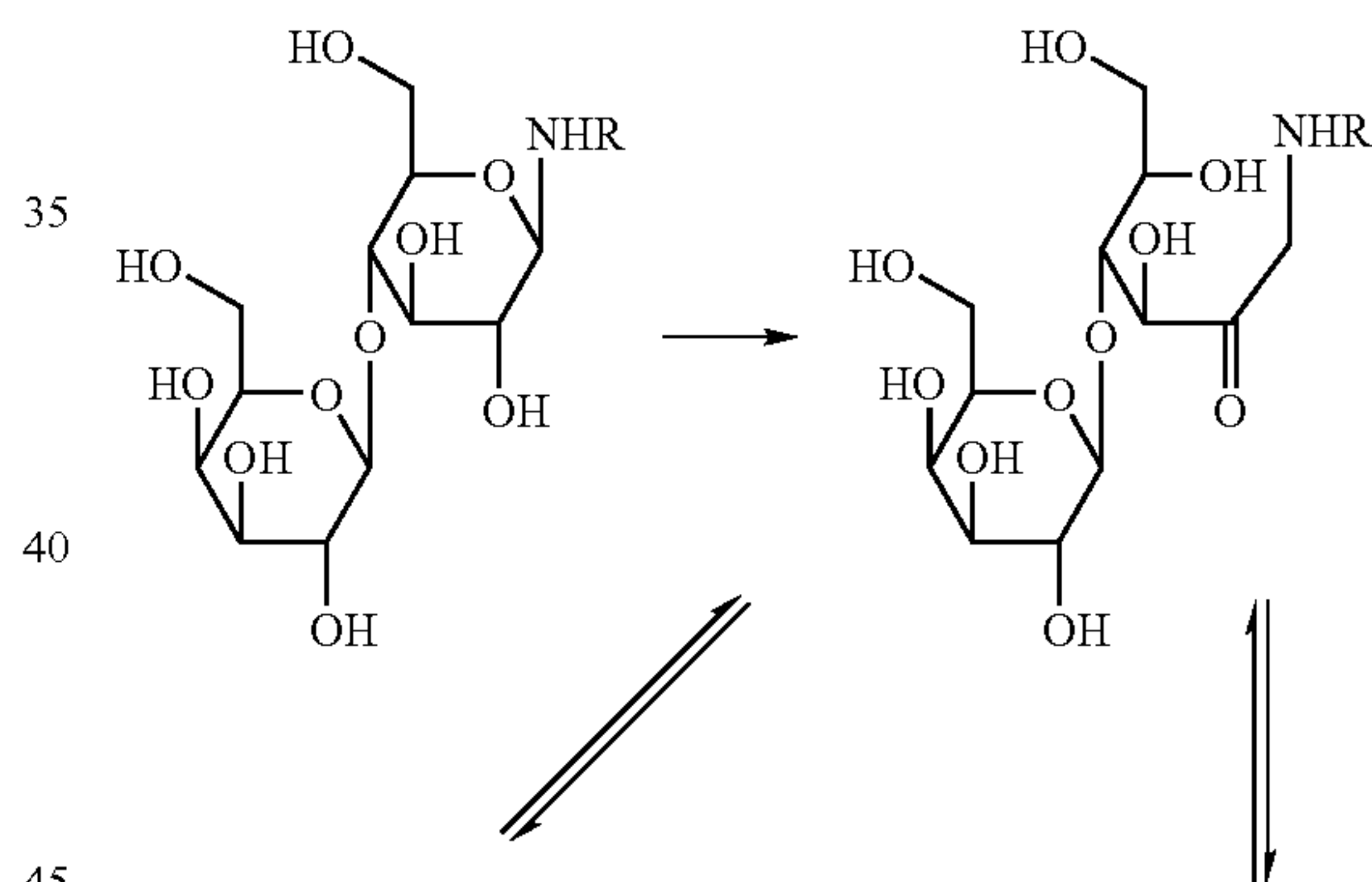
Scheme 2 Amadori Arrangement
