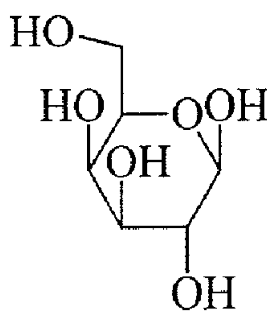
b-Galactose
