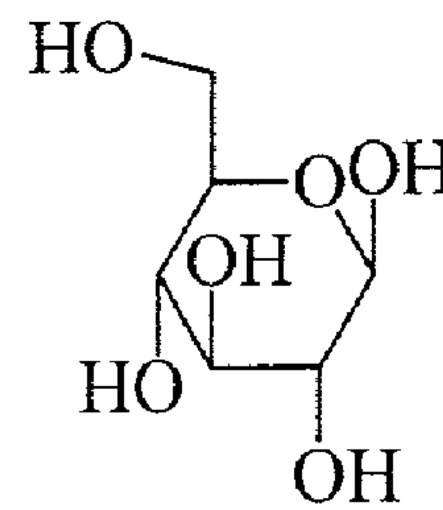
b-Glucose
