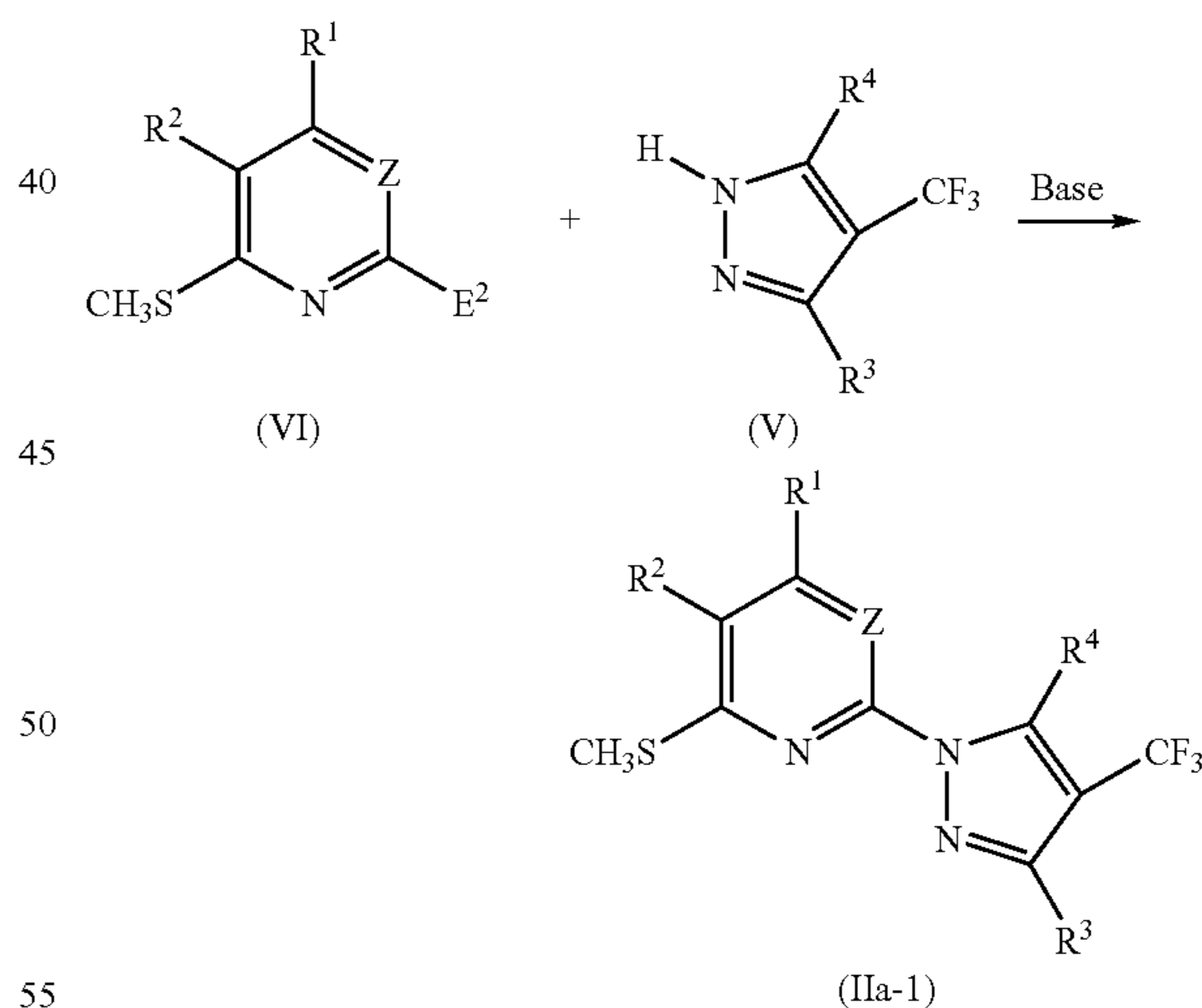
Scheme 4:
