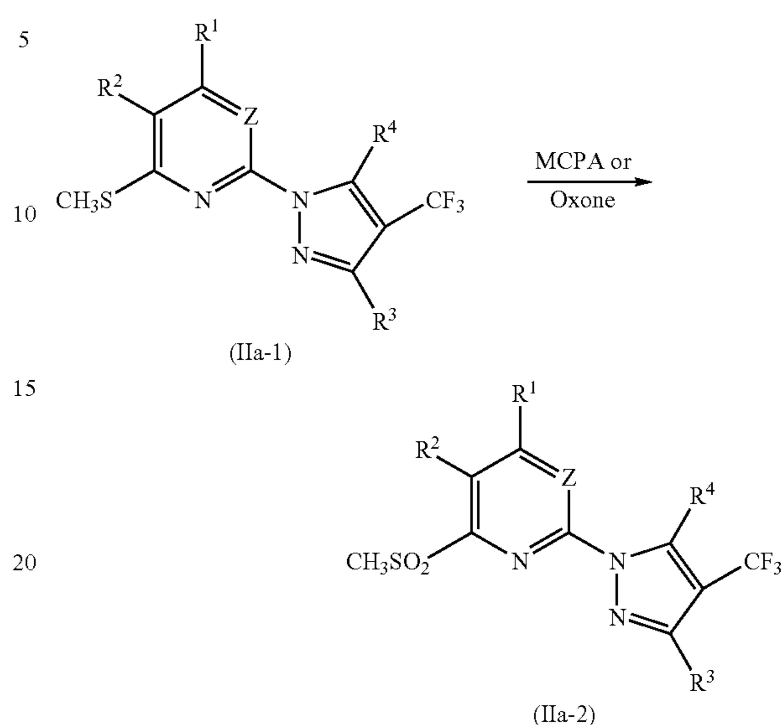
Scheme 3:
