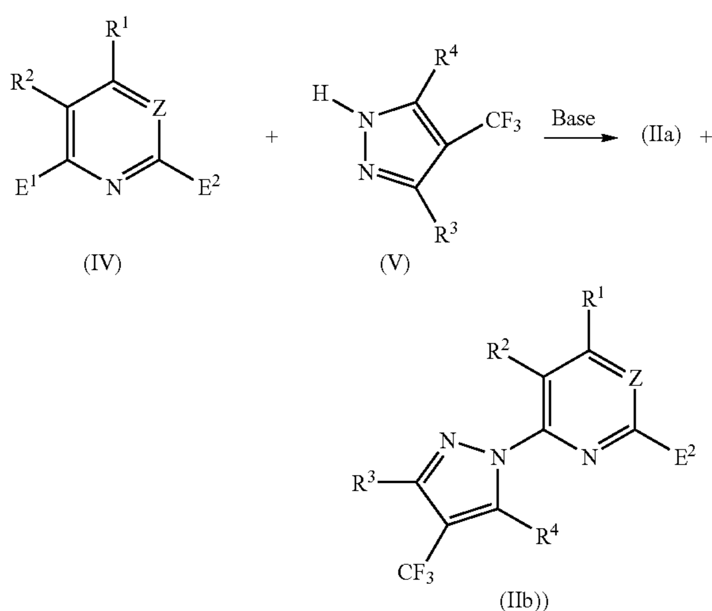
Scheme 2:
