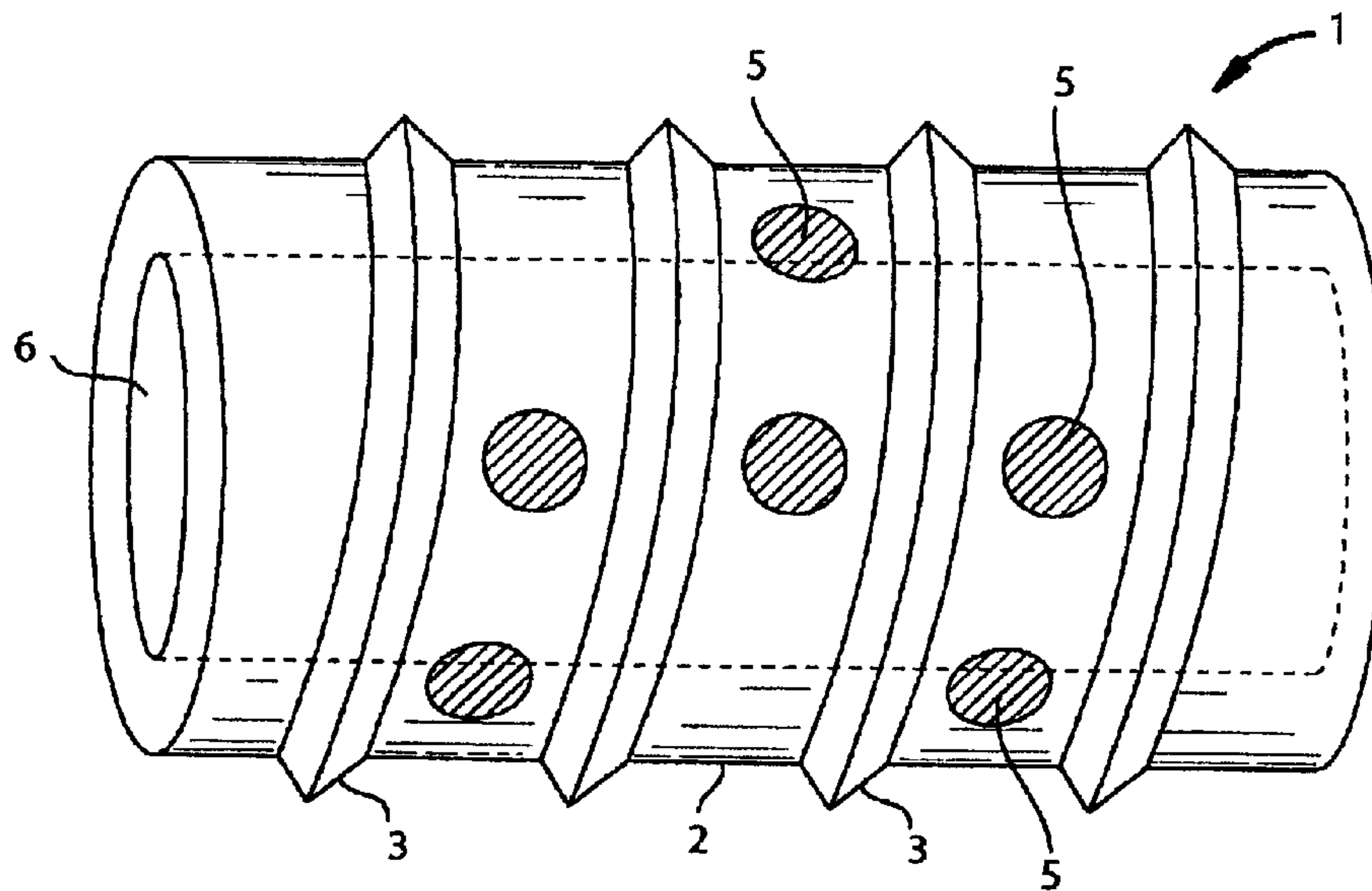
FIG. 13 (PRIOR ART)
