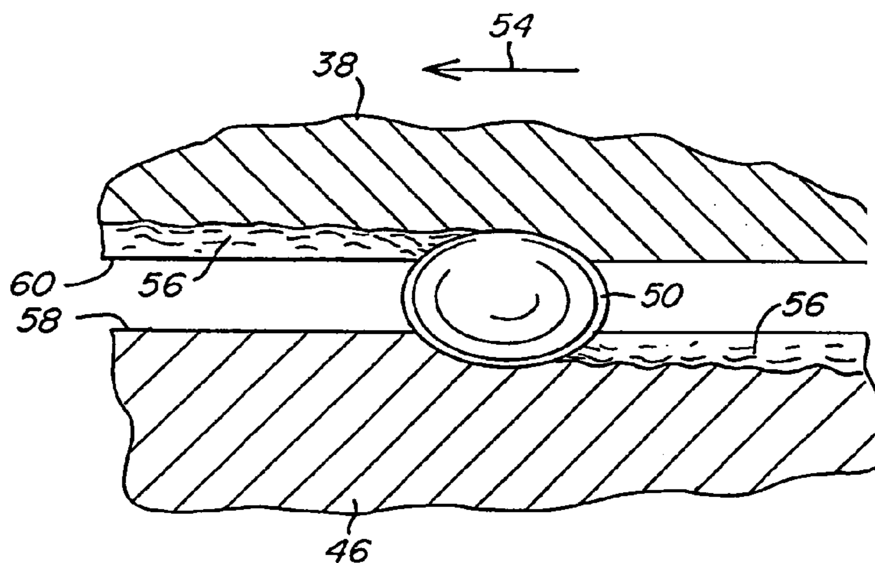
Fig. 5 (PRIOR ART)
