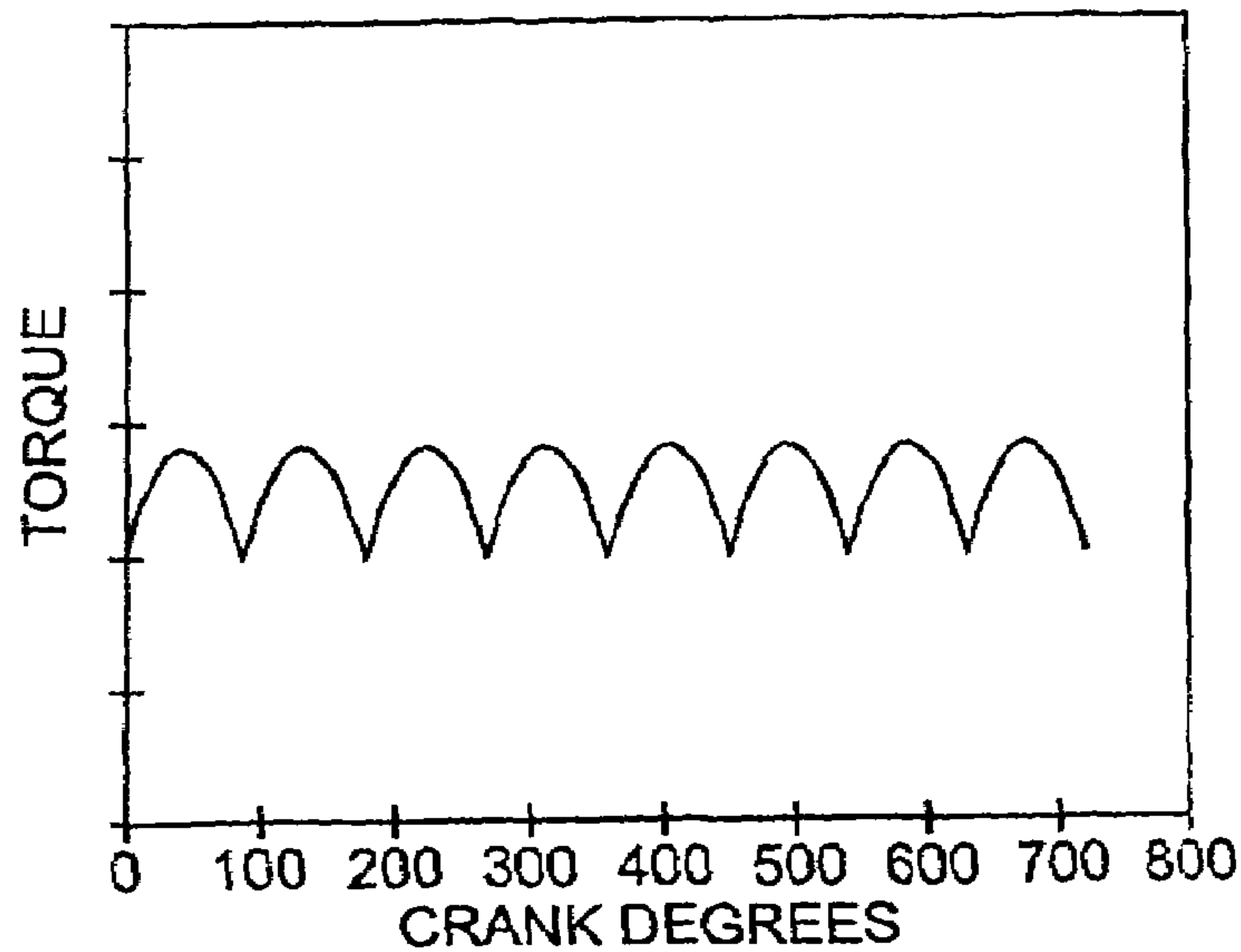
TORQUE PULSATIONS FOR ALL 8 CYLINDERS FIRING
