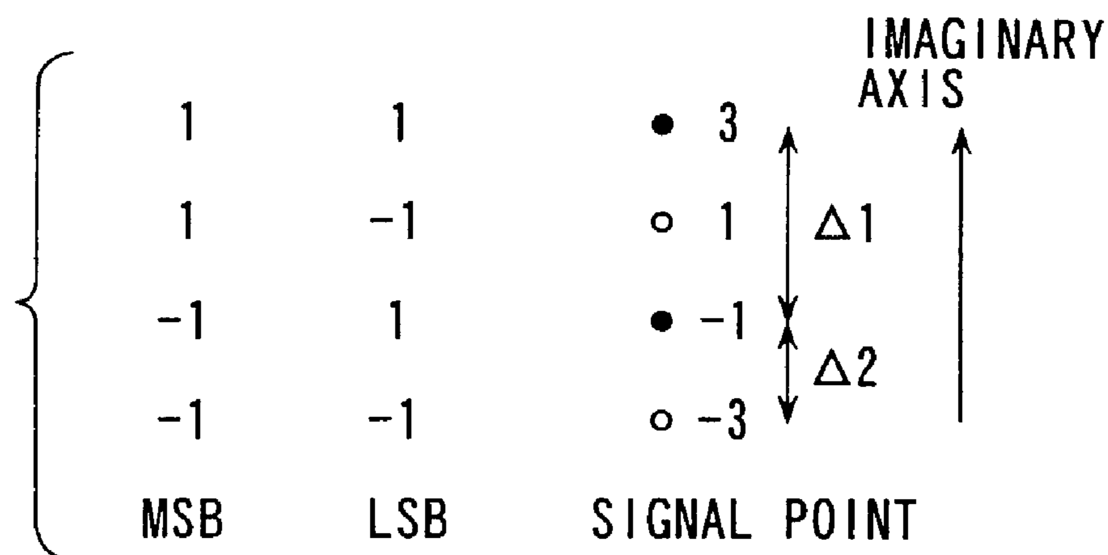
IMAGINARY AXIS COMPONENT OF SIGNAL POINT
