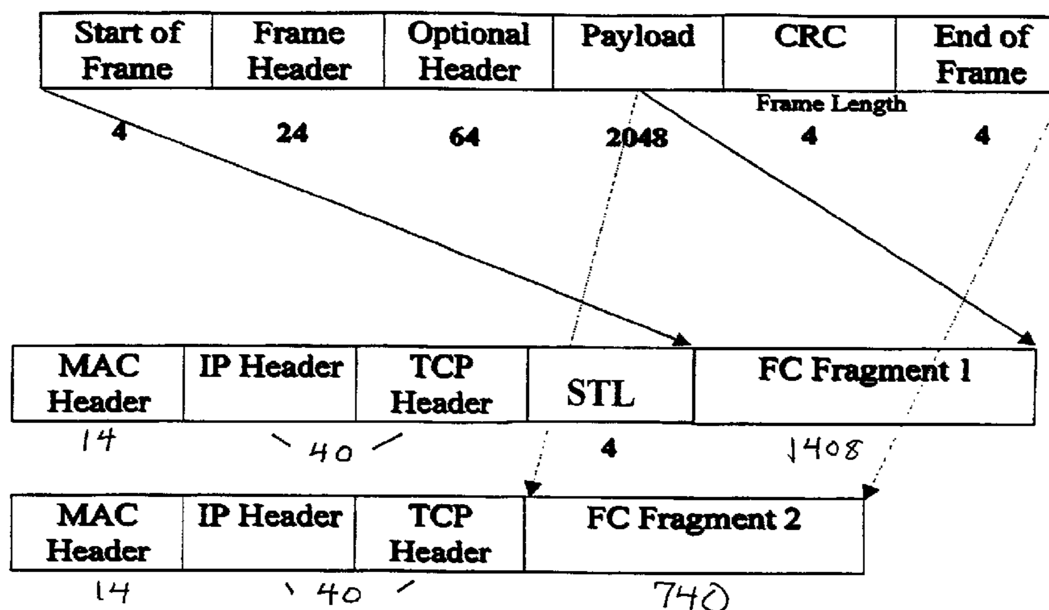
FC Frame segmented into two Ethernet Frames
