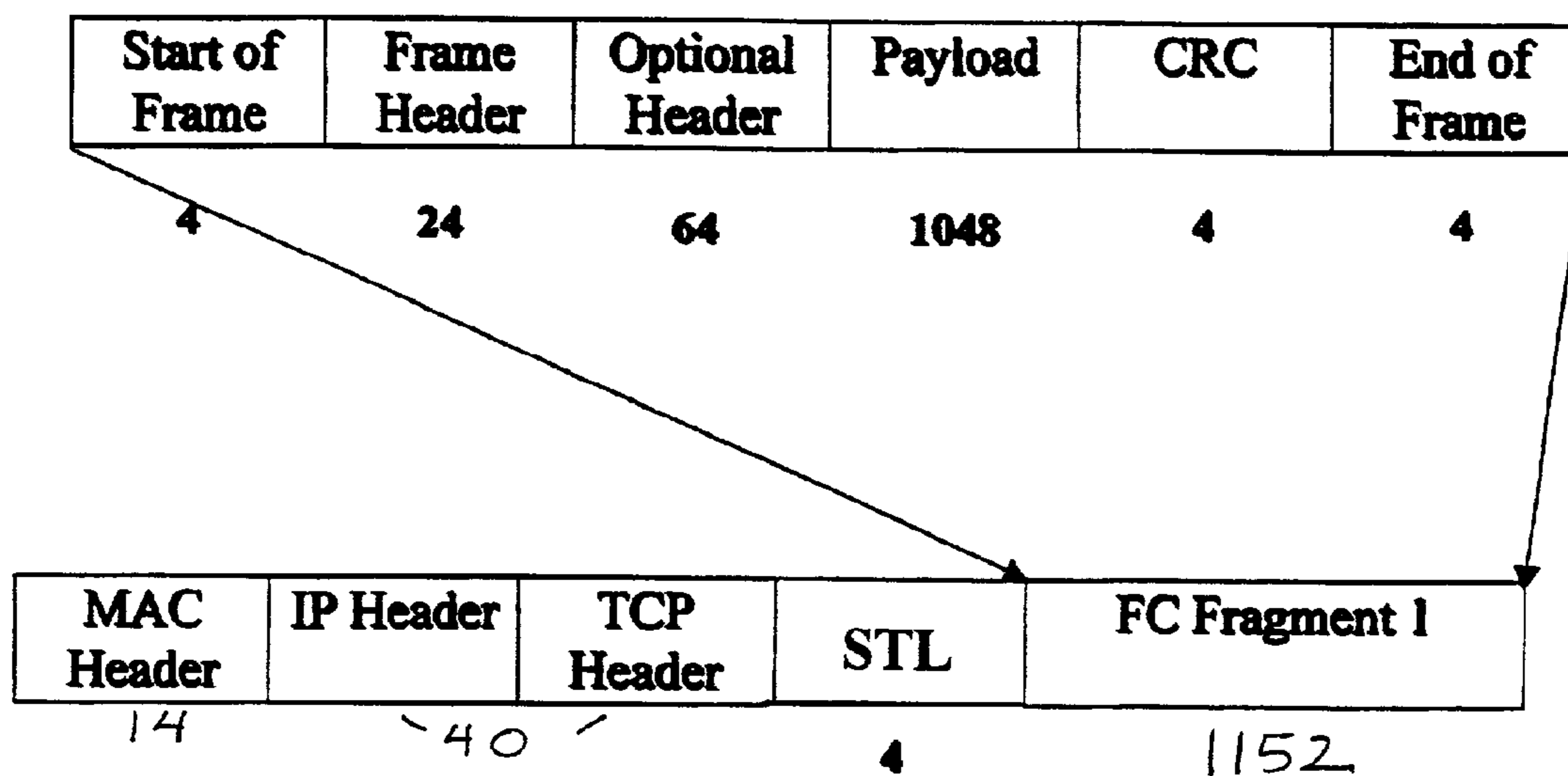
FC Frame segmented into one Ethernet Frame
