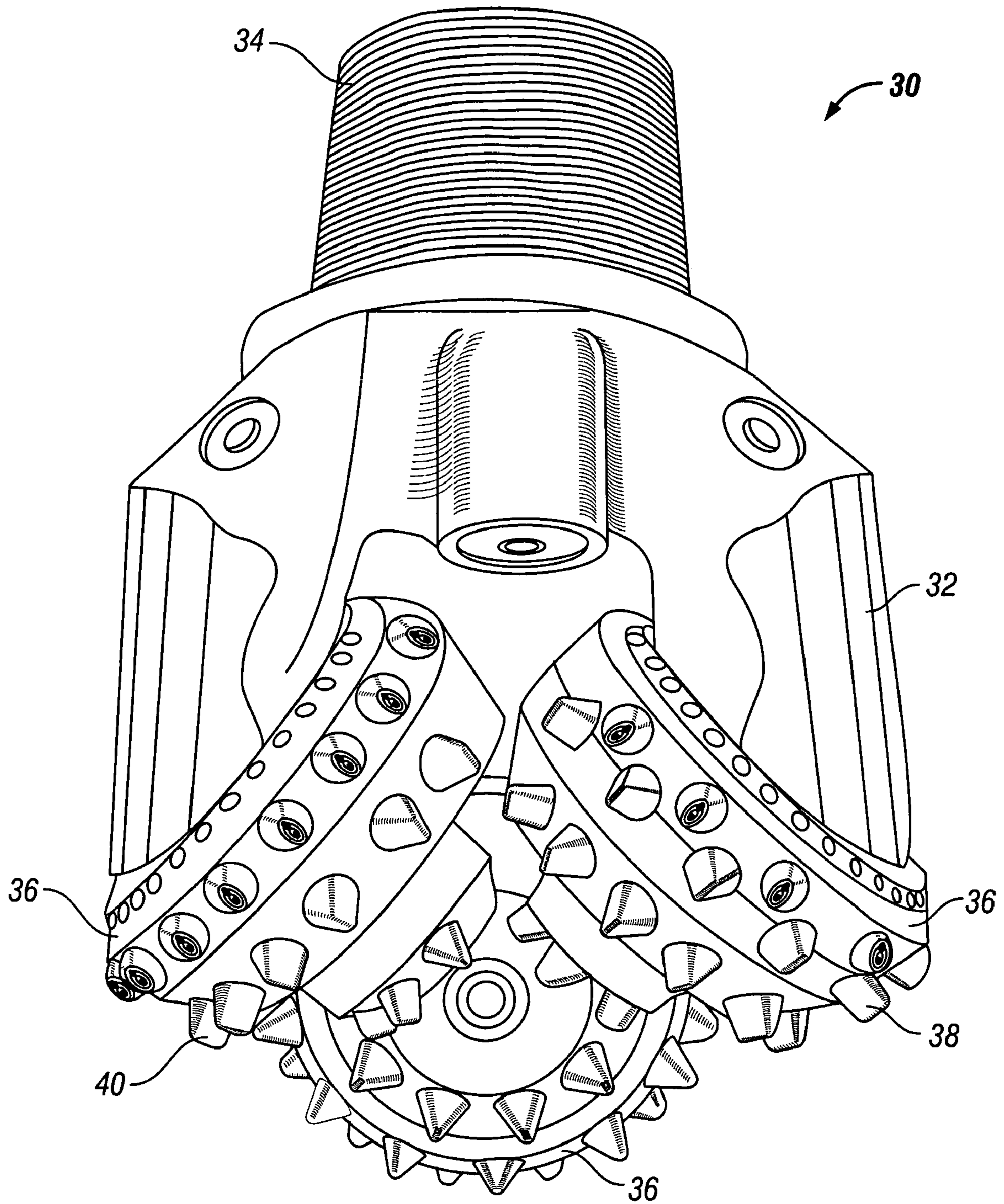
FIG. 3 (Prior Art)
